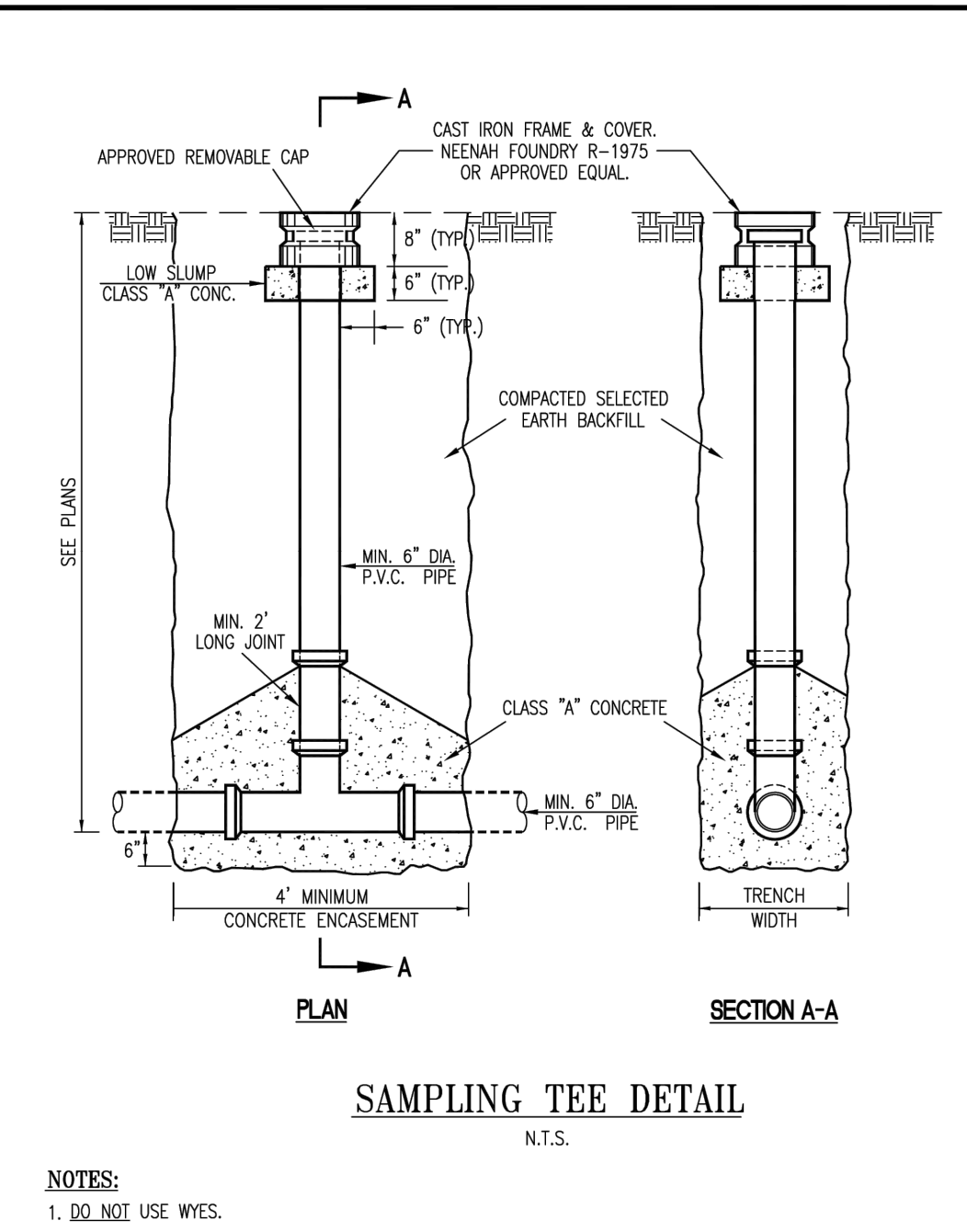
Duckett Creek Sanitary District SAMPLING TEE H SAMPLING TEE NOT TO SCALE
