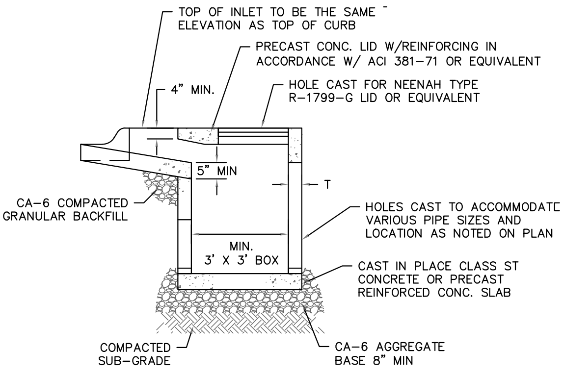
NOTE: 1. PRE-CAST INLET SHALL CONFORM TO ASTM C-478 2. ALL INLET BOXES WITH STORM SEWER PIPES HAVE INNER DIMENSIONS OF 12" PLUS THE DIAMETER OF THE PIPE C OPEN THROAT INLET DETAIL NOT TO SCALE
