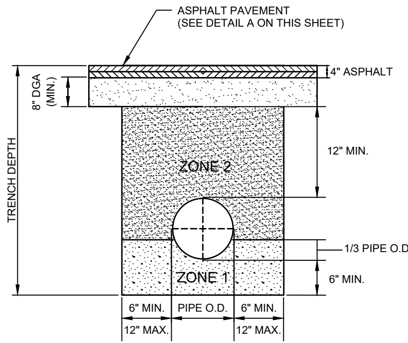
A PIPE TRENCH DETAIL NOT TO SCALE
