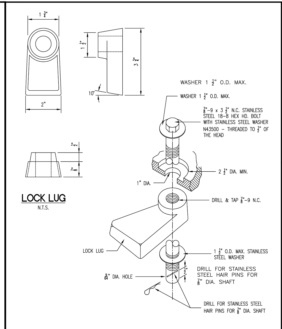
Duckett Creek Sanitary District LOCKING DEVICE FOR TYPE "N" LOCK TYPED MANHOLE COVER I LOCKING DEVICE FOR TYPE "N" LOCK TYPED MANHOLE COVER NOT TO SCALE
