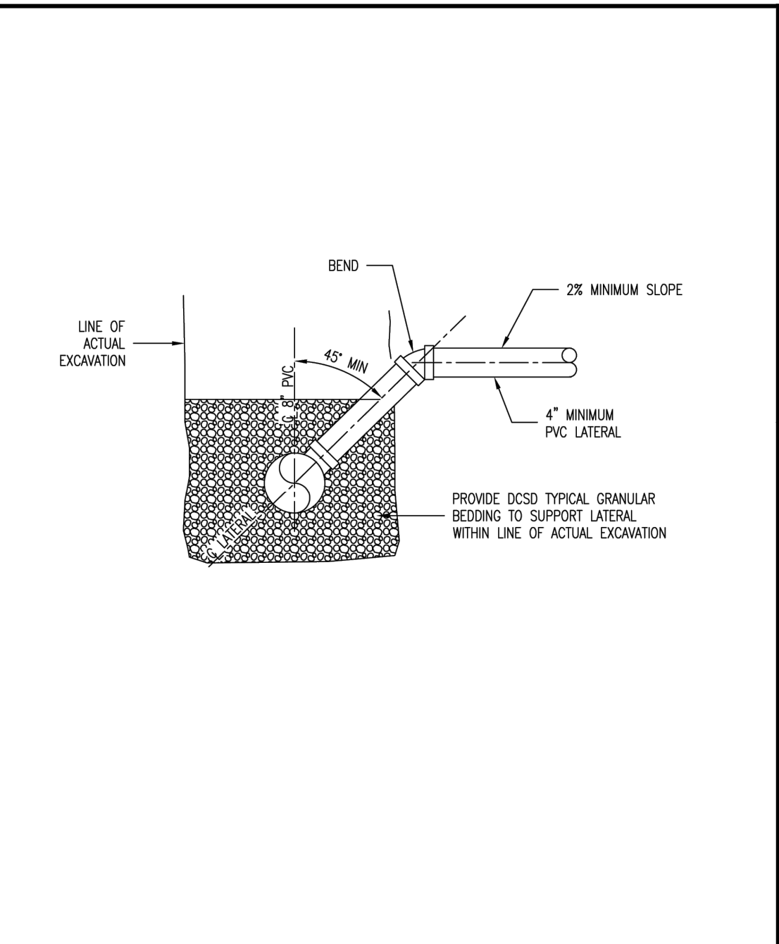
Duckett Creek Sanitary District SANITARY SEWER LATERAL RISER DETAIL G SANITARY SEWER LATERAL RISER DETAIL NOT TO SCALE
