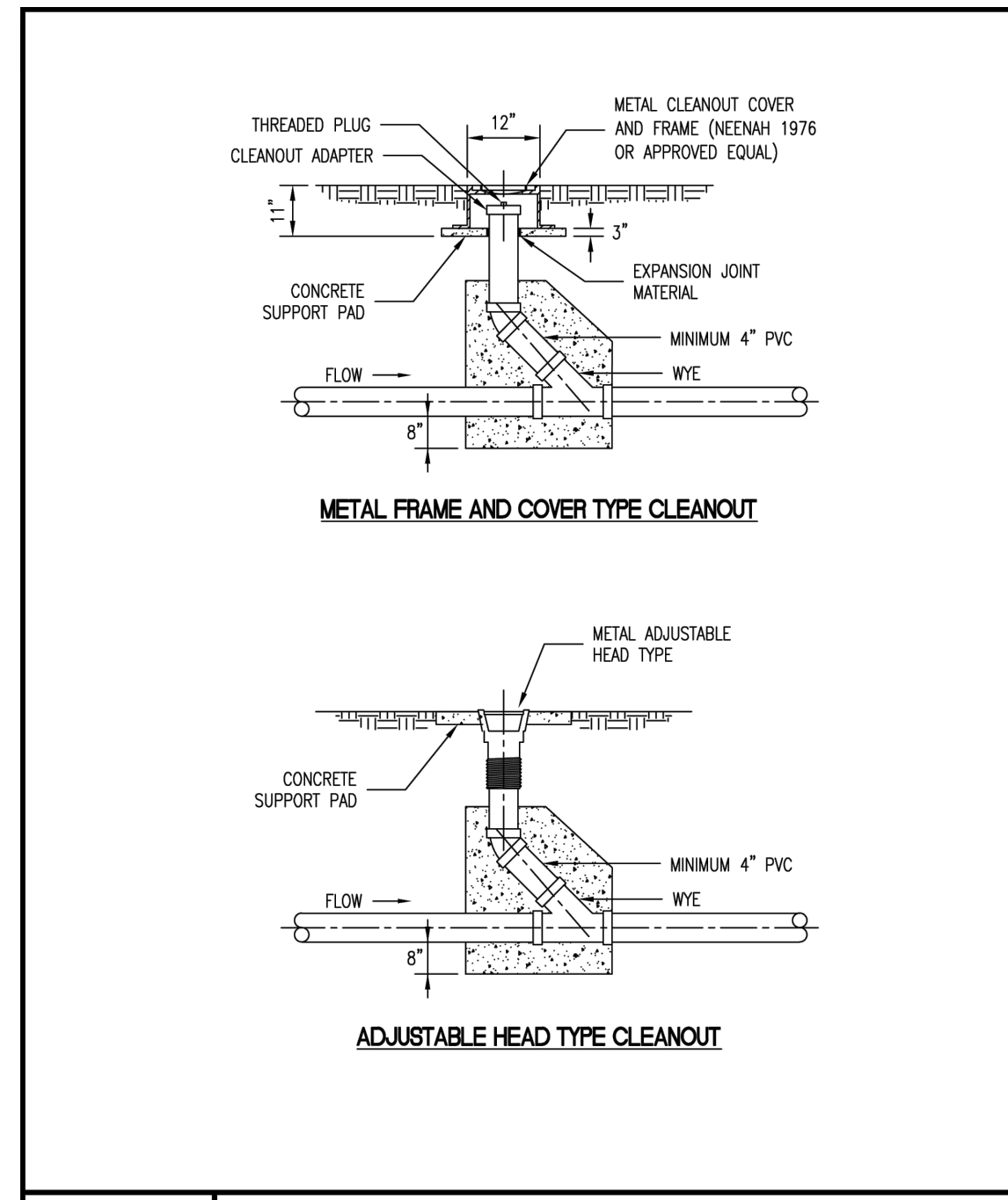
Duckett Creek Sanitary District TYPICAL SANITARY SEWER CLEANOUT DETAIL B SANITARY SEWER CLEANOUT DETAIL NOT TO SCALE
