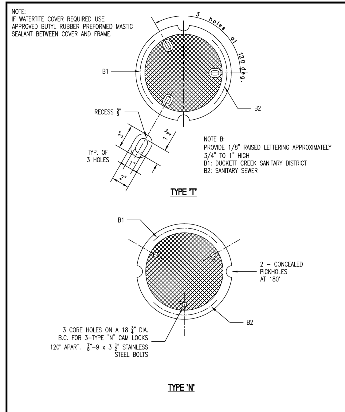
Duckett Creek Sanitary District CAST IRON MANHOLE COVERS (LOCK TYPE) E CAST IRON MANHOLE COVERS (LOCK TYPE) NOT TO SCALE
