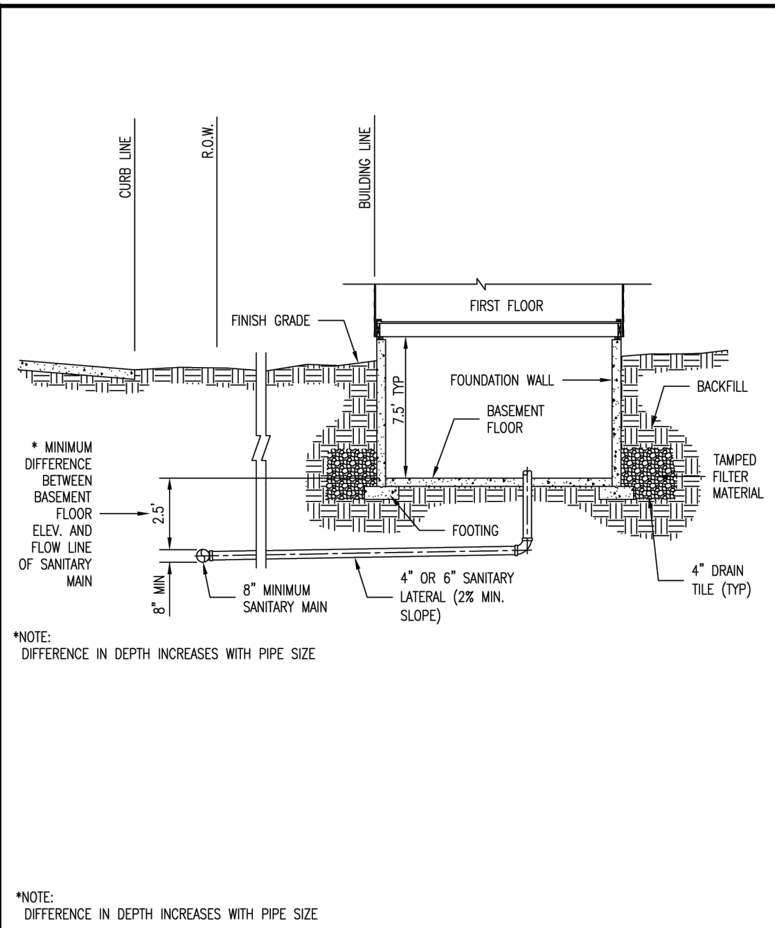
Duckett Creek Sanitary District TYPICAL SANITARY SEWER LATERAL PROFILE F TYPICAL SANITARY SEWER LATERAL PROFILE NOT TO SCALE
