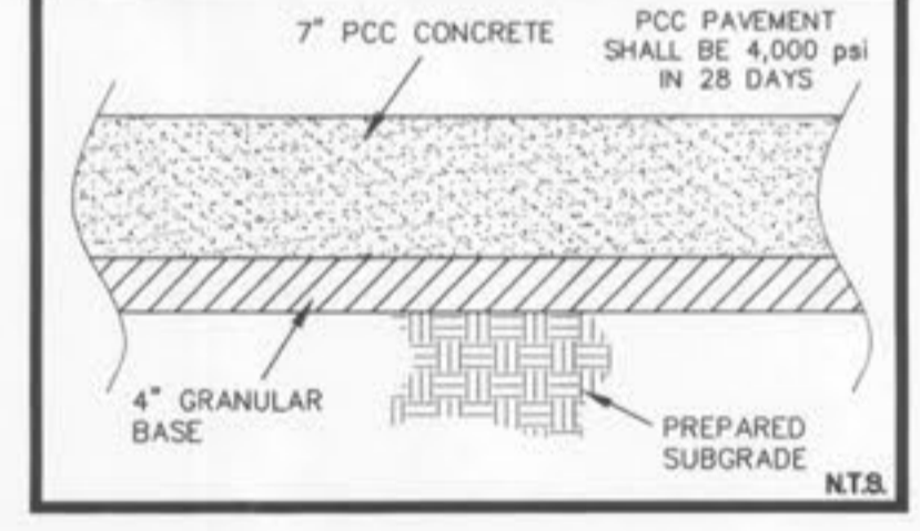
ENTRANCE PAVEMENT WITH IN RIGHT OF WAY
