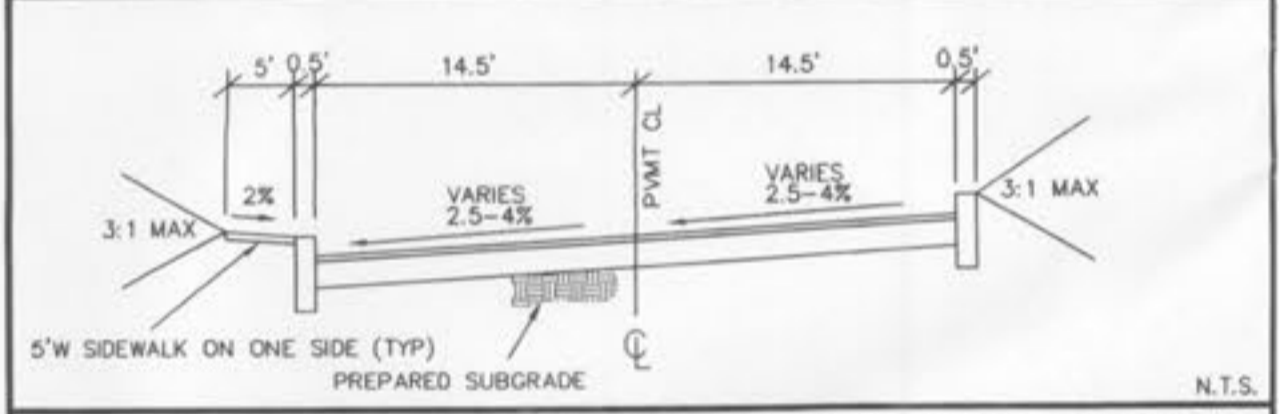
ACCESS ROAD CROSS SECTION (STA 1+65 - 4+09)
