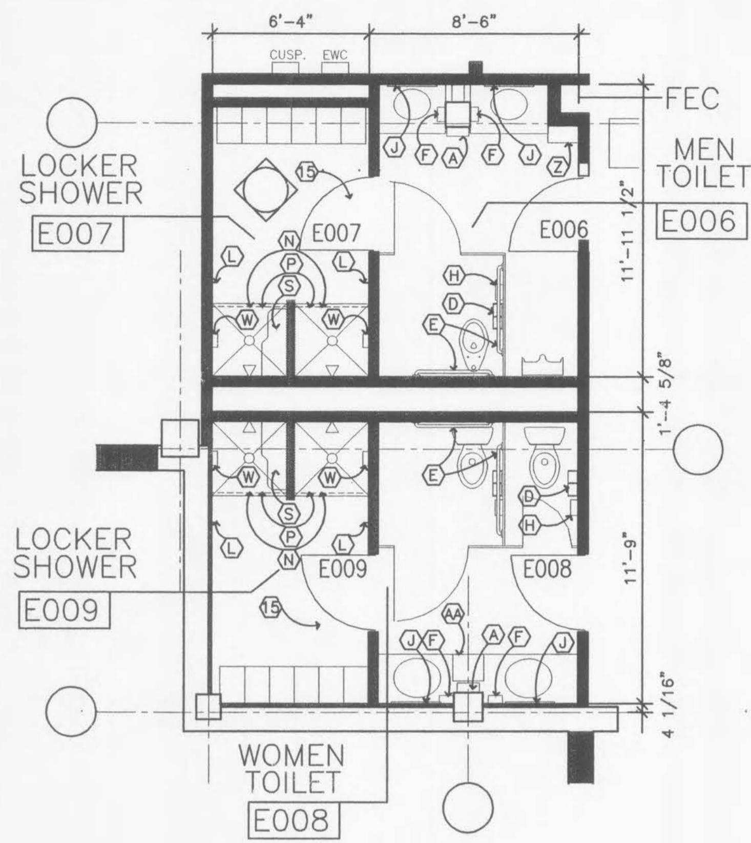
1 BASEMENT FLOOR TOILET PLAN SCALE: 1/4" = 1'-0"
