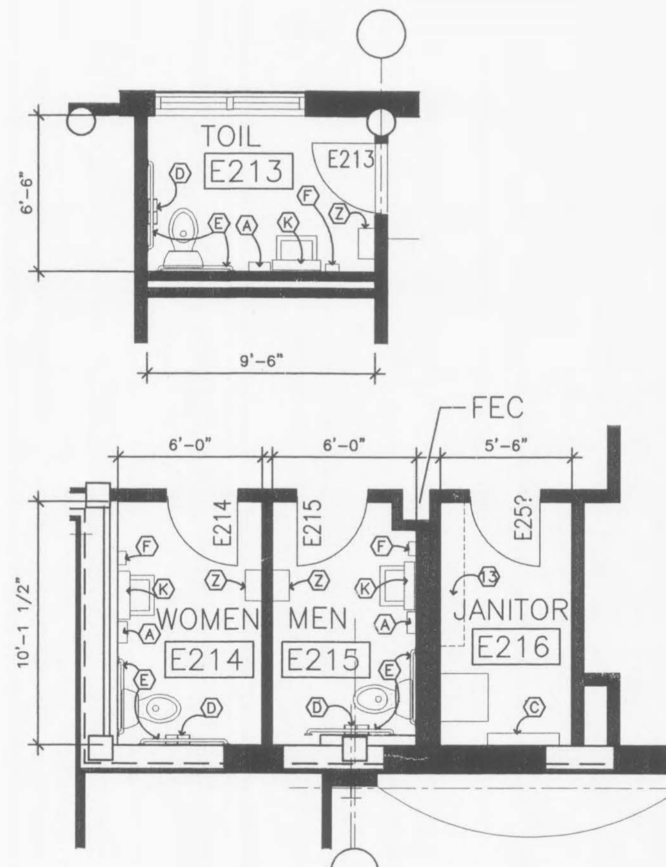
6 SECOND FLOOR TOILET PLAN SCALE: 1/4" = 1'-0"
