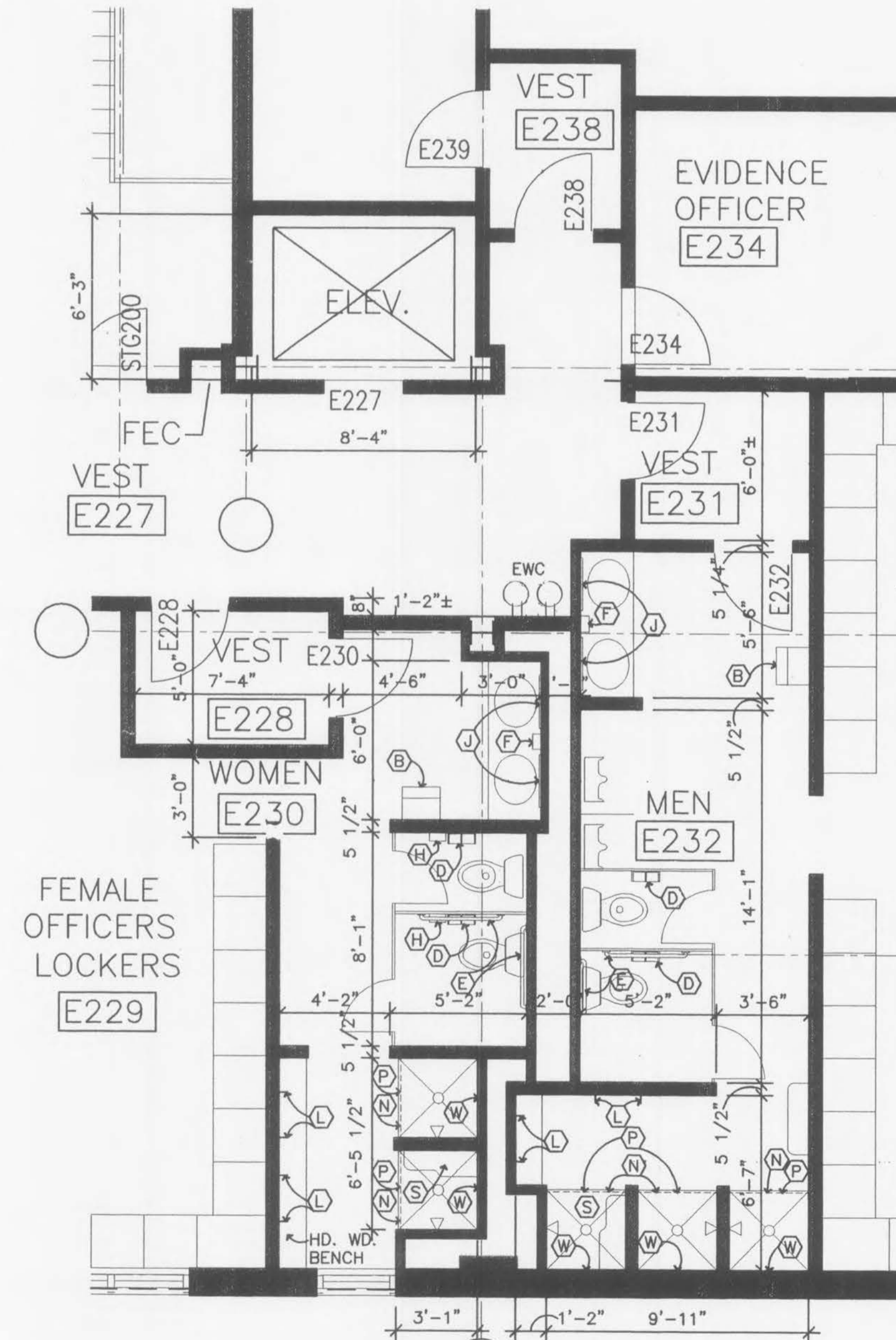
7 SECOND FLOOR TOILET PLAN SCALE: 1/4" = 1'-0"
