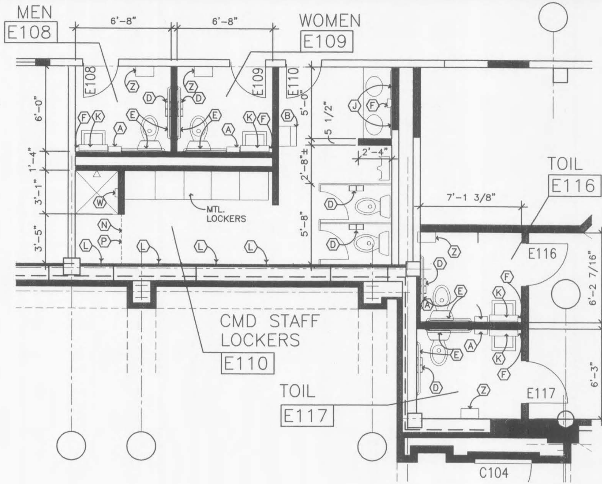
2 FIRST FLOOR TOILET PLAN SCALE: 1/4" = 1'-0"
