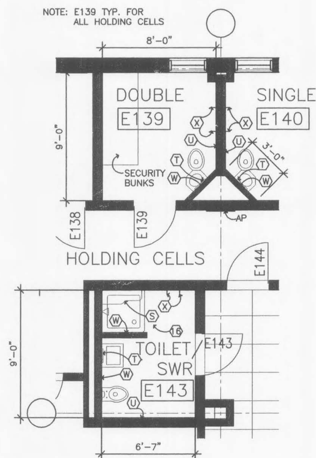
5 FIRST FLOOR TOILET PLAN SCALE: 1/4" = 1'-0"
