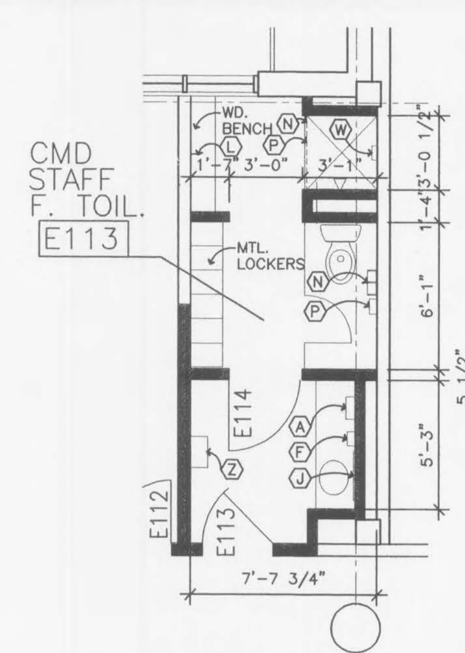
3 FIRST FLOOR TOILET PLAN SCALE: 1/4" = 1'-0"
