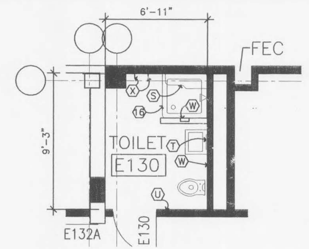
4 FIRST FLOOR TOILET PLAN SCALE: 1/4" = 1'-0"
