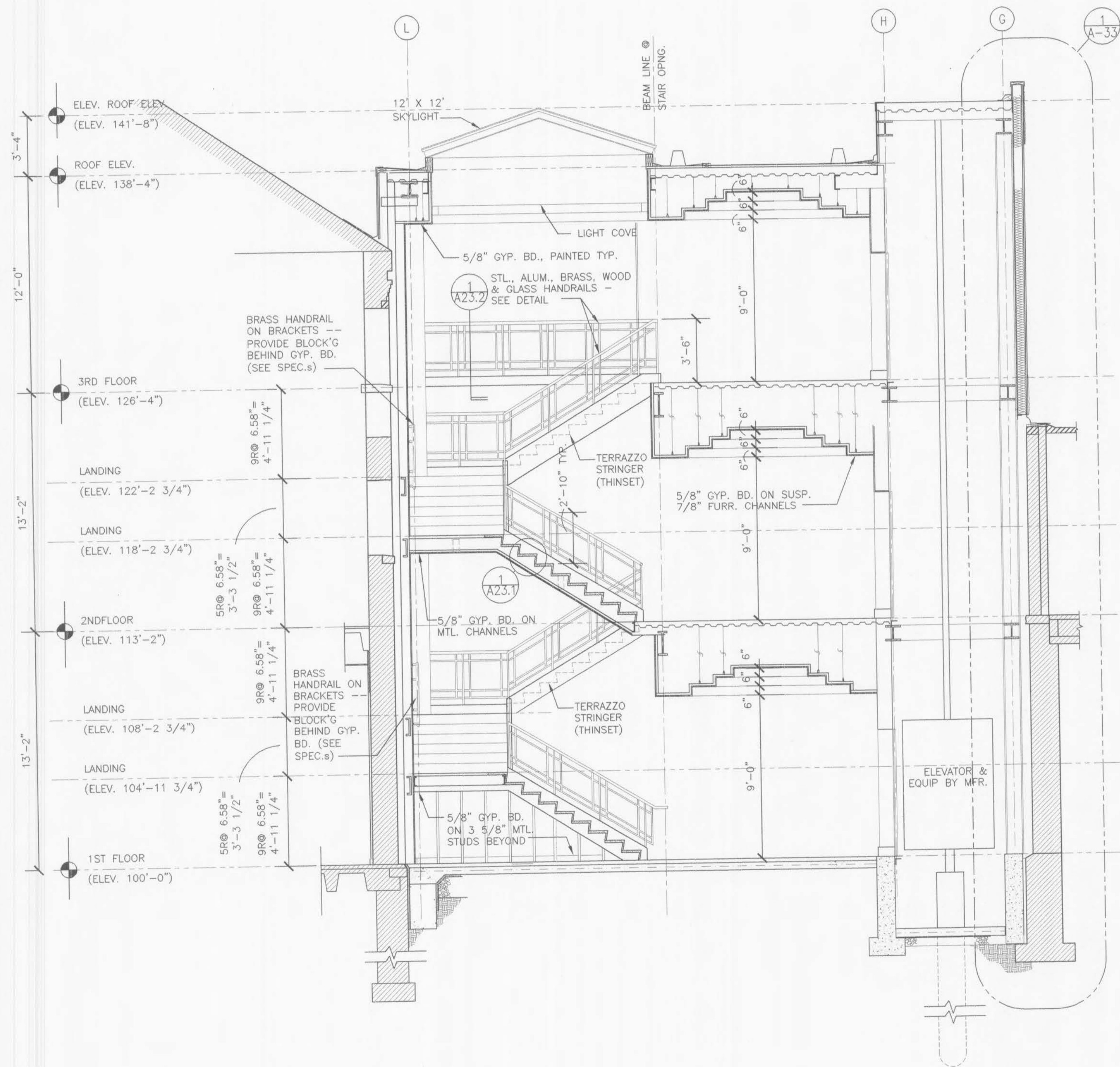
4 SECTION • STAIRS A SCALE 1/4" = 1'-0"
