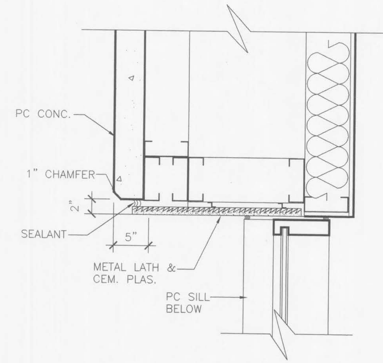
3 A-39.1 JAMB CONDITION & BASE SCALE: 1 1/2" = 1'-0"
