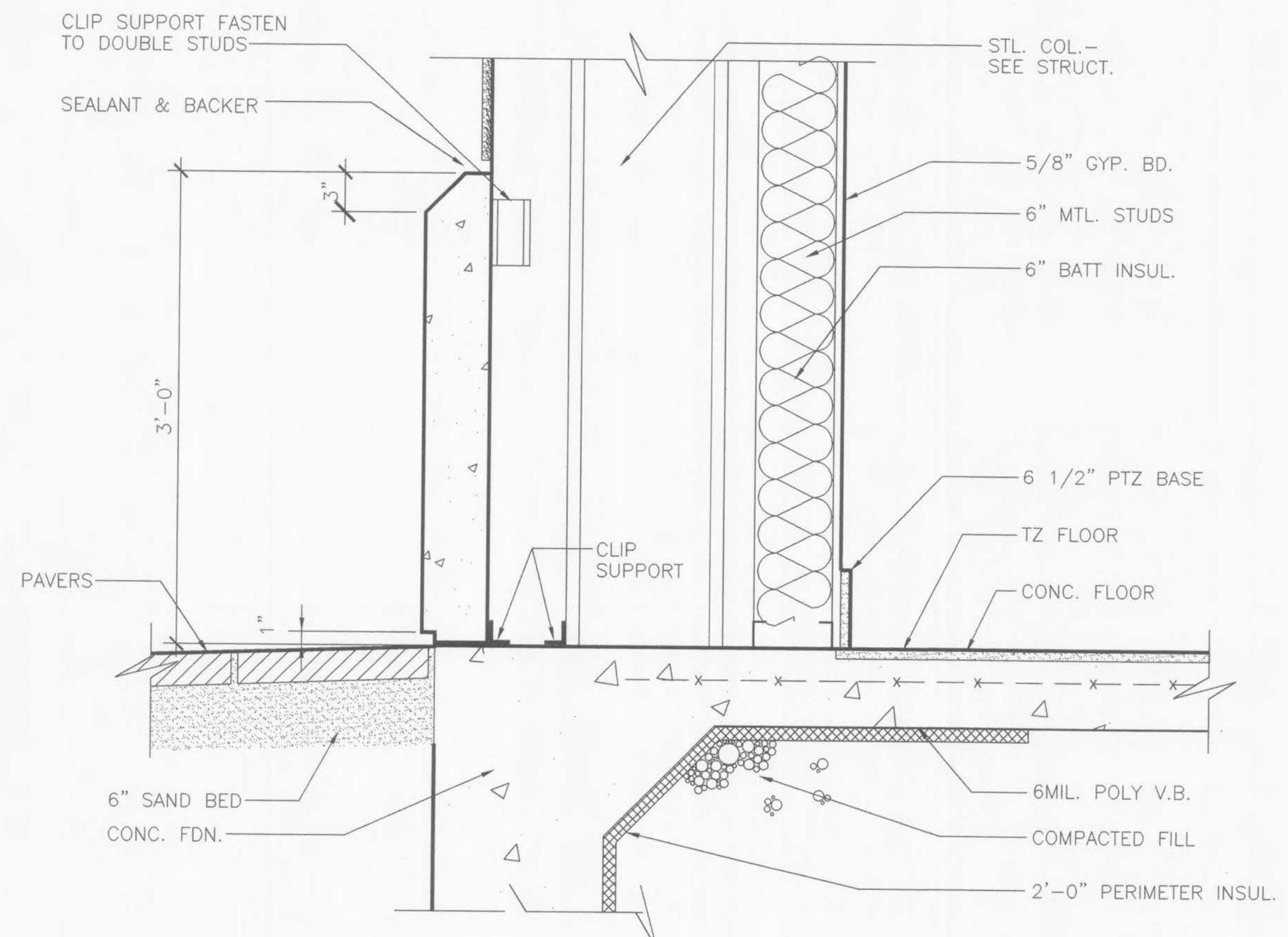
1 A-39.1 BASE CONDITION DETAIL SCALE: 1 1/2" = 1'-0"
