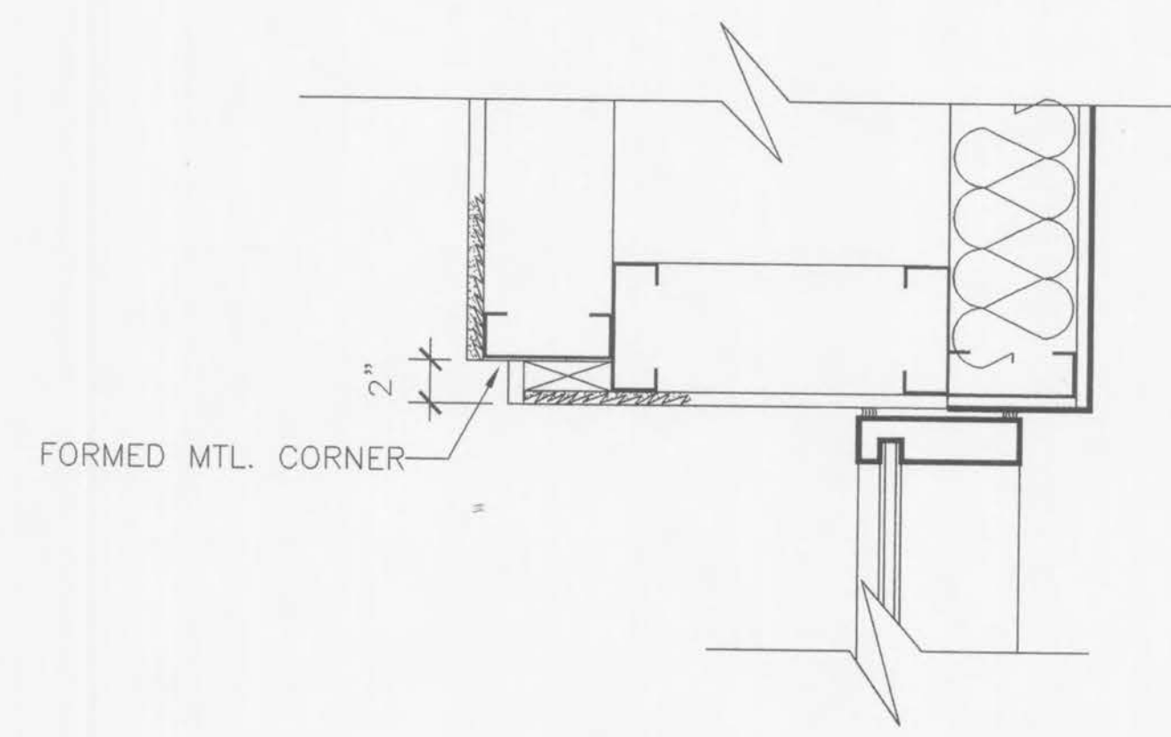
4 A-39.1 PLASTER ALTERNATE JAMB SCALE: 1 1/2" = 1'-0"
