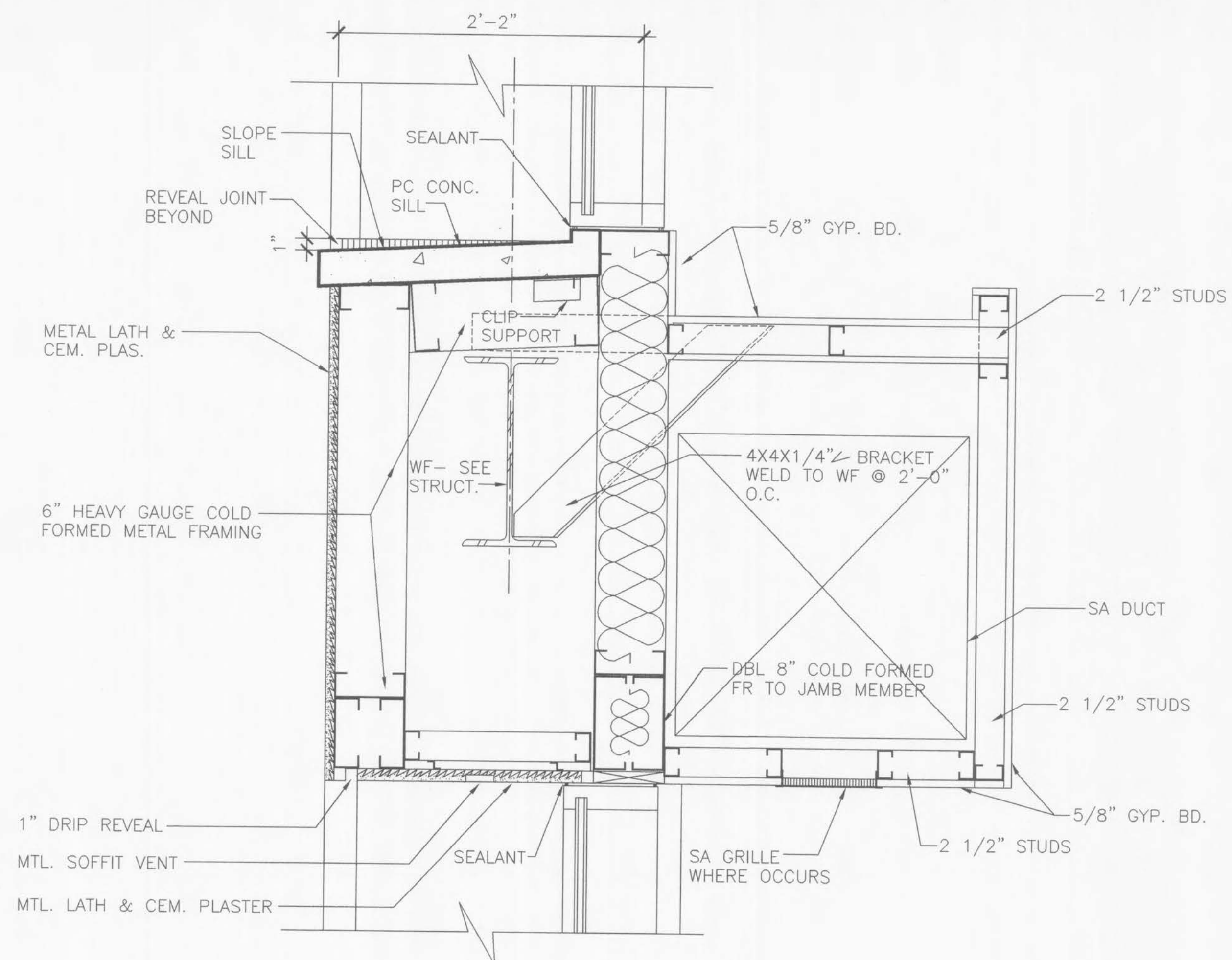
2 A-39.1 PLASTER ALTERNATE SPANDREL PANEL + DUCT SOFFIT DETAIL SCALE: 1 1/2" = 1'-0"
