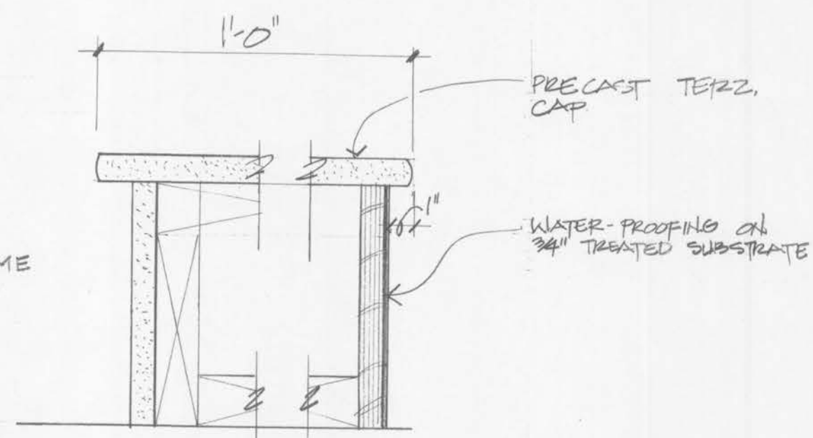
5 PLANTER 3" x 1'-0"
