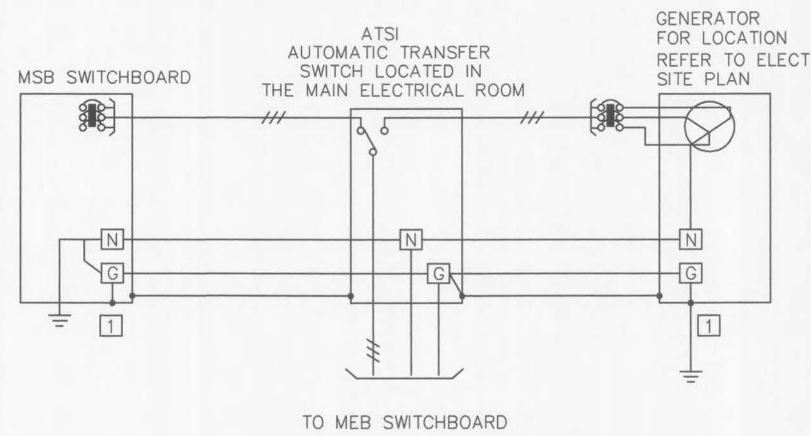
AUTOMATIC TRANSFER SWITCH (ATS) CONNECTION DETAIL NTS
