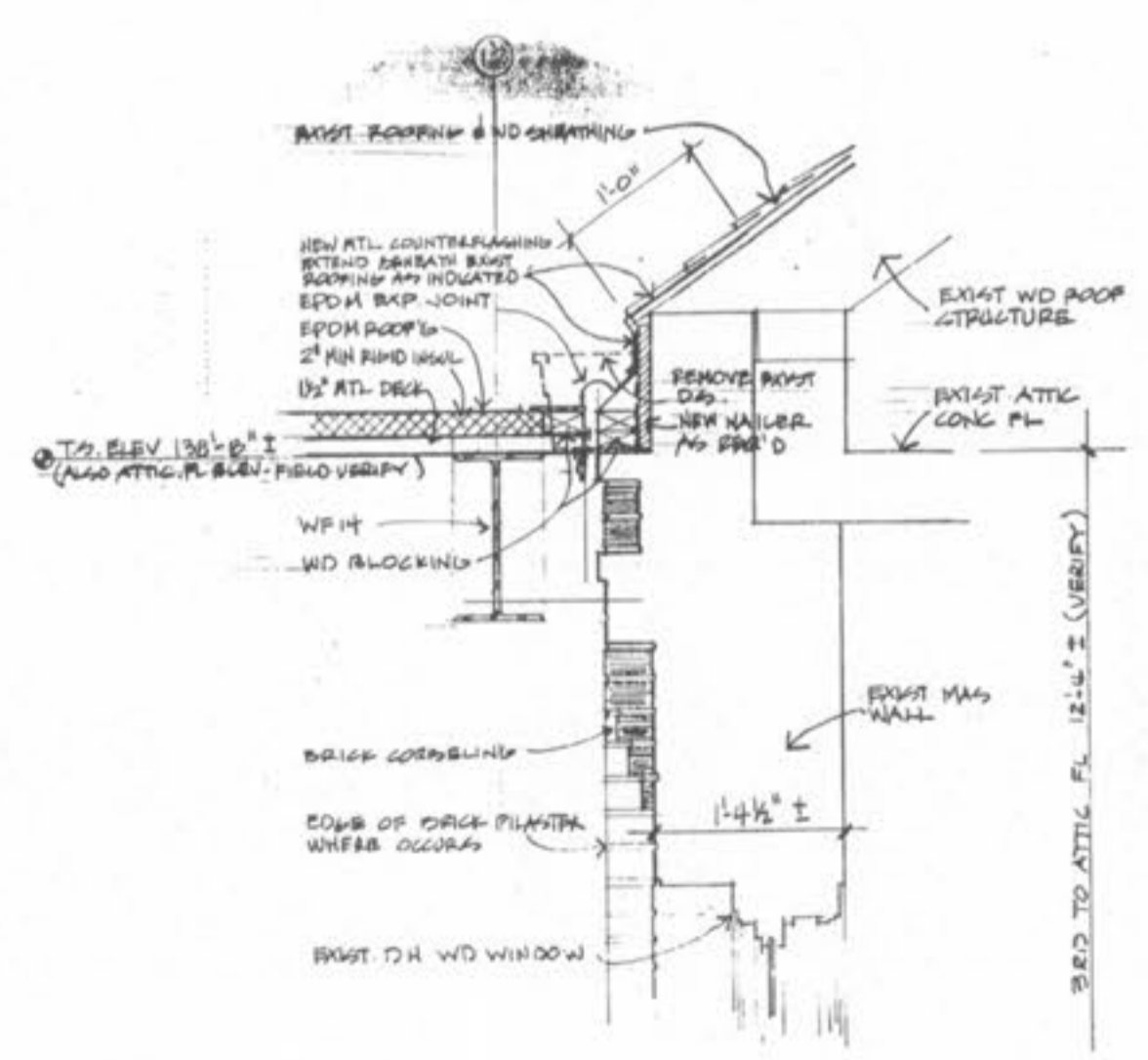
1 DETAIL • EXIST WEST WING ROOF/CENTRAL ROOF A-5 SCALE: 3/4" = 1'-0"
