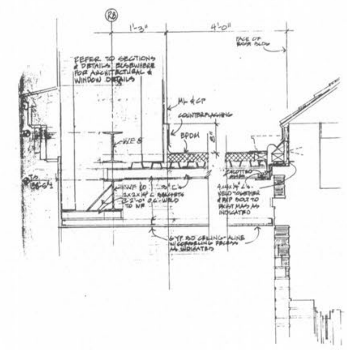
2 DETAIL • EXIST WEST WING ROOF/LOBBY ROOF A-5 SCALE: 3/4" = 1'-0"
