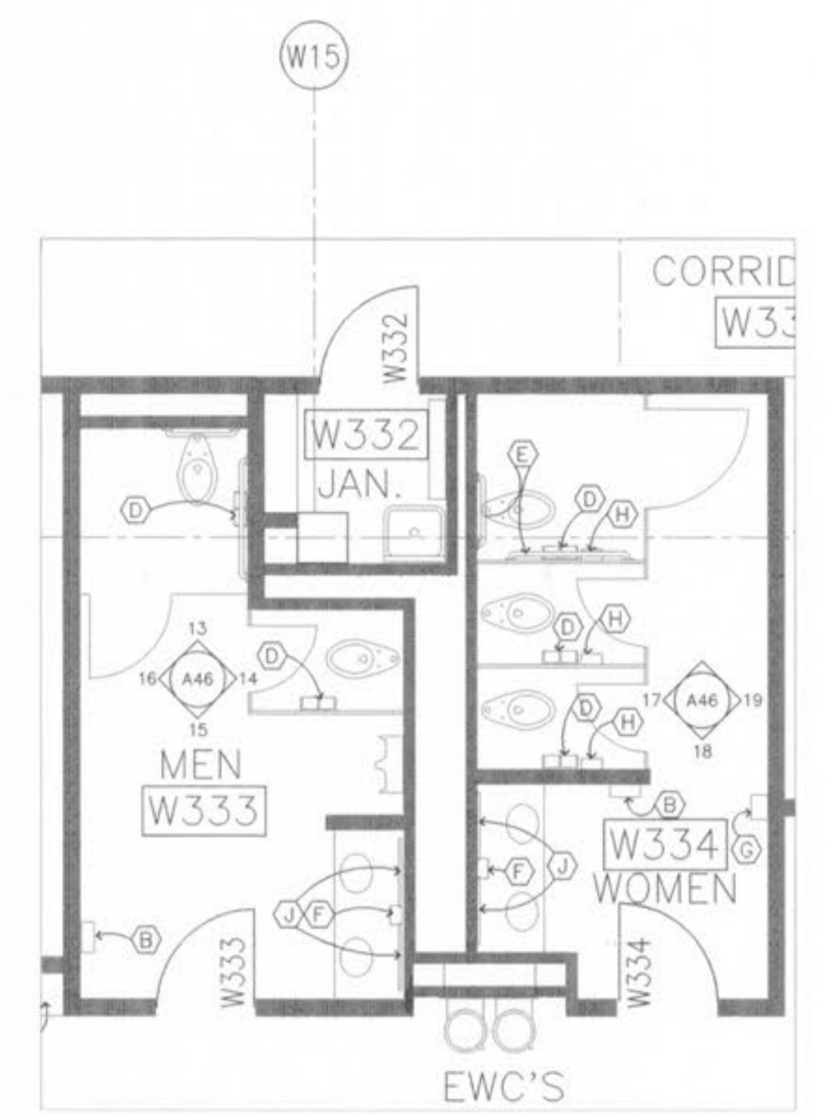
3 THIRD FLOOR TOILET PLAN SCALE: 1/4" = 1'-0"
