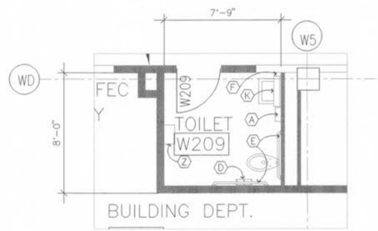
5 SECOND FLOOR TOILET PLAN SCALE: 1/4" = 1'-0"
