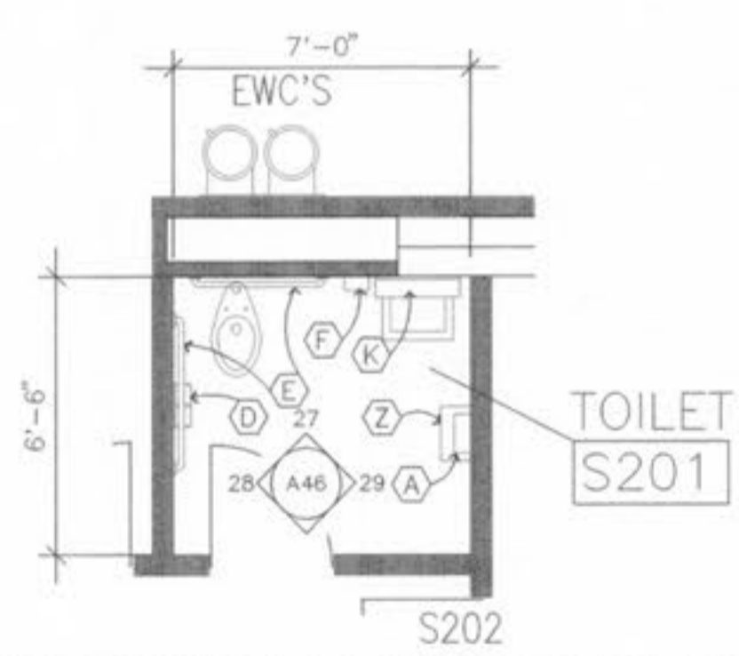
8 SECOND FLOOR TOILET PLAN SCALE: 1/4" = 1'-0"
