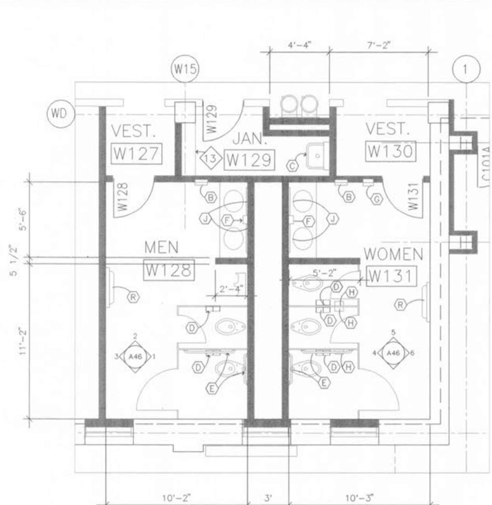
1 FIRST FLOOR TOILET PLAN SCALE: 1/4" = 1'-0"
