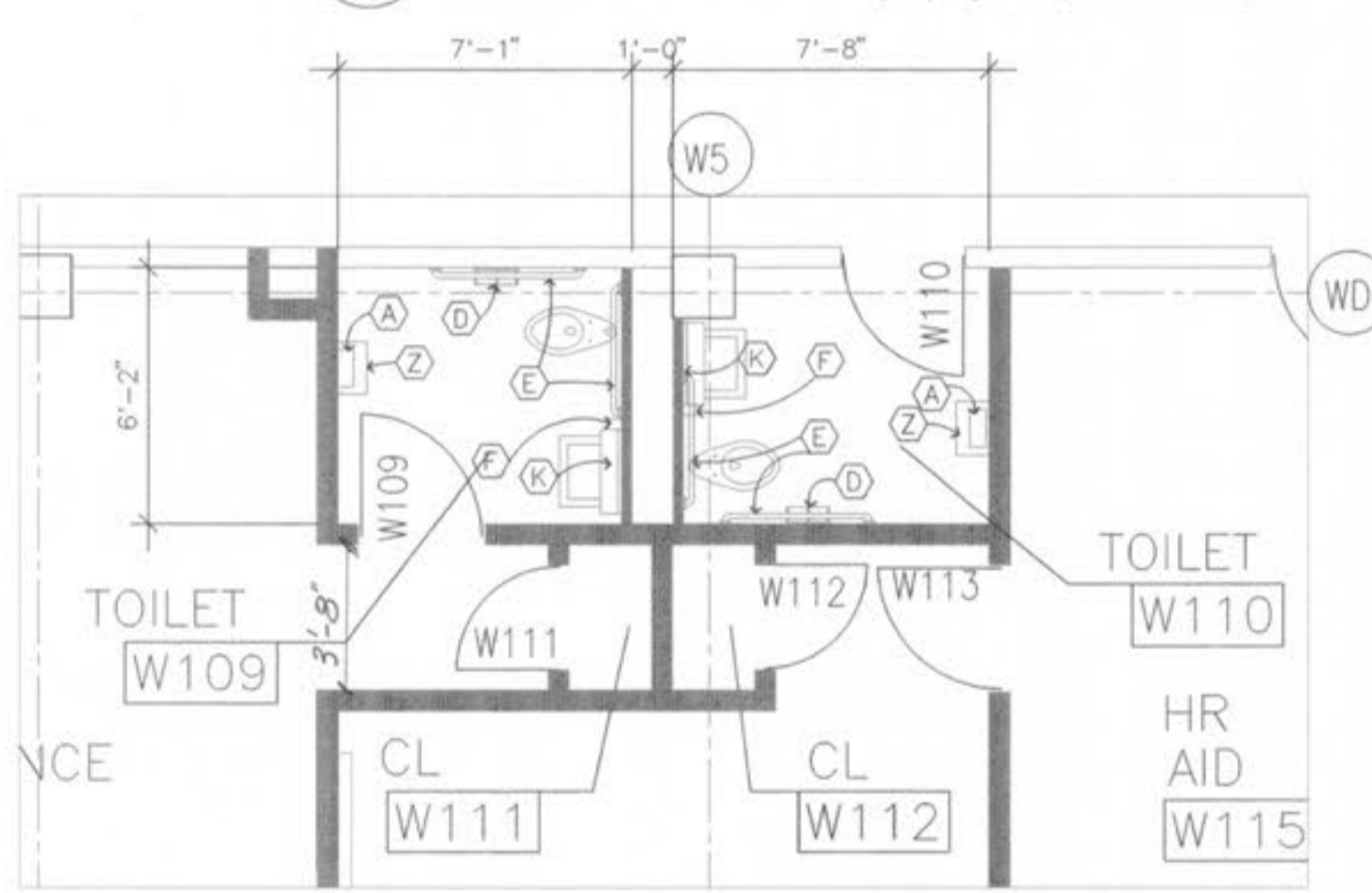
1 FIRST FLOOR TOILET PLAN SCALE: 1/4" = 1'-0"
