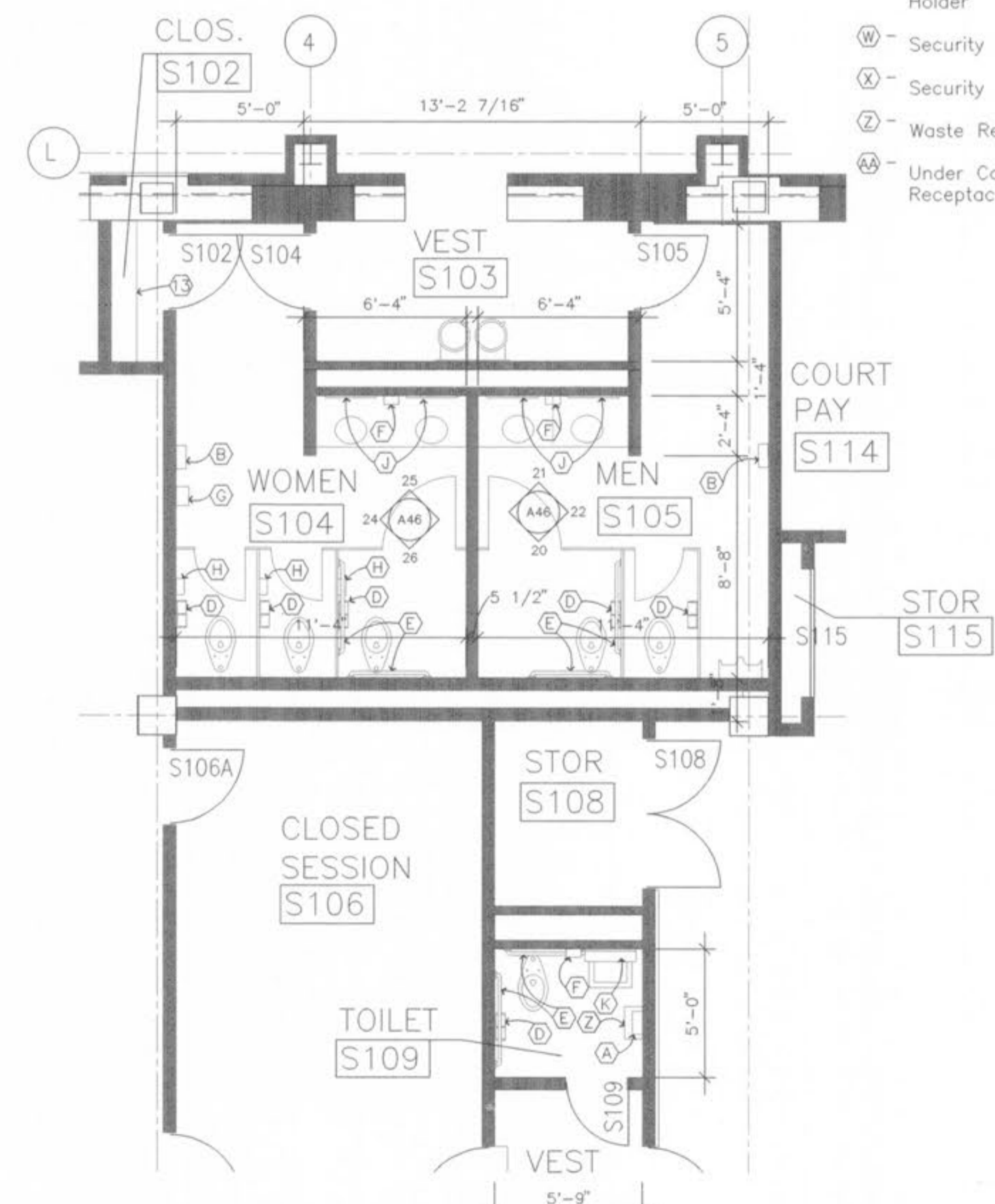
7 FIRST FLOOR TOILET PLAN SCALE: 1/4" = 1'-0"
