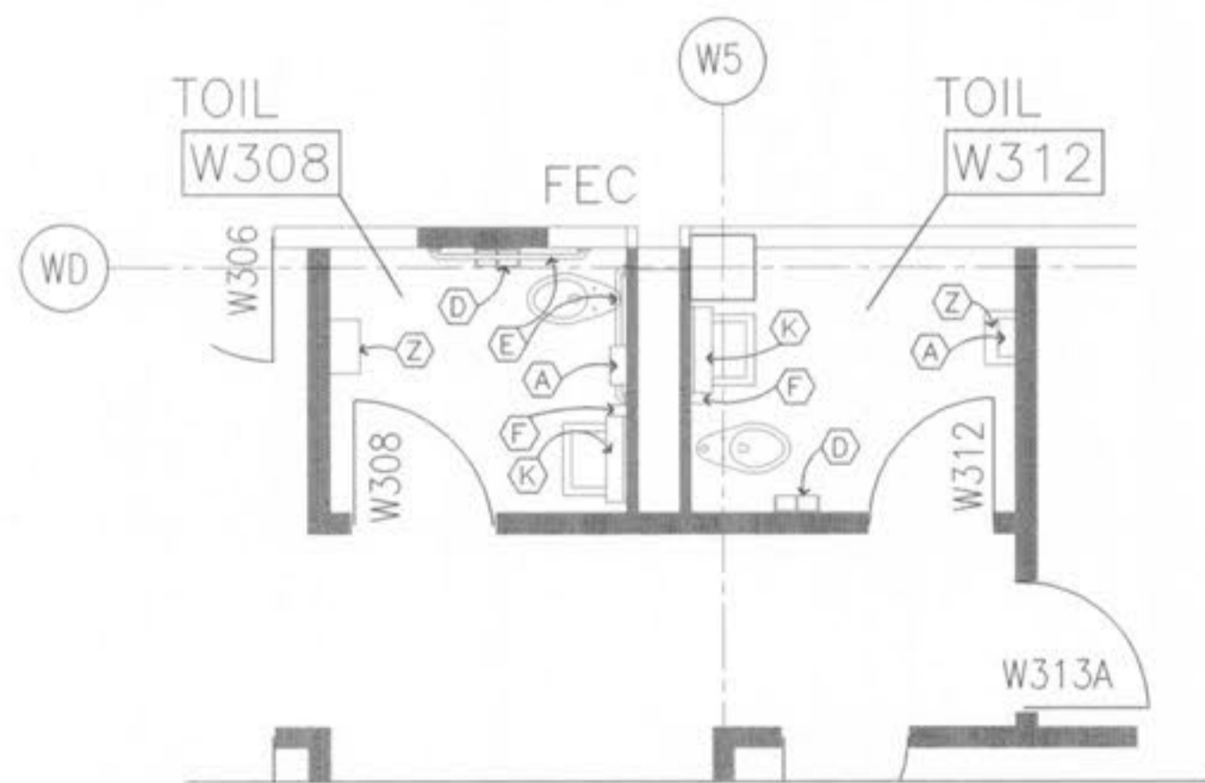
6 THIRD FLOOR TOILET PLAN SCALE: 1/4" = 1'-0"
