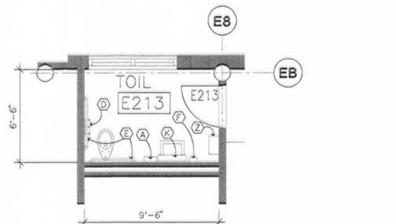
8 SECOND FLOOR TOILET PLAN SCALE: 1/4" = 1'-0"
