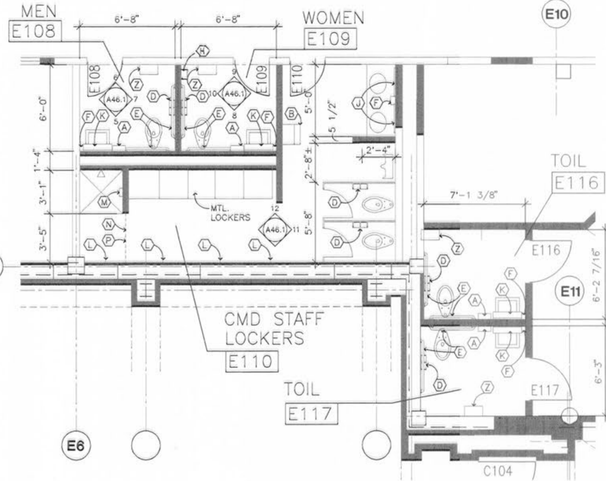
2 FIRST FLOOR TOILET PLAN SCALE: 1/4" = 1'-0"
