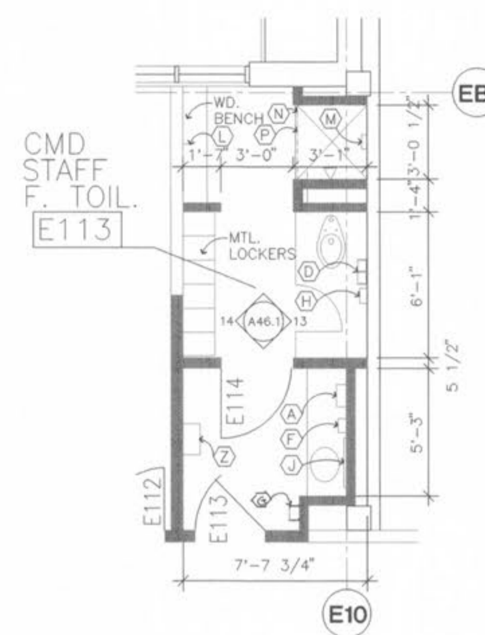
3 FIRST FLOOR TOILET PLAN SCALE: 1/4" = 1'-0"
