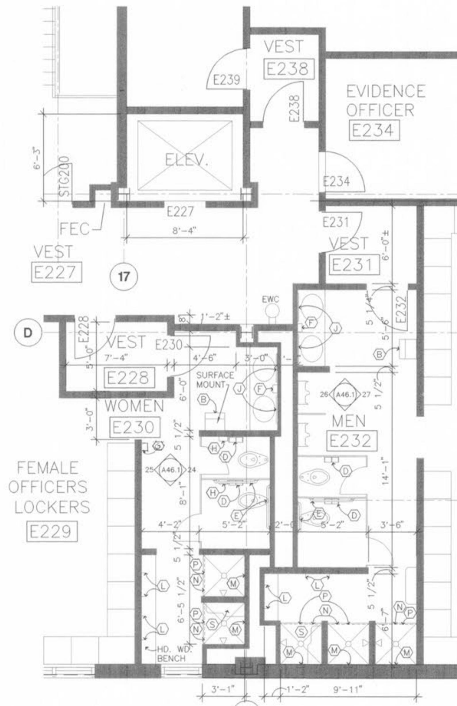
7 SECOND FLOOR TOILET PLAN SCALE: 1/4" = 1'-0"
