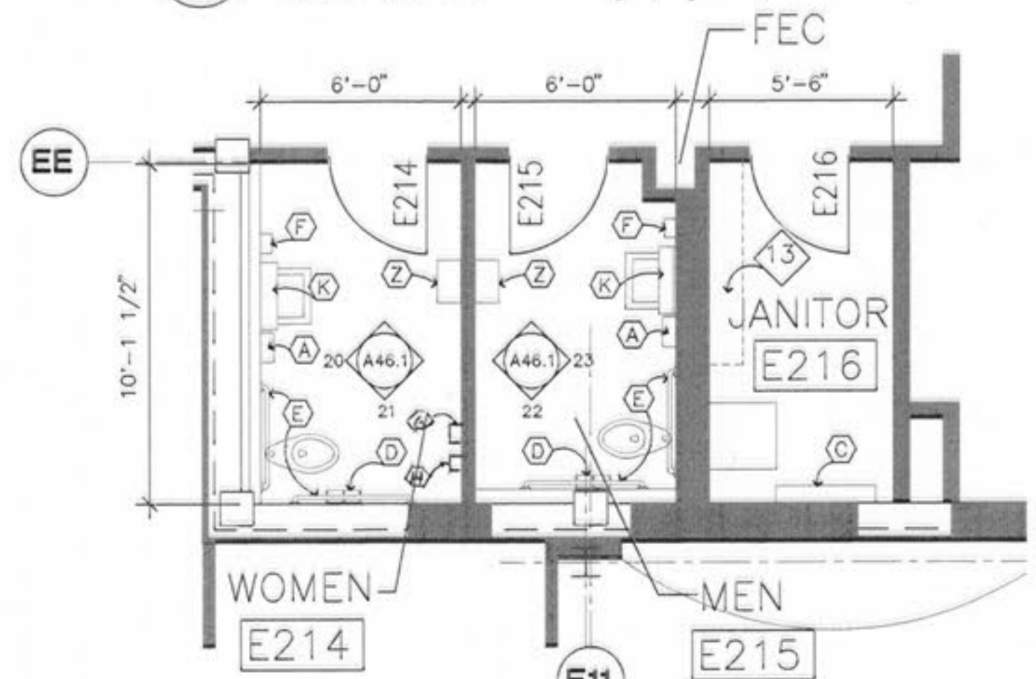
6 SECOND FLOOR TOILET PLAN SCALE: 1/4" = 1'-0"
