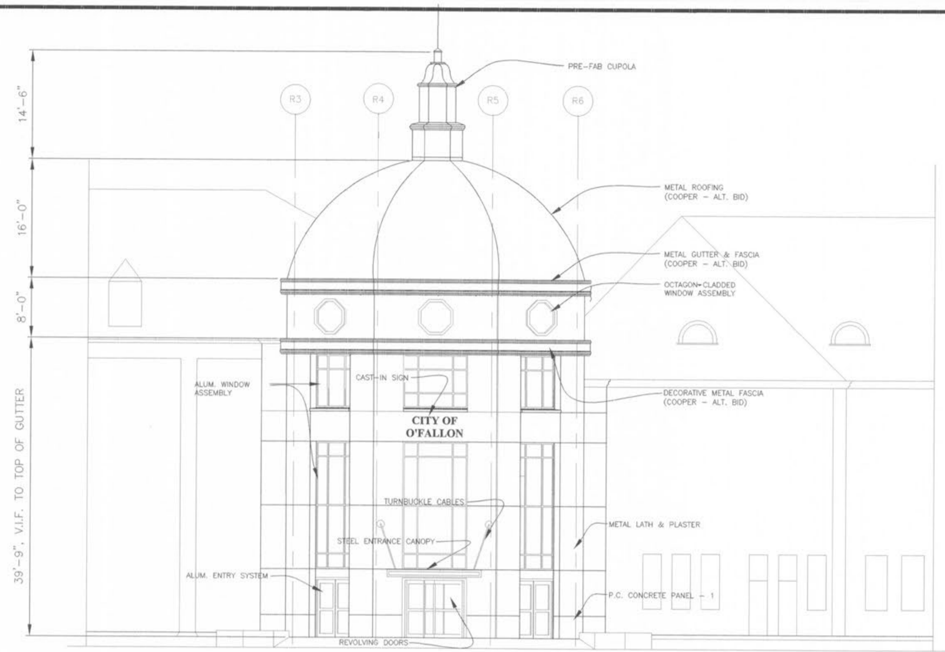
2 SOUTHWEST ELEVATION @ W. ENTRANCE SCALE: 1/8" = 1'-0"
