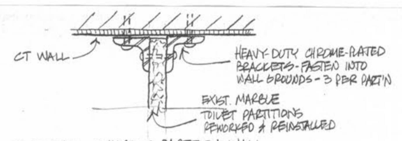
5 DETAIL @ MARBLE PARTITION WALL 3" = 1'-0"
