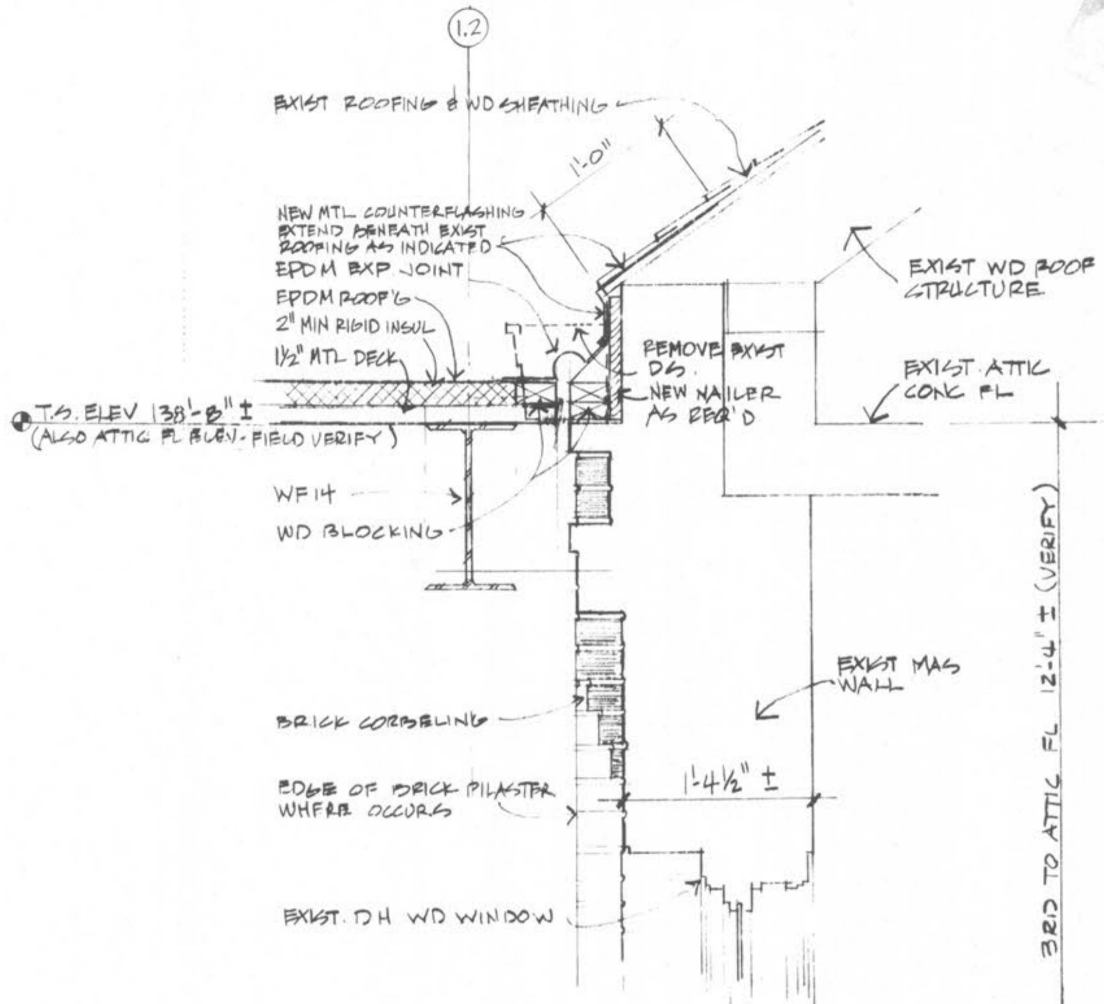
1 DETAIL @ EXIST WEST WING ROOF / CENTRAL ROOF SCALE = 1'-0"
