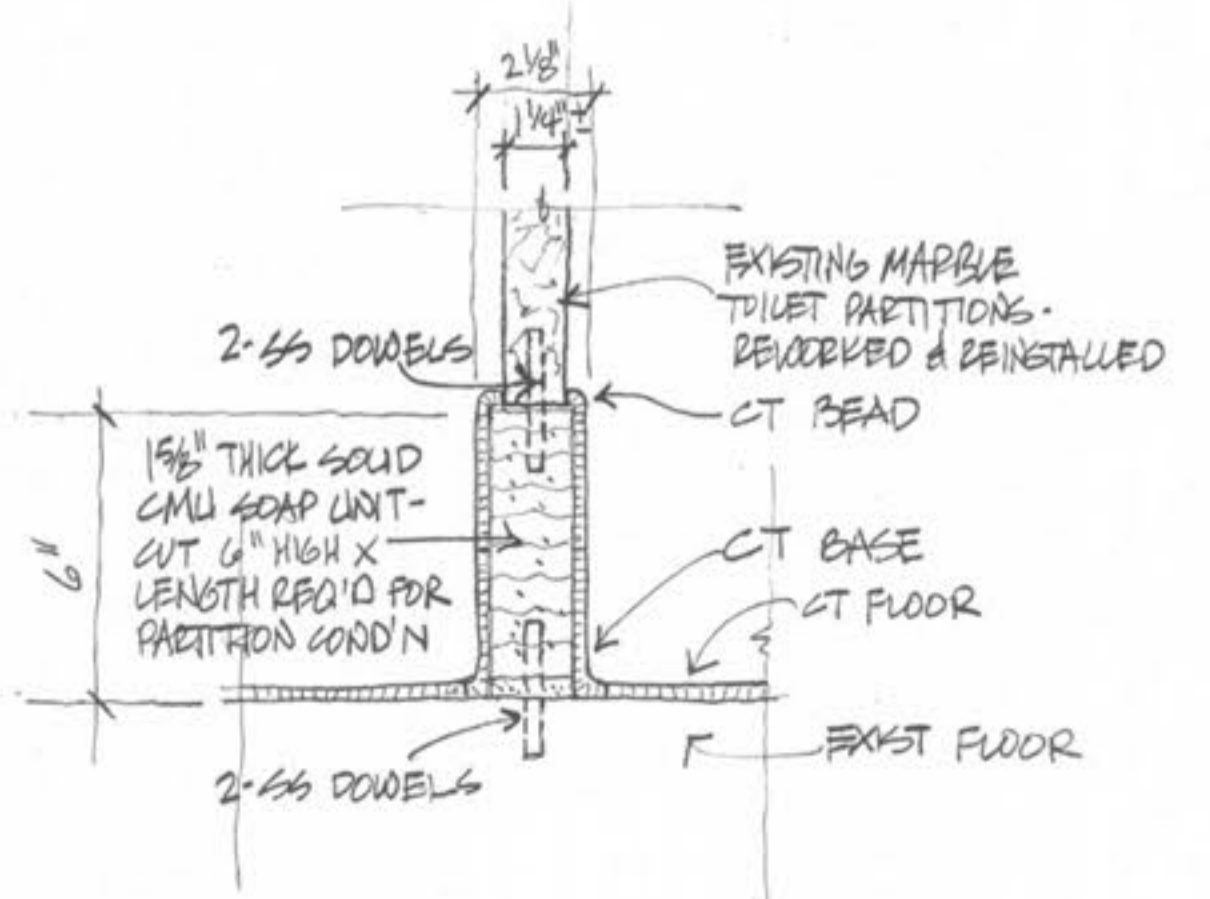
6 DETAIL @ MARBLE PARTITION BASE 3" = 1'-0"
