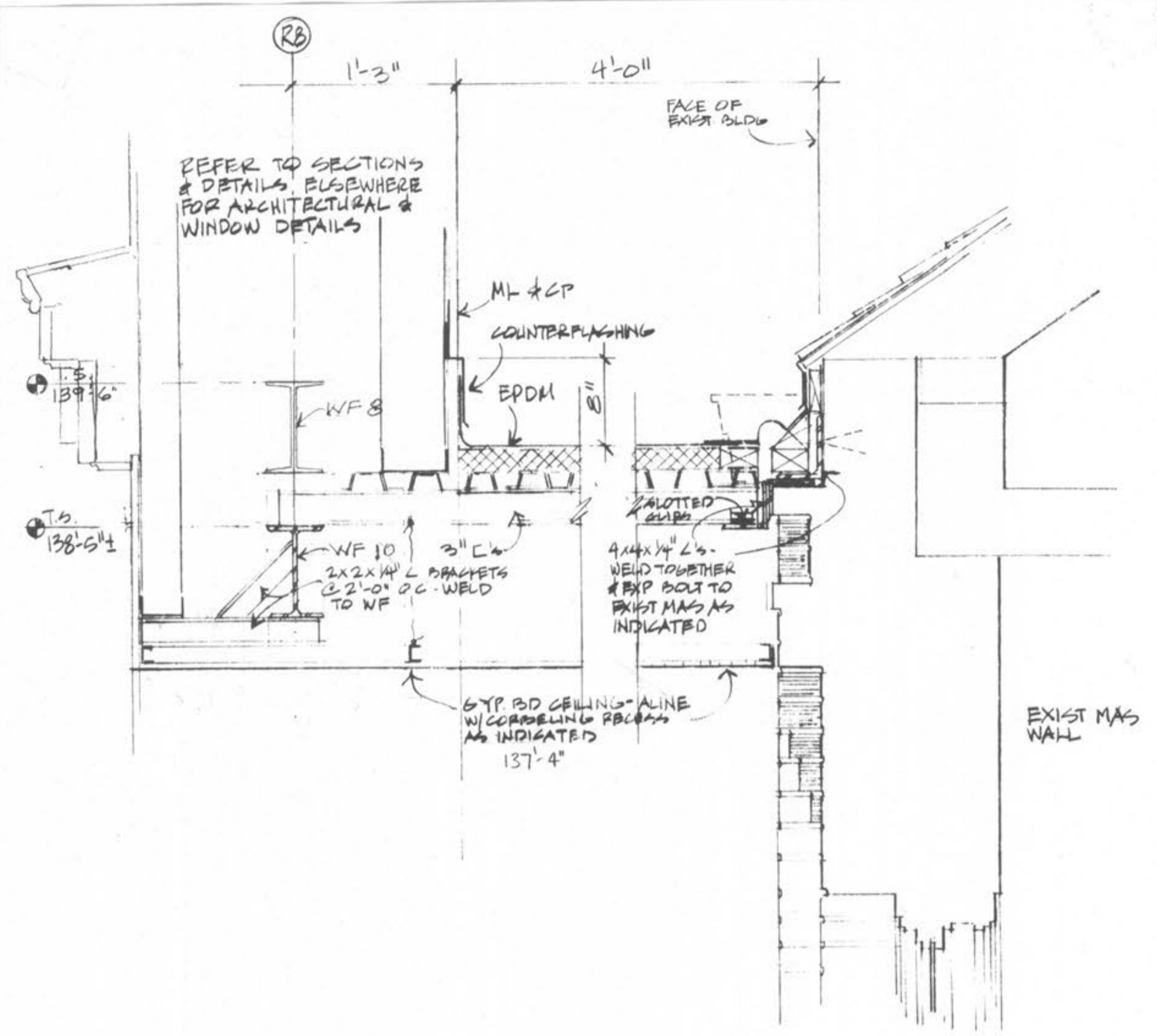
2 DETAIL @ EXIST WEST WING ROOF / LOBBY ROOF SCALE = 1'-0"
