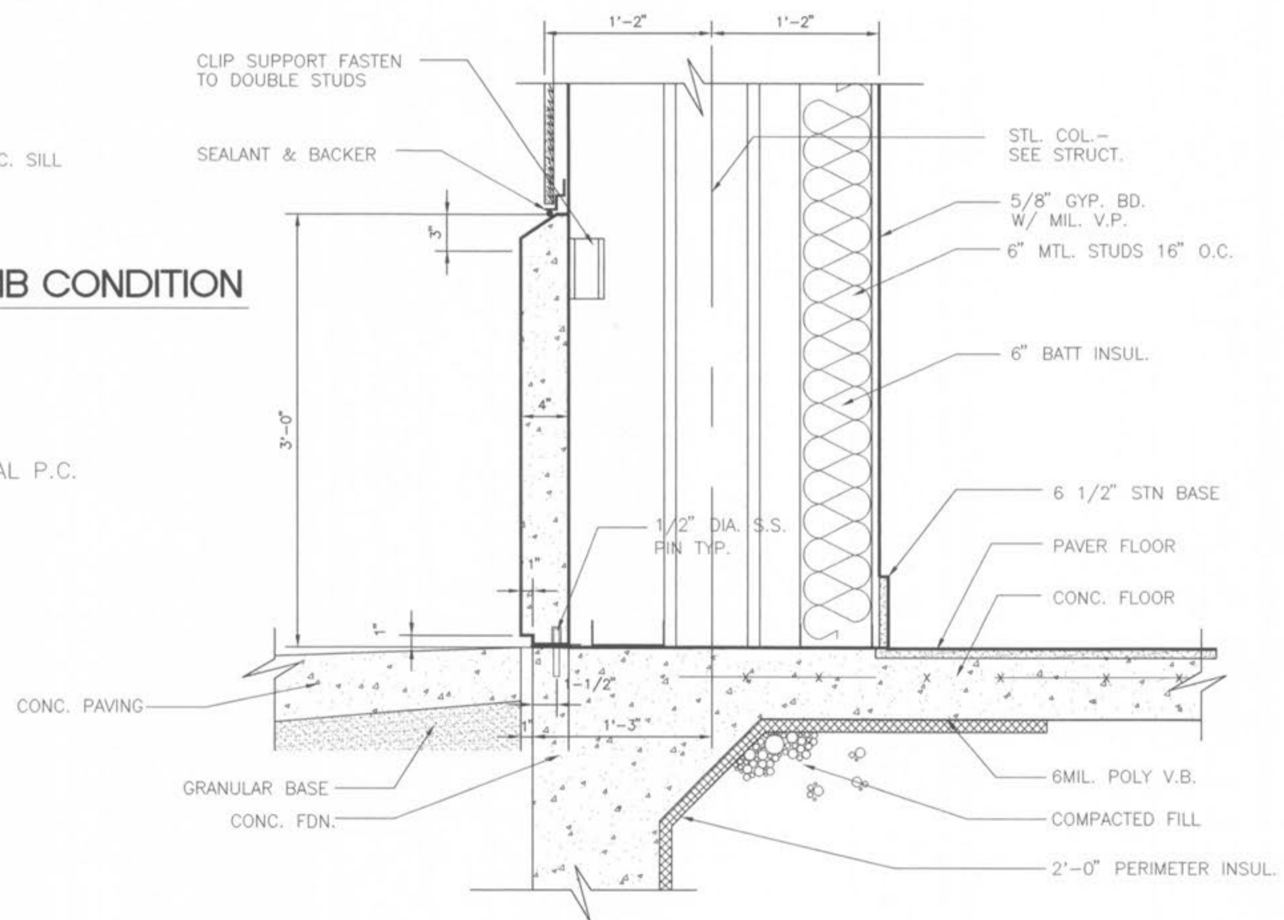
1 BASE CONDITION DETAIL A-39.1 SCALE: 1 1/2"=1'-0"
