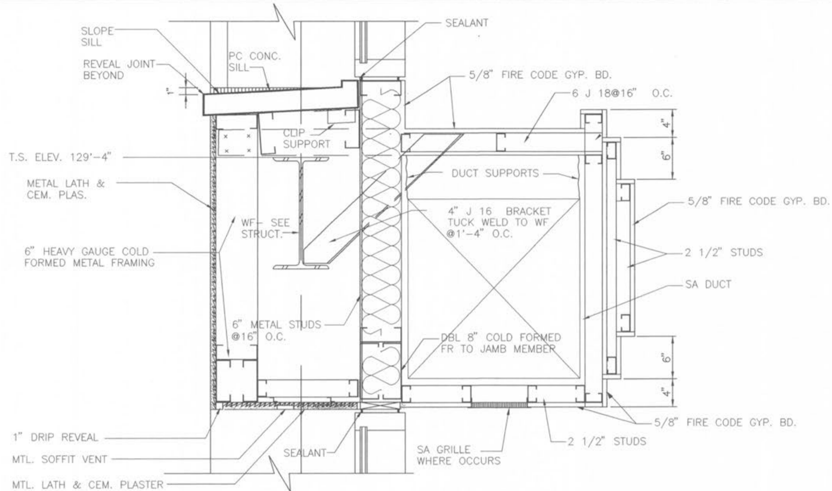
2 PLASTER ALTERNATE SPANDREL PANEL + DUCT SOFFIT DETAIL A-39.1 SCALE: 1 1/2"=1'-0"
