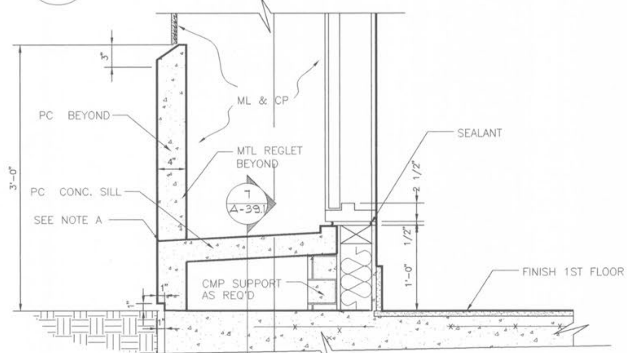
6 SILL CONDITION DETAIL A-39.1 SCALE: 1 1/2"=1'-0"
