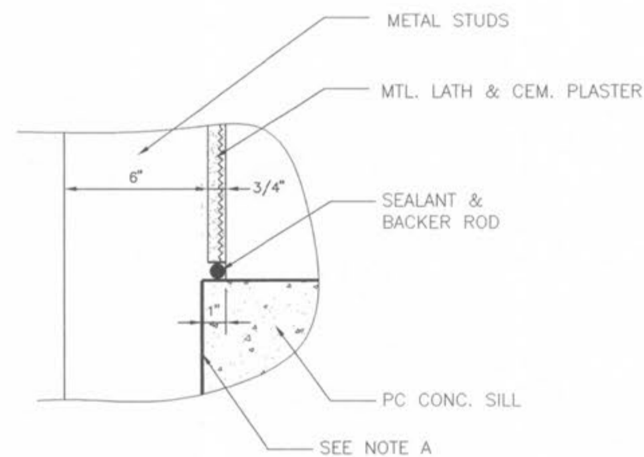
7 DETAIL @ SILL JAMB CONDITION A-39.1 SCALE: 3"=1'-0"
