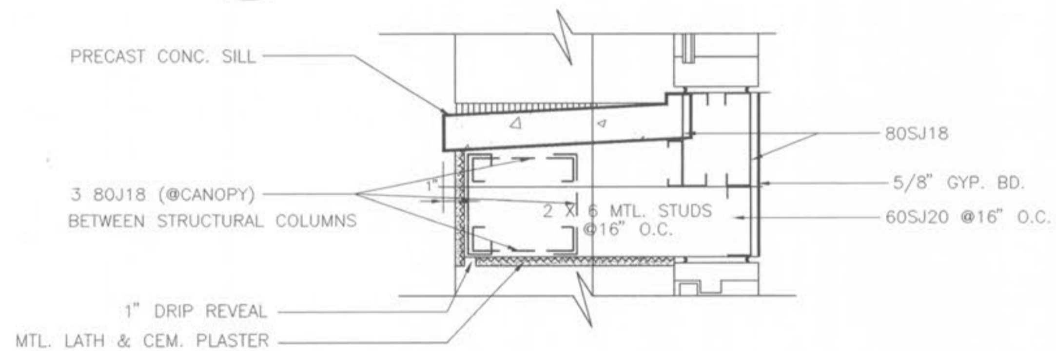
5 HEAD CONDITION DETAIL @ ENTRY DOOR A-39.1 SCALE: 1 1/2"=1'-0"
