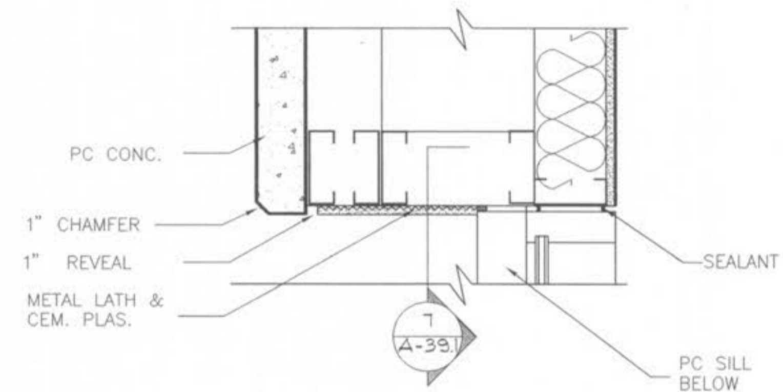
3 PLASTER JAMB CONDITION @ BASE A-39.1 SCALE: 1 1/2"=1'-0"
