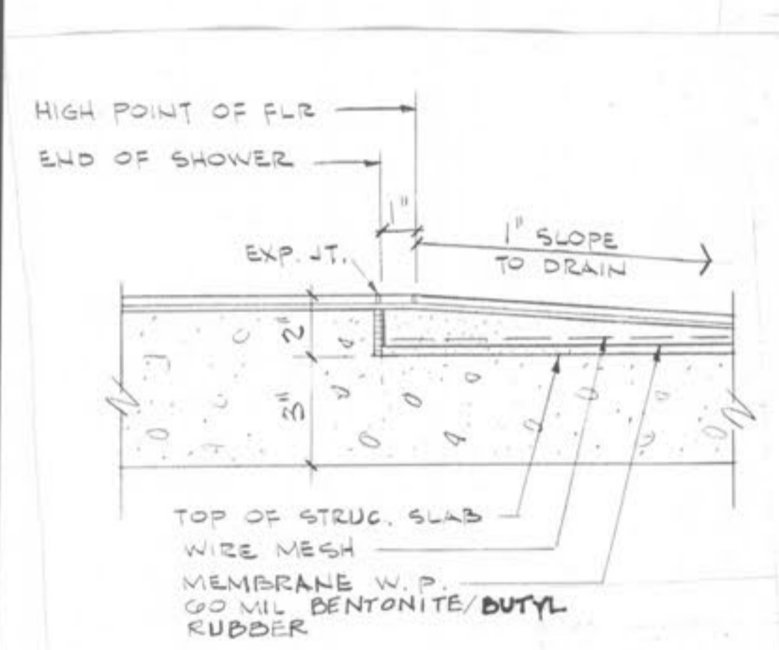
13 ACCESSIBLE SHOWER SCALE 3/4"=1'-0"
