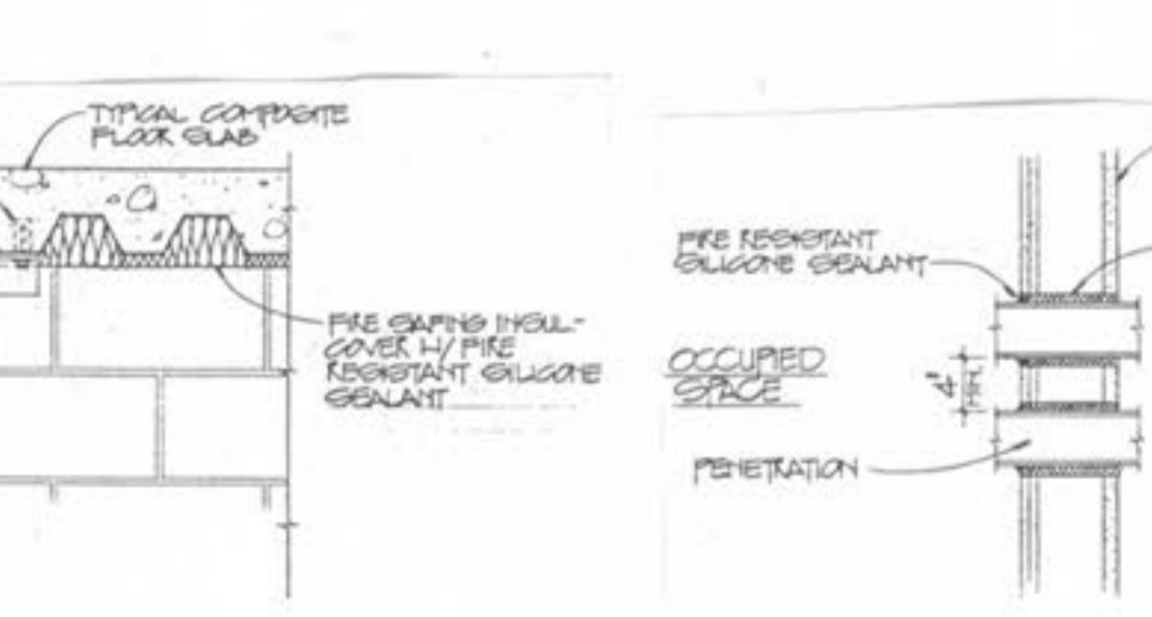
20 DETAIL @ MASONRY PARTITION SCALE: 3/4"=1'-0" (PERPENDICULAR TO DECK)
