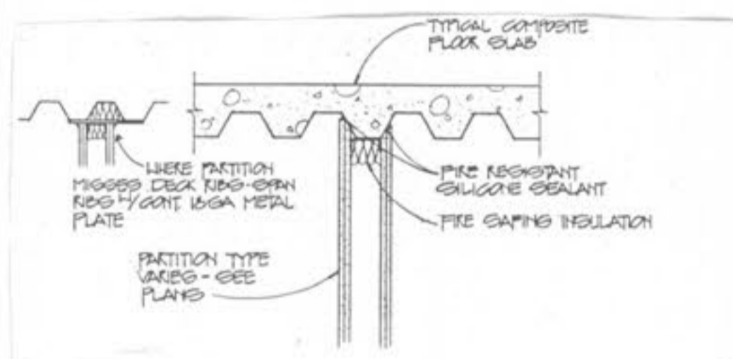
14 DETAIL @ RATED PARTITION SCALE: 3/4"=1'-0" (PARALLEL TO DECK)
