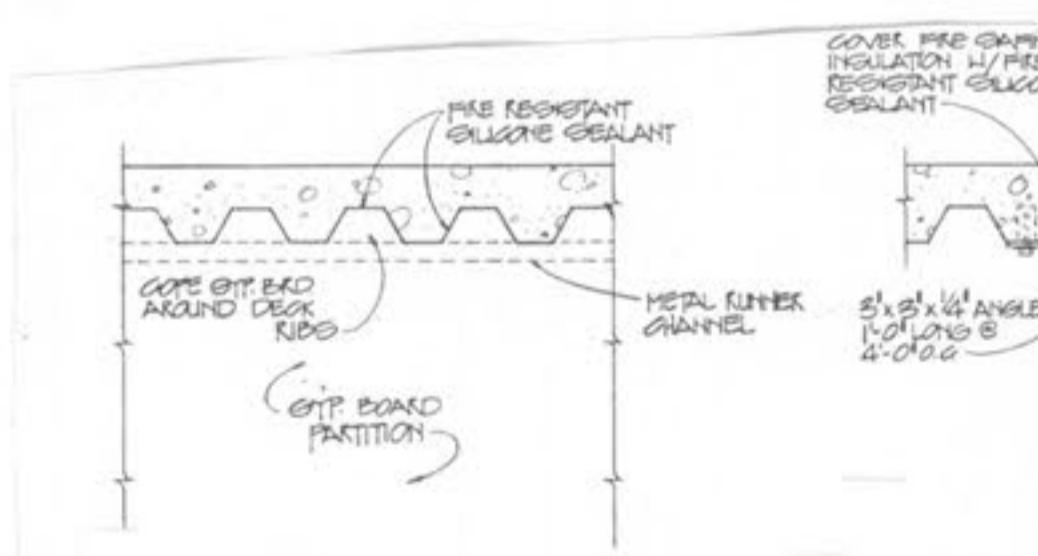
18 DETAIL @ NON-RATED PARTITION SCALE: 3/4"=1'-0" (PERPENDICULAR TO DECK)
