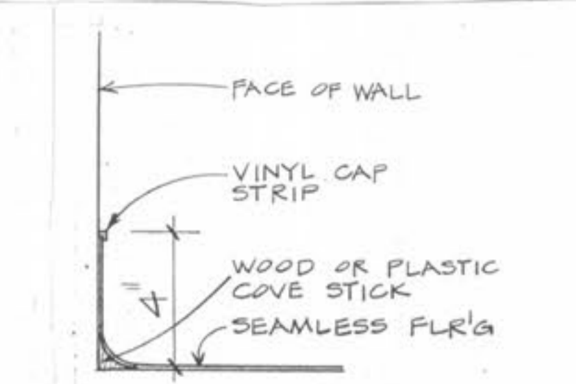
3 BASE DTL SCALE 3/4"=1'-0"
