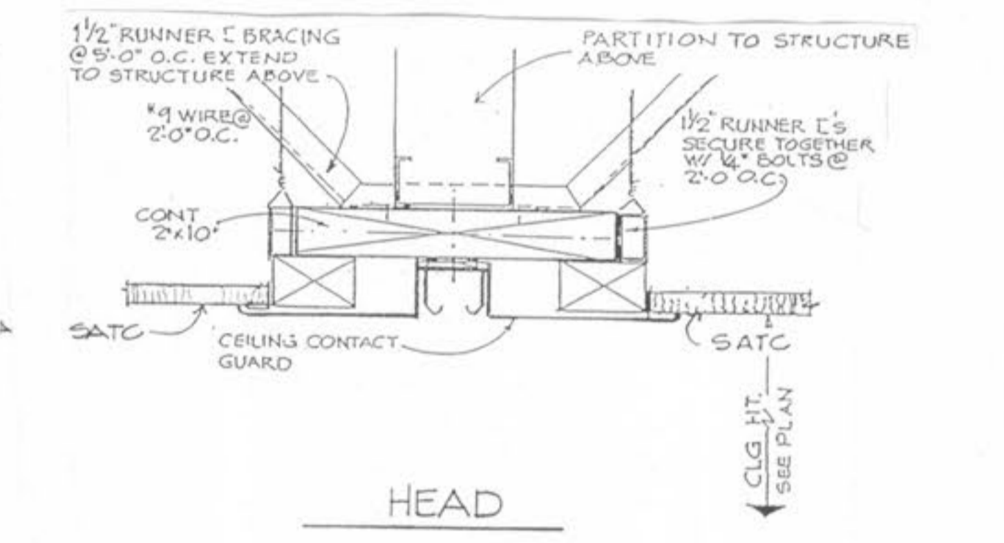
17 MULTI PURPOSE RM-OPERABLE PART SCALE 3/4"=1'-0"
