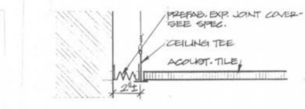
9 EXP. JT. @ ACOUST. TILE/WALL SCALE 3/4"=1'-0"
