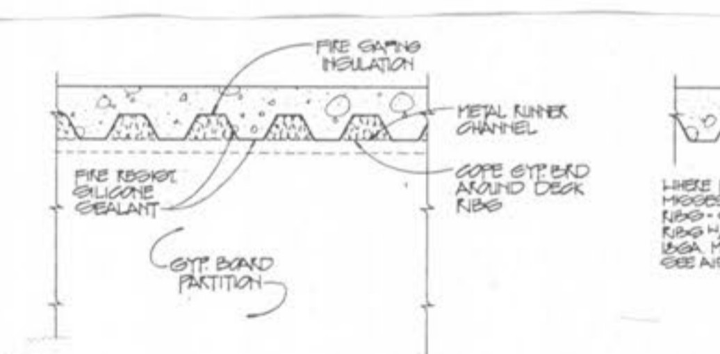
15 DETAIL @ RATED PARTITION SCALE: 3/4"=1'-0" (PERPENDICULAR TO DECK)
