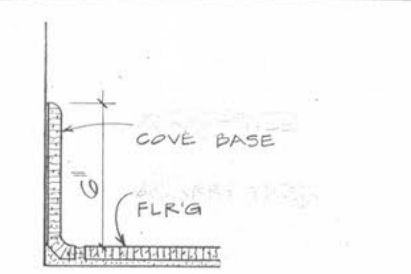
4 BASE DTL SCALE 3/4"=1'-0"
