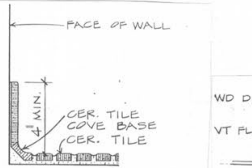
5 BASE DTL SCALE 3/4"=1'-0"
