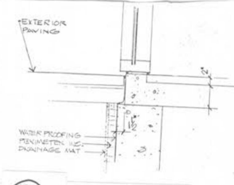
12A ENTRANCE FLR COND. SCALE 3/4"=1'-0"
