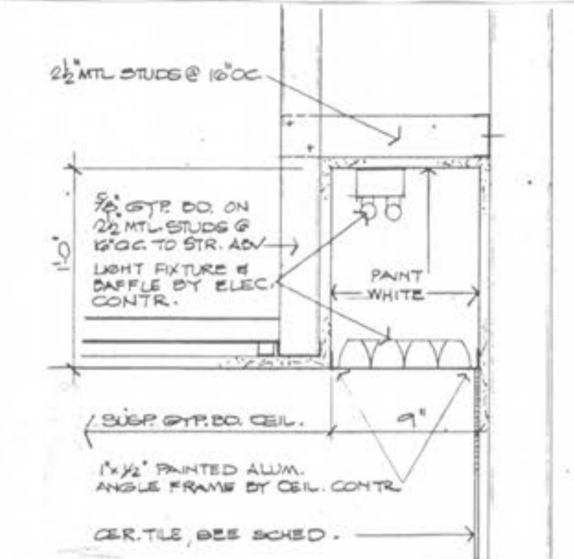
2 TOILET RM. LIGHT COVE @ GYP. BD. SCALE 3/4"=1'-0"
