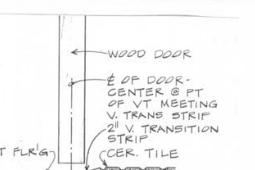
7 TRANS'N DTL SCALE 3/4"=1'-0"
