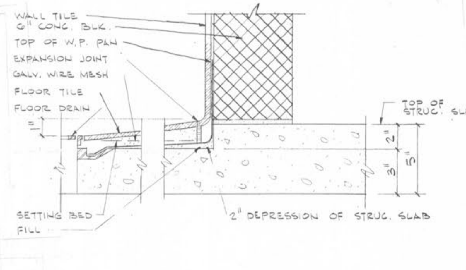
13 ACCESSIBLE SHOWER SCALE 3/4"=1'-0"
