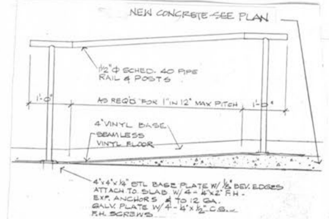
12 CORRIDOR RAISED FLR & RAMP SCALE 3/4"=1'-0"
