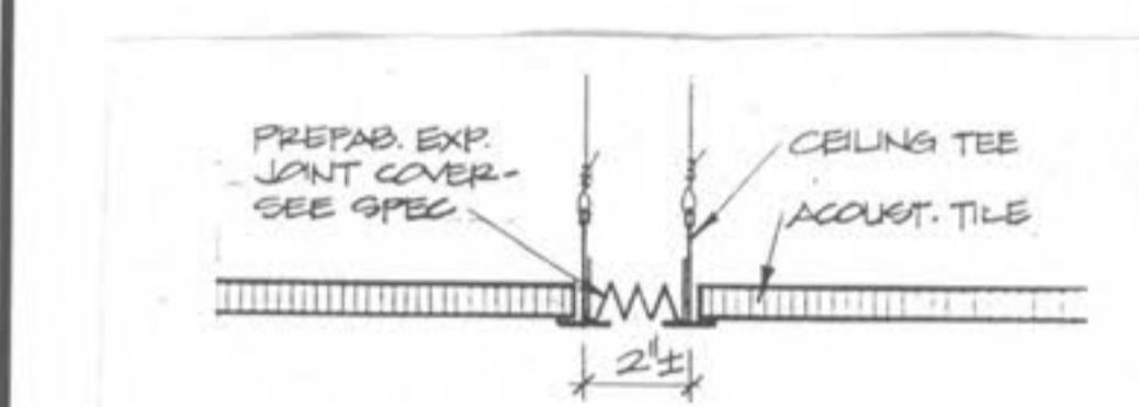
8 EXP. JT. @ ACOUST. TILE SCALE 3/4"=1'-0"
