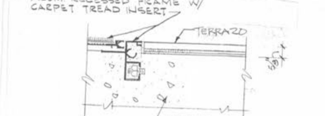
11 RECESSED MAT SCALE: HALF FULL SIZE
