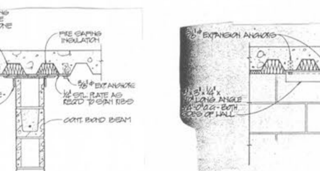
19 DETAIL @ MASONRY PARTITION SCALE: 3/4"=1'-0" (PARALLEL TO DECK)
