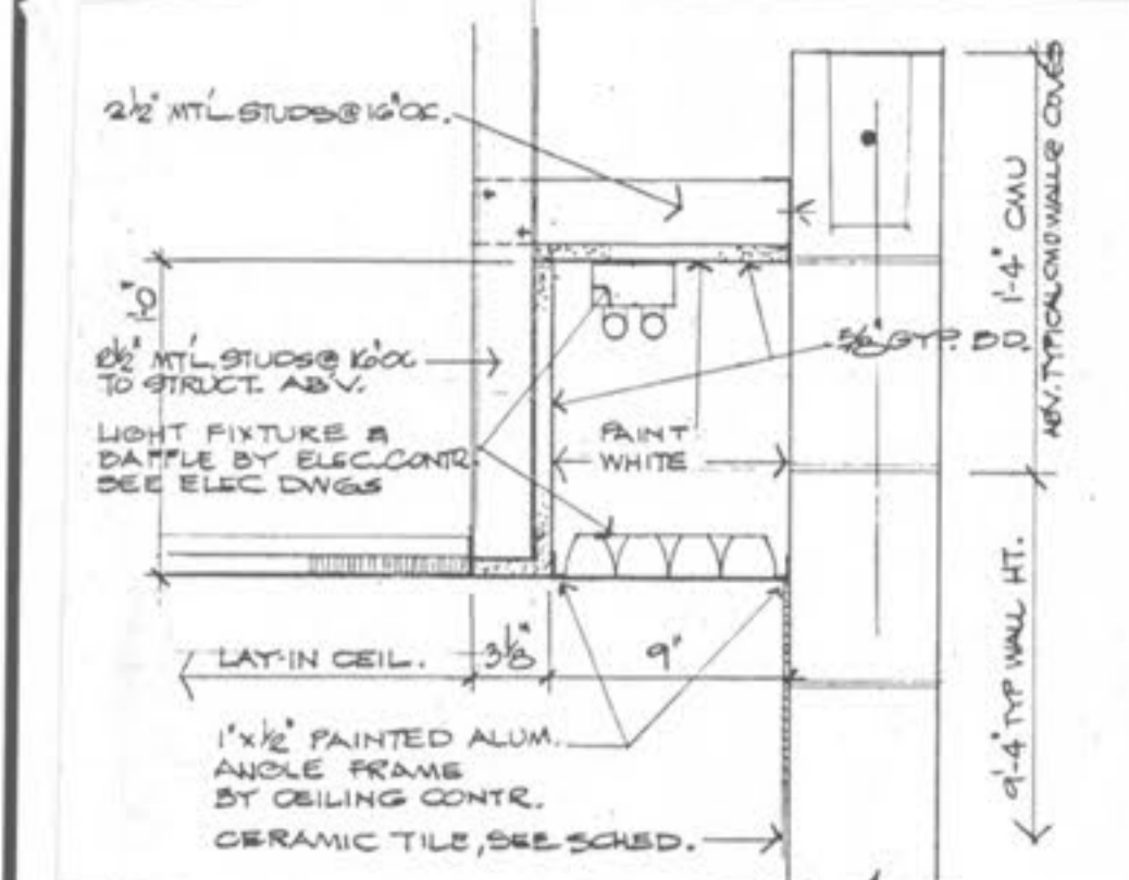
1 TOILET RM. LIGHT COVE @ ACT. SCALE 3/4"=1'-0"
