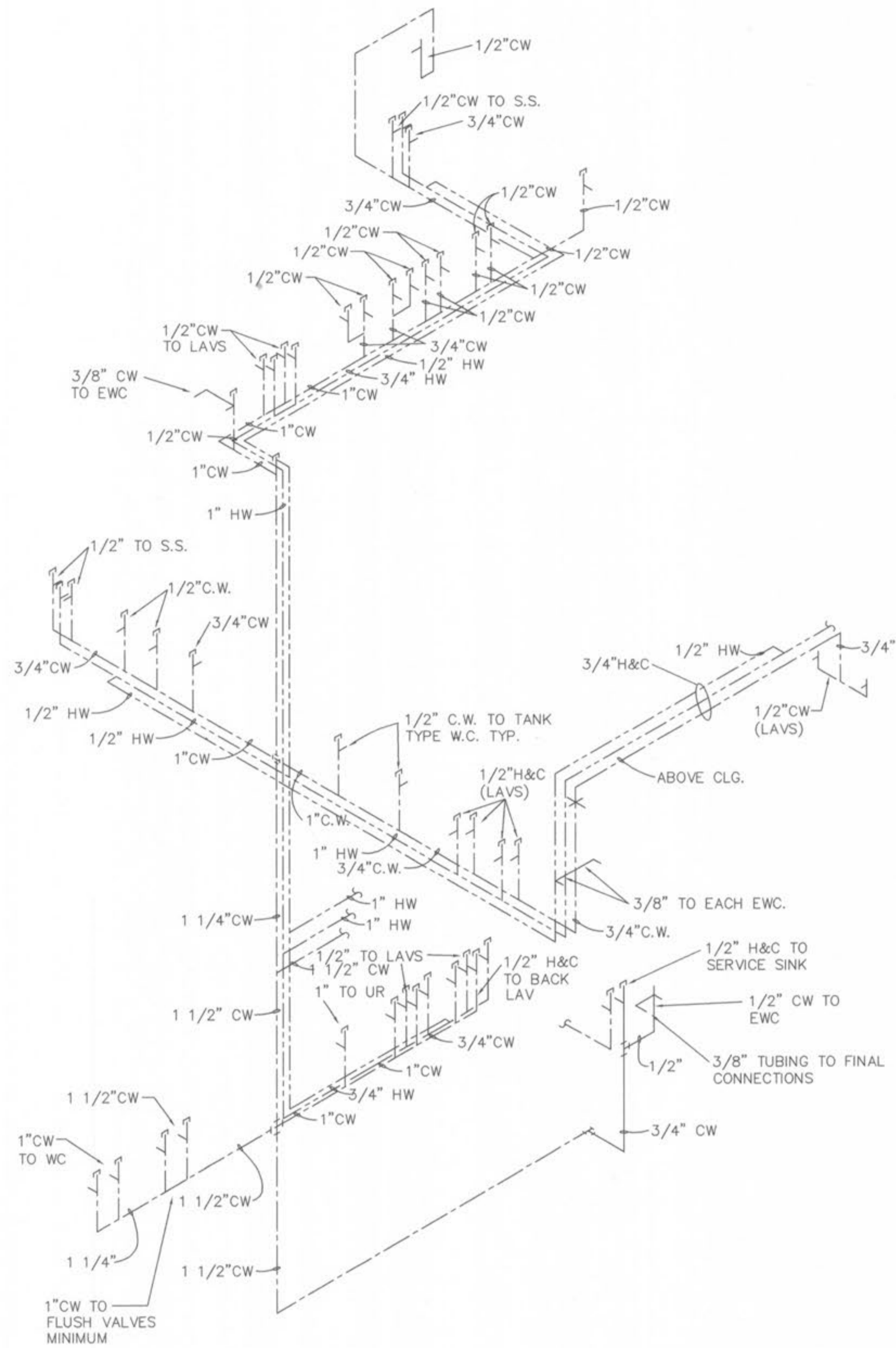
P I-B WATER ISOMETRIC WEST WING
