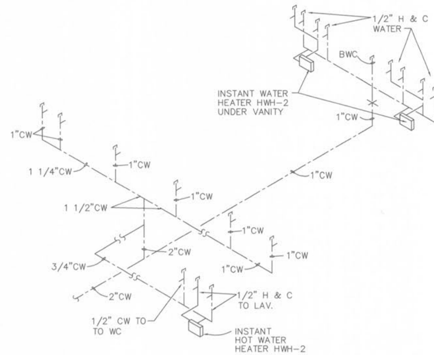
P I-D WATER ISOMETRIC SOUTH WING
