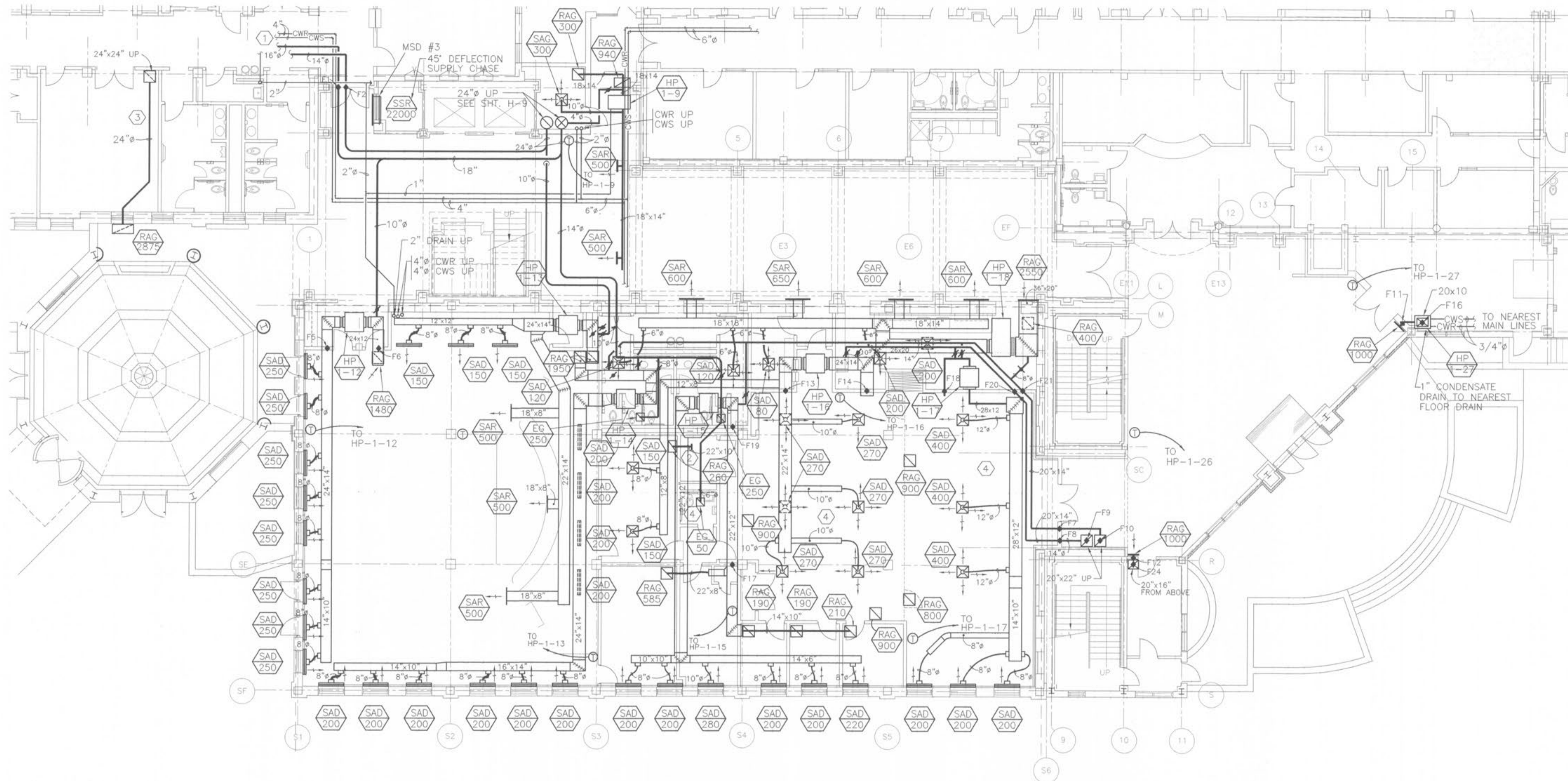
HVAC FIRST FLOOR PLAN - SOUTH WING SCALE: 1/8" = 1'-0"
