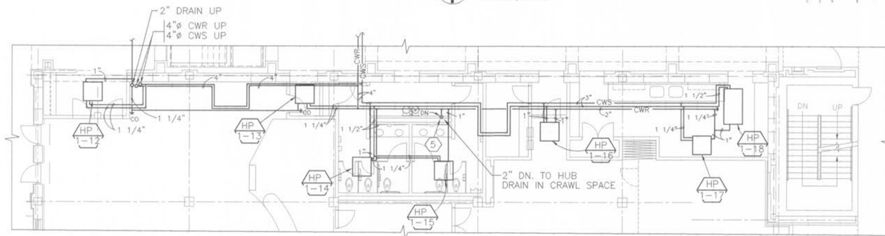
PARTIAL FIRST FLOOR PIPING PLAN - SOUTH WING SCALE: 1/8" = 1'-0"
