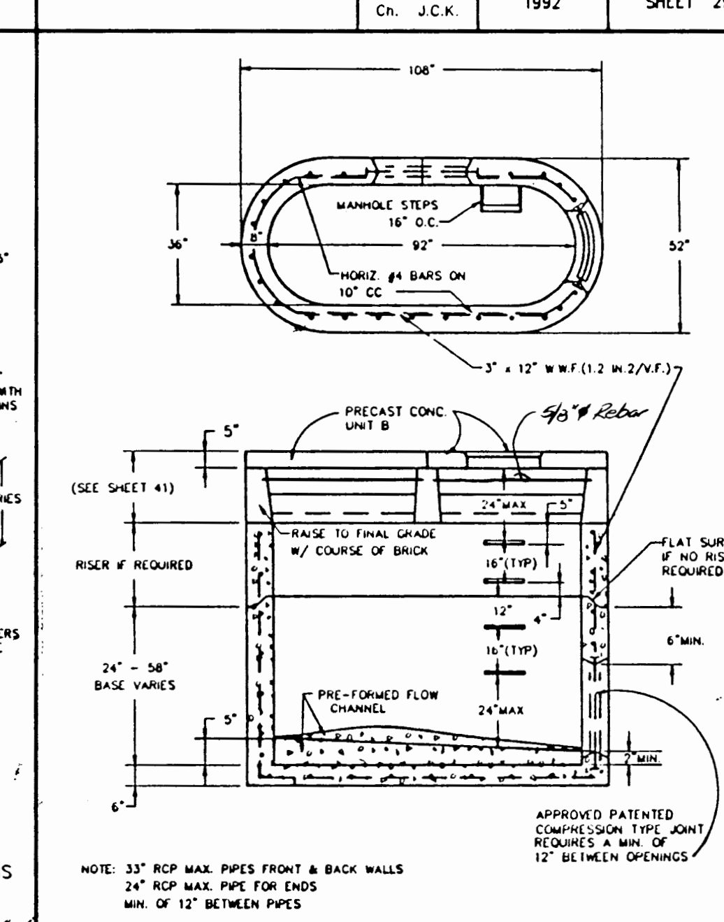
DOUBLE UNTRAPPED STREET INLET PRECAST CONCRETE METROPOLITAN ST. LOUIS SEWER DISTRICT Standard Details of Sewer Construction Dr. J.L.C. Ch. J.C.K. SEPT. 1992 SHEET 35
