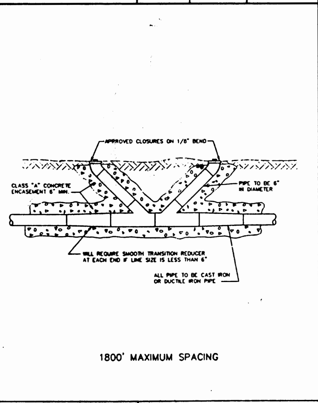
FORCE MAIN CLEANOUT (6" DIA. & SMALLER) METROPOLITAN ST. LOUIS SEWER DISTRICT Standard Details of Sewer Construction Dr. R.G.W. Ch. J.C.K. 1992 SHEET 65
