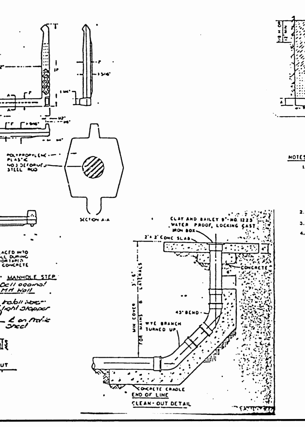
FORCE MAIN CLEANOUT (6" DIA. & SMALLER) METROPOLITAN ST. LOUIS SEWER DISTRICT Standard Details of Sewer Construction Dr. R.G.W. Ch. J.C.K. 1992 SHEET 65
