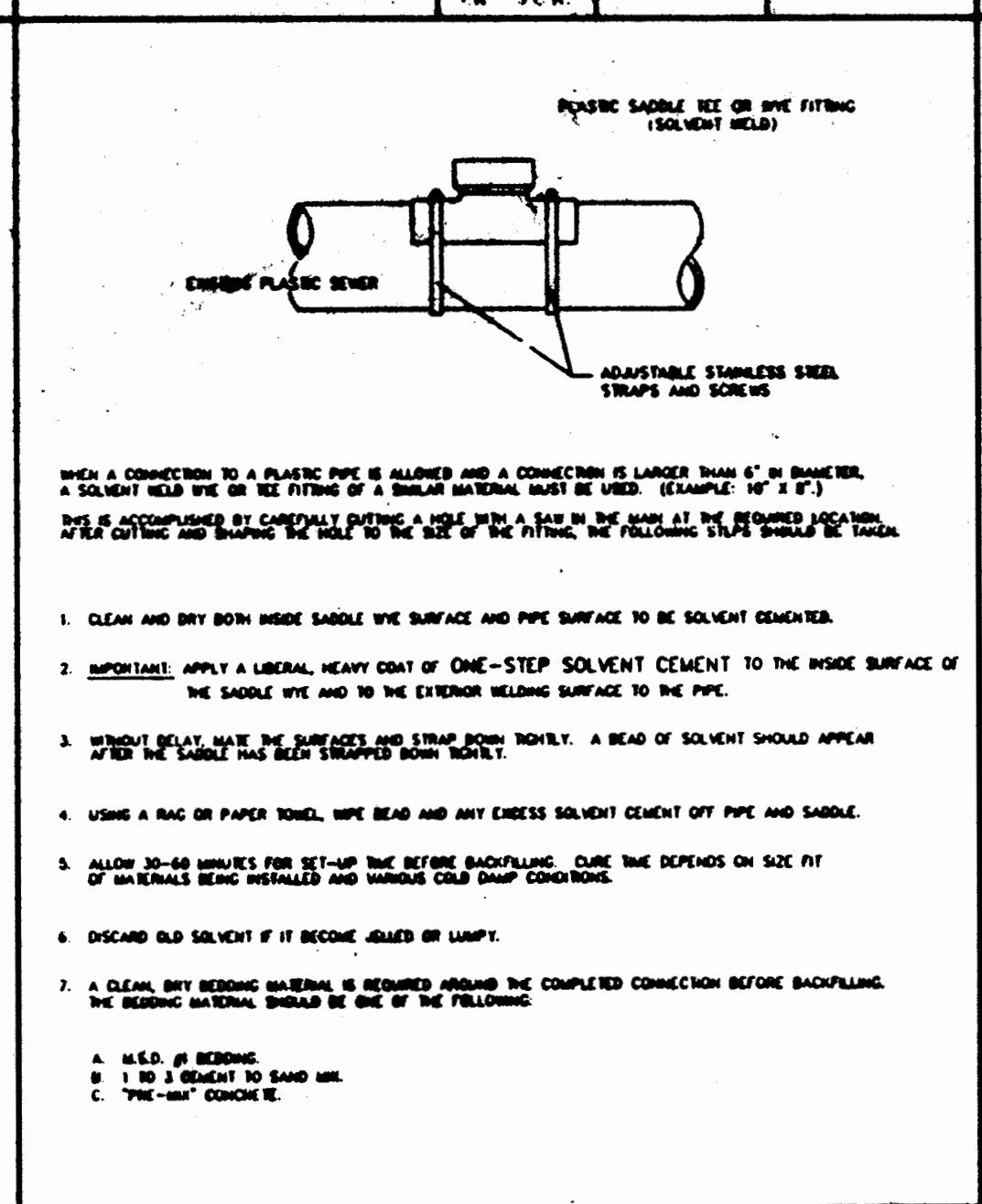
B' (& LARGER) CONNECTION TO PLASTIC MAIN METROPOLITAN ST. LOUIS SEWER DISTRICT Standard Details of Sewer Construction Dr. D.A.B. Ch. J.C.K. 1992 SHEET 62
