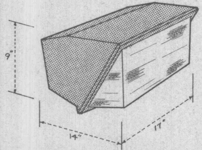
250/400 WATT WALL PACK LIGHTING DETAIL
