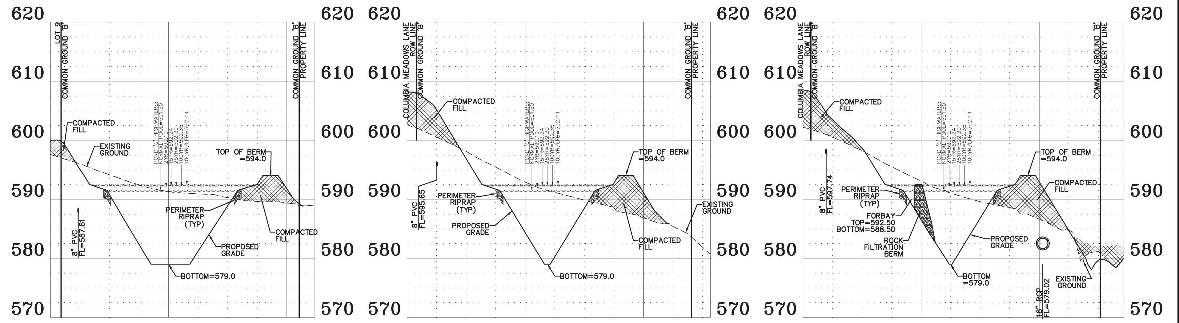
POND SECTION G-G
