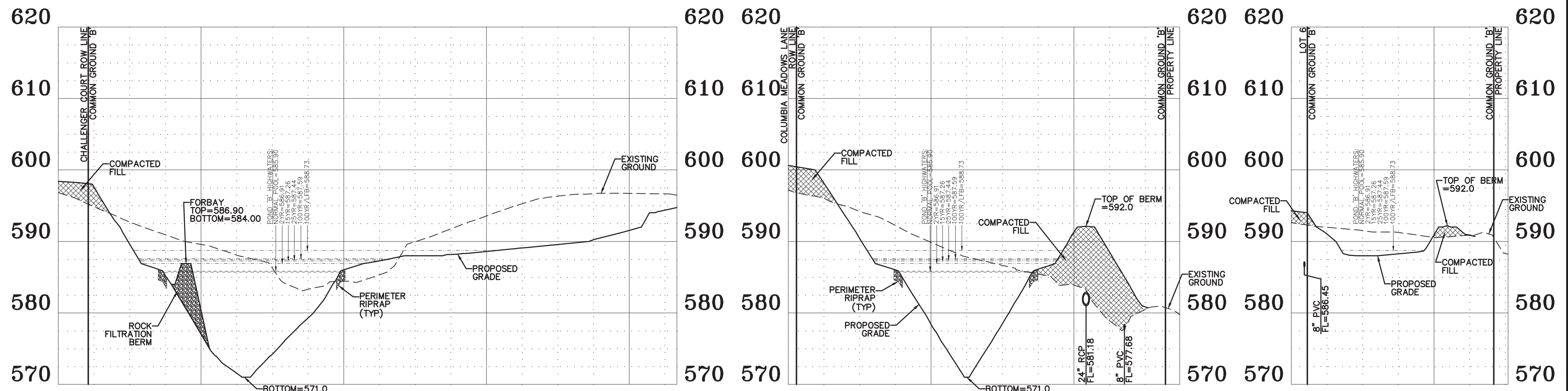
POND SECTION D-D
