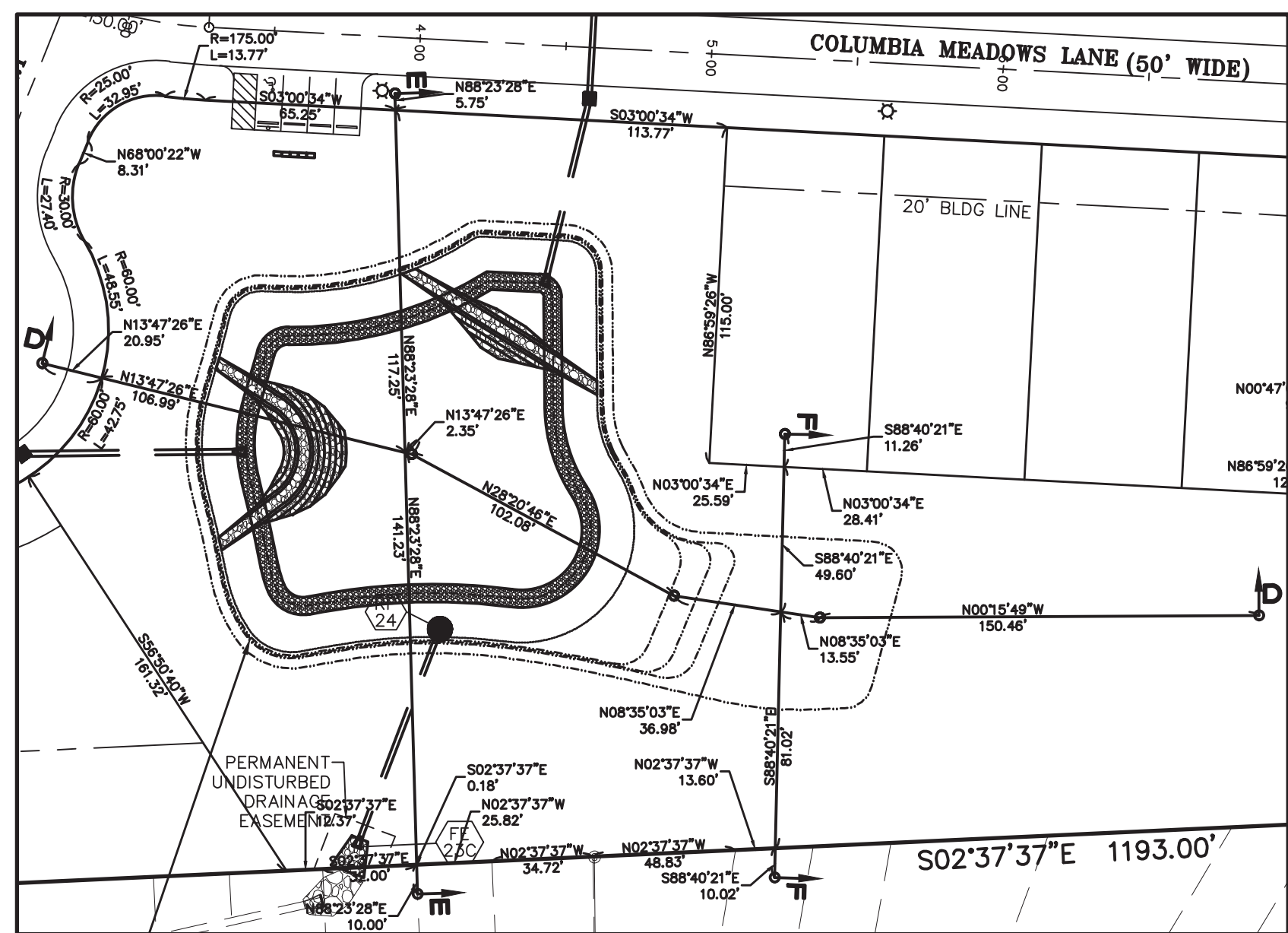
POND 'B' SECTION DETAIL
