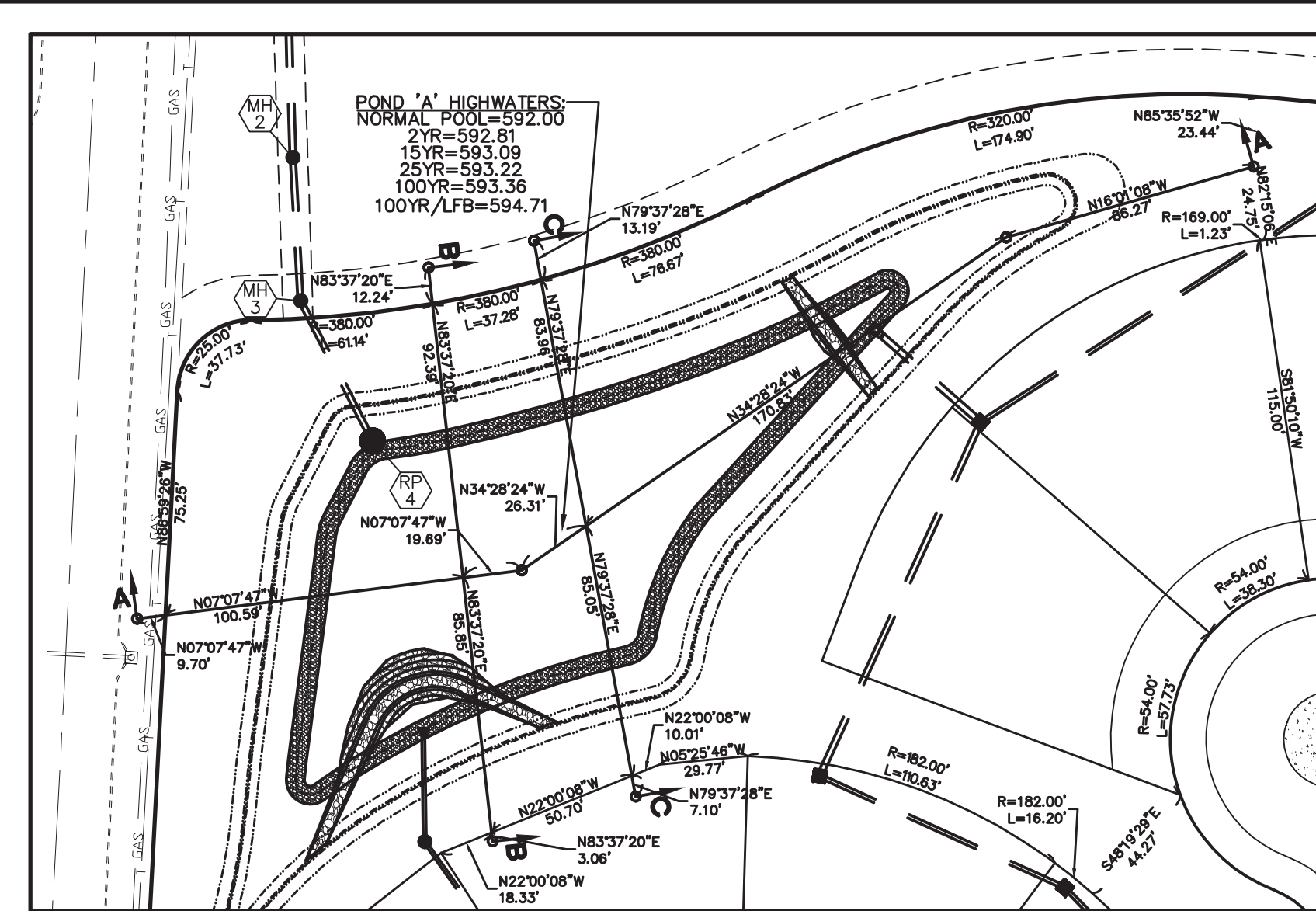
POND 'A' SECTION DETAIL
