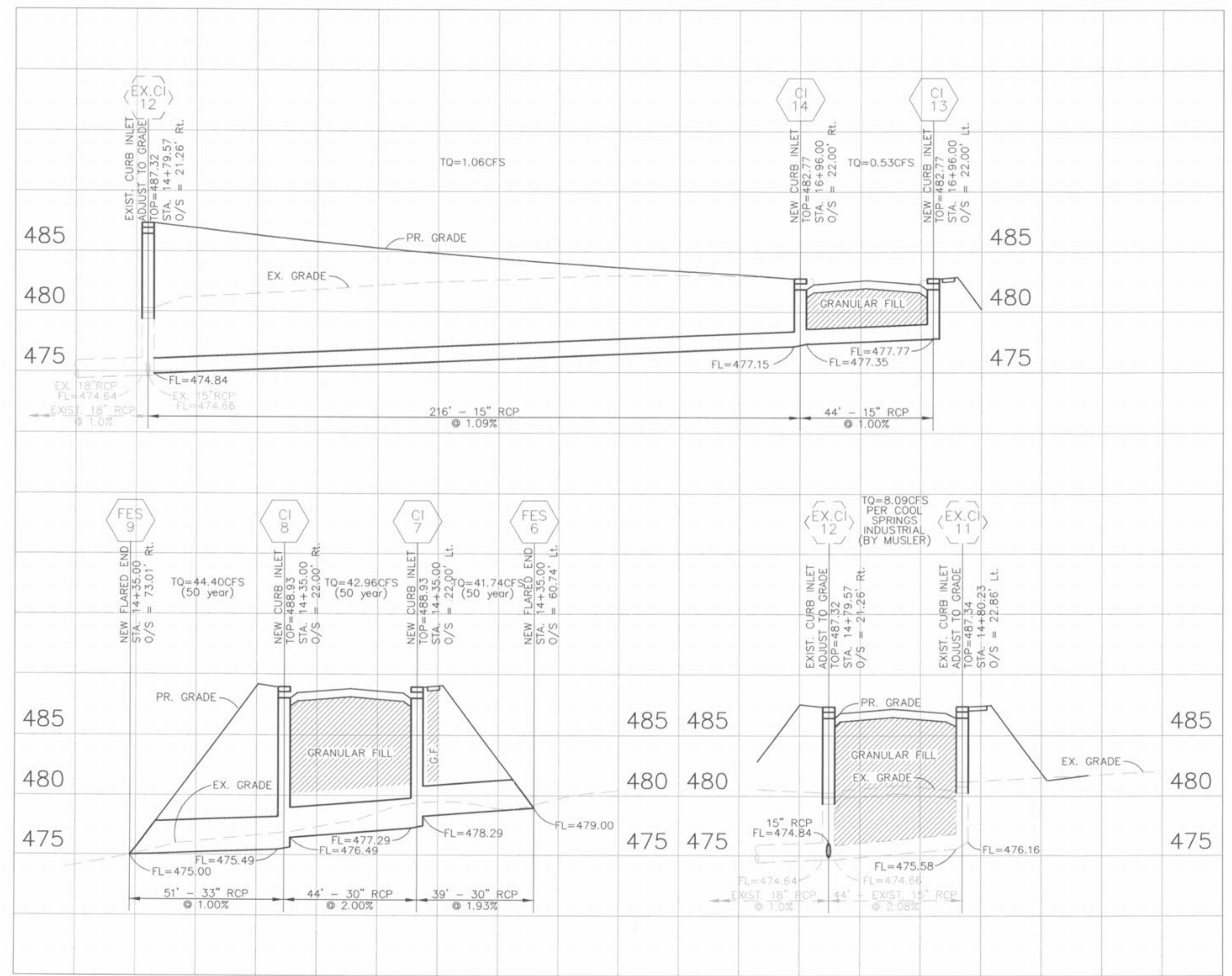
STORM SEWER PROFILE
