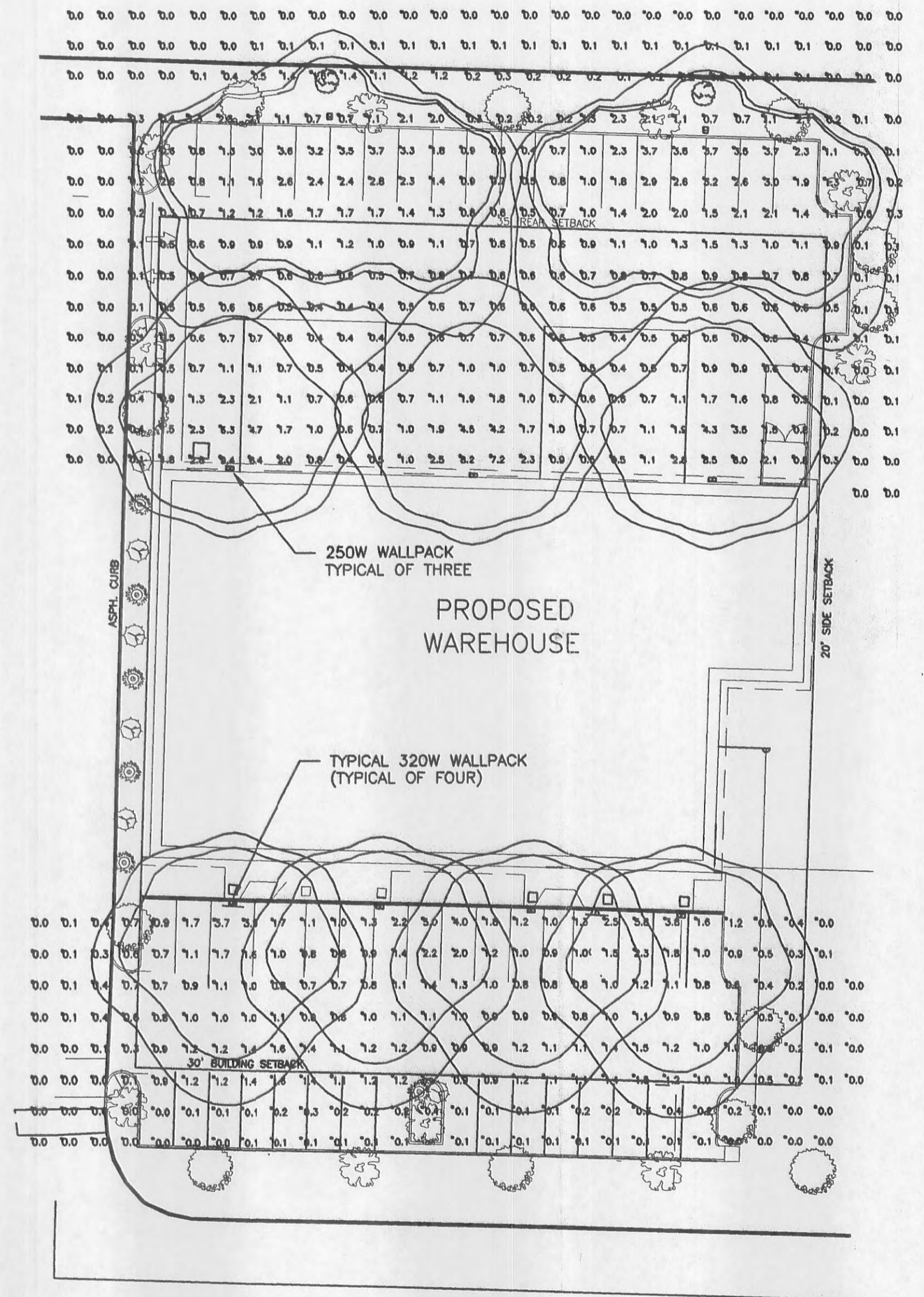
1 SITE LIGHTING PLAN & PHOTOMETRICS E2.0 1"=30'-0"
