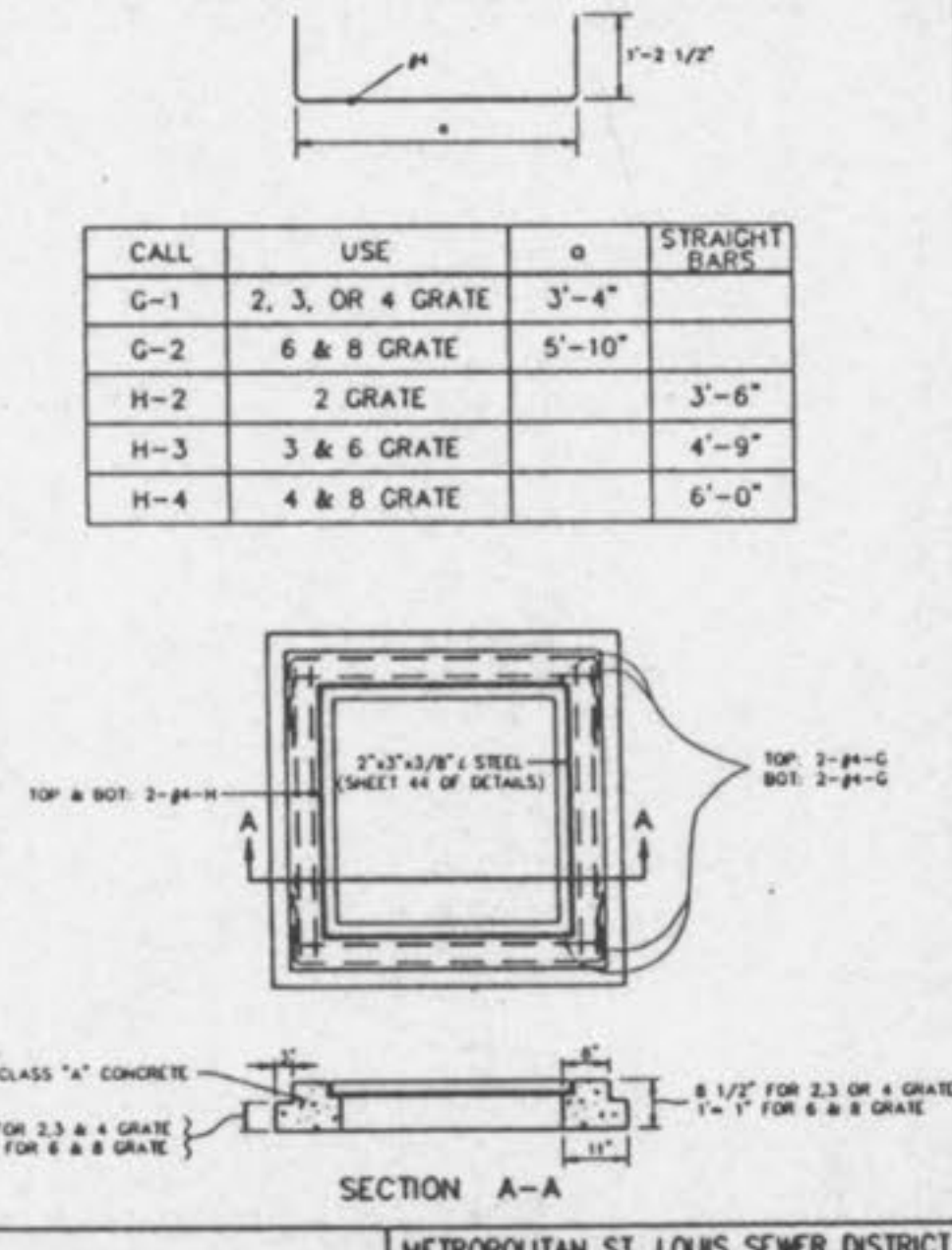
STEEL REQUIREMENTS FOR GRATE INLET SEAT METROPOLITAN ST. LOUIS SEWER DISTRICT Standard Details of Sewer Construction Dr. W.S.H. Ch. J.C.P. 1992 SHEET 46
