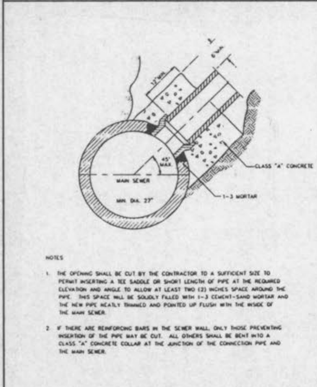
HOUSE CONNECTIONS ALLOWED BY TEE SADDLE METROPOLITAN ST. LOUIS SEWER DISTRICT Standard Details of Sewer Construction Dr. D.A.B. J.C.K. 1992 SHEET 61
