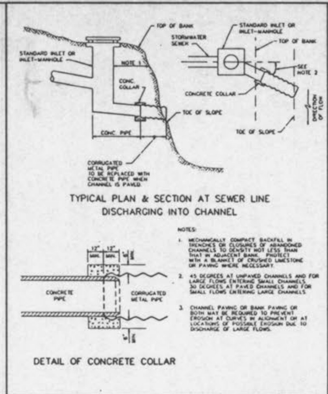
STORMWATER CHANNELS METROPOLITAN ST. LOUIS SEWER DISTRICT Standard Details of Sewer Construction Dr. R.C.W. J.C.K. 1992 SHEET 58
