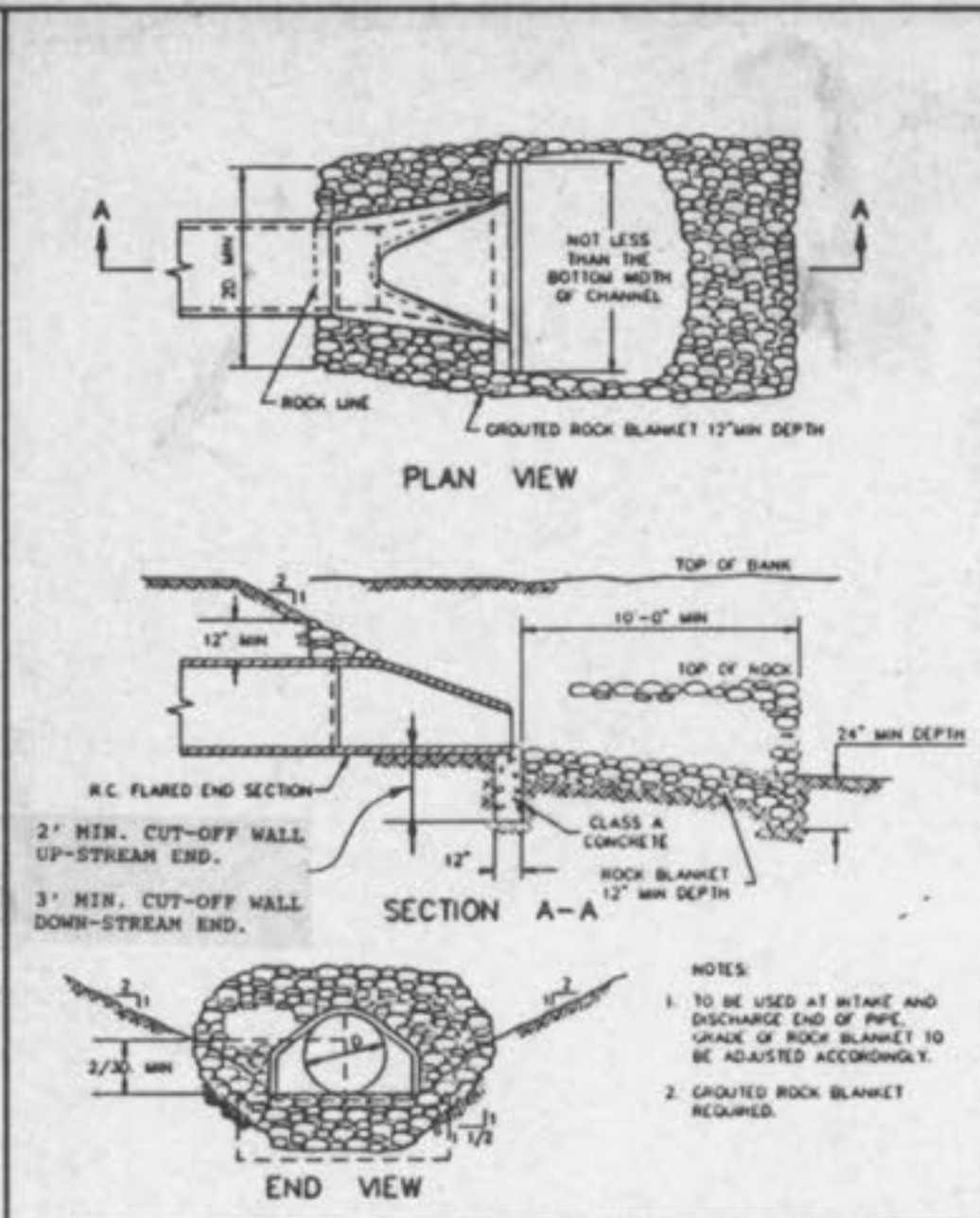
FLARED END SECTION METROPOLITAN ST. LOUIS SEWER DISTRICT Standard Details of Sewer Construction Dr. W.S.H. J.C.K. 1992 SHEET 57
