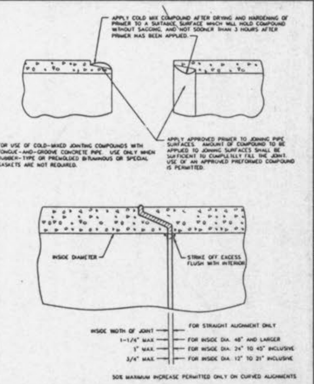
TONGUE AND GROOVE CONCRETE PIPE JOINTS METROPOLITAN ST. LOUIS SEWER DISTRICT Standard Details of Sewer Construction Dr. D.A.B. J.C.K. 1992 SHEET 66
