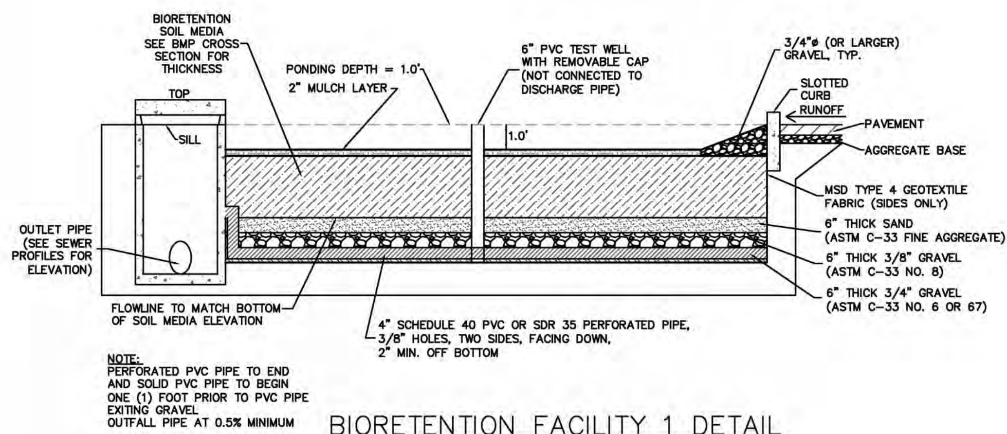
BIORETENTION FACILITY 1 DETAIL N.T.S.
