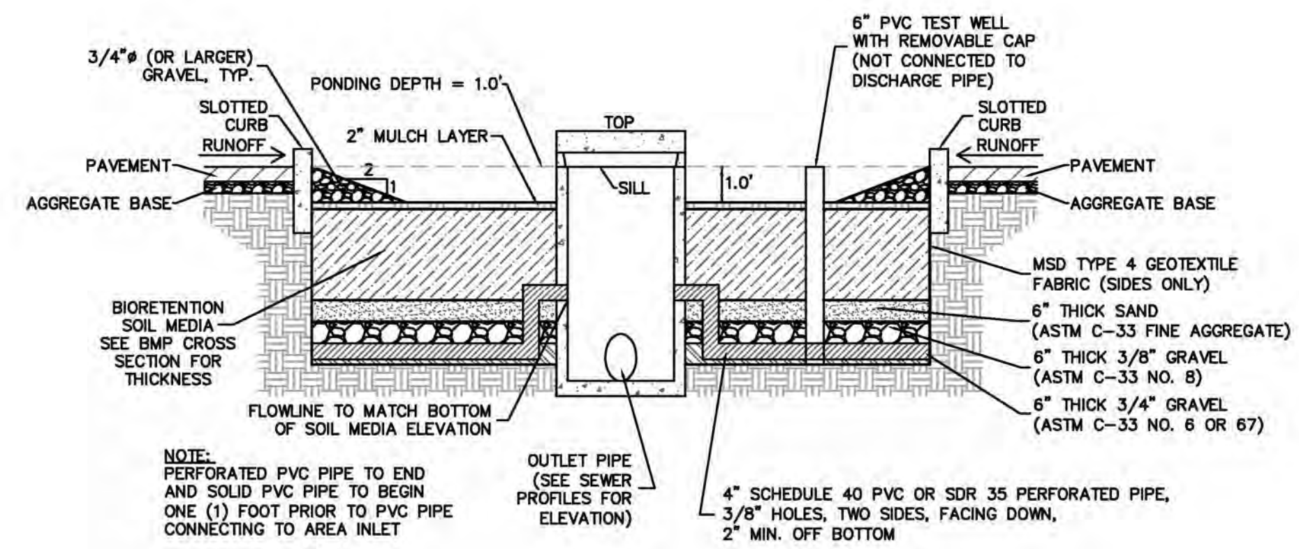
PARKING LOT BIORETENTION FACILITY 2 & 3 DETAIL N.T.S.
