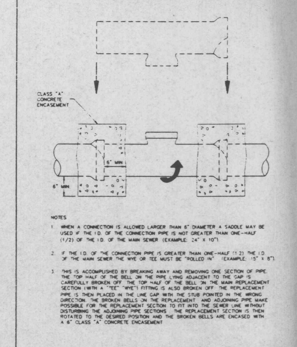
"ROLL-IN" (FOR EXISTING CLAY OR CONCRETE PIPE) METROPOLITAN ST. LOUIS SEWER DISTRICT Standard Details of Sewer Construction Dr. D.A.B. Ch. J.C.K. 1992 SHEET 63
