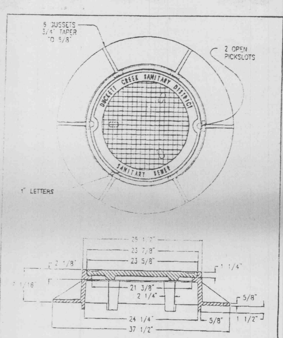
MANHOLE RING & COVER DUCKETT CREEK SANITARY DISTRICT STANDARD CONSTRUCTION DETAIL DETAIL NO. MAY 1998
