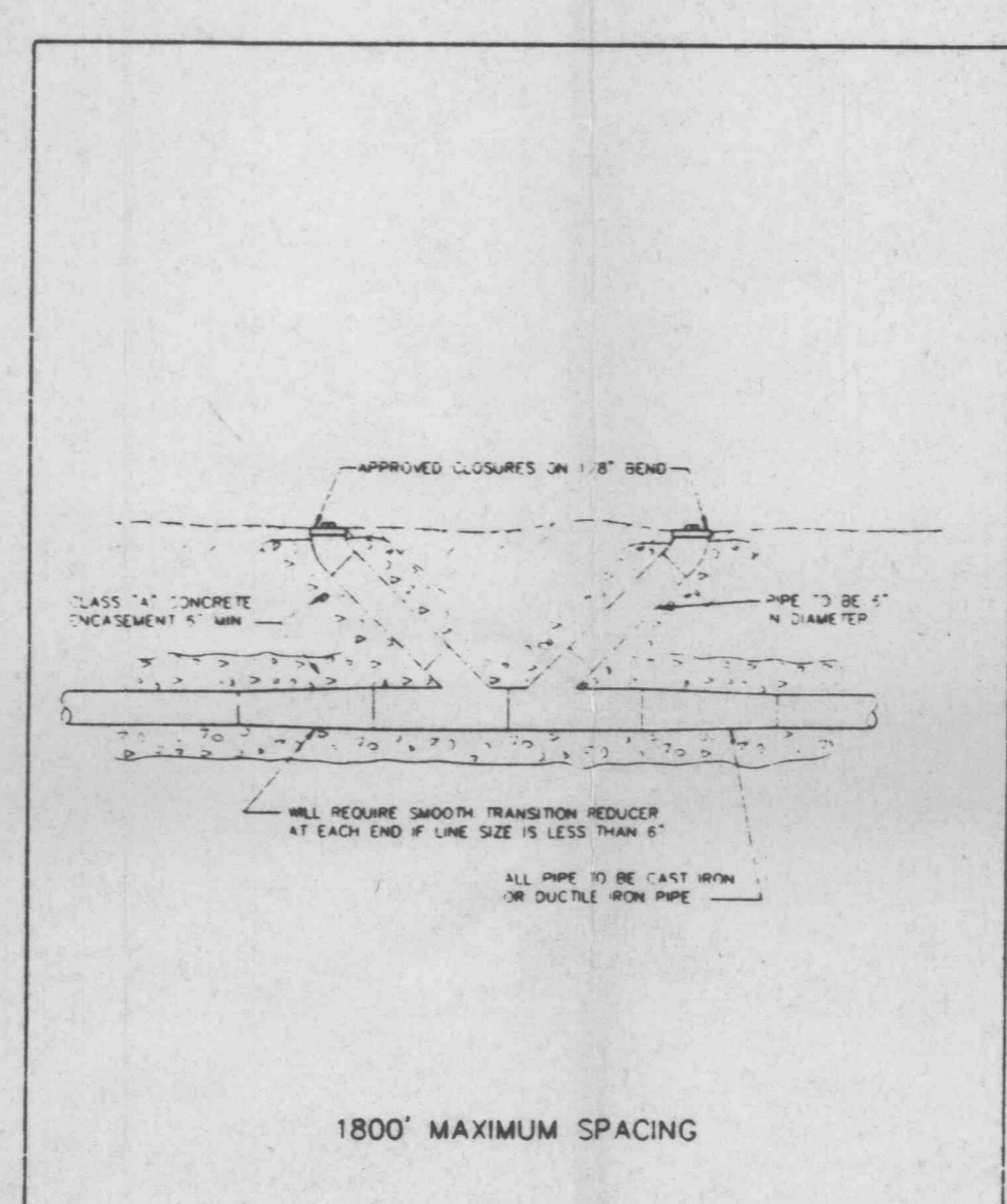
FORCE MAIN CLEANOUT (6" DIA. & SMALLER) METROPOLITAN ST. LOUIS SEWER DISTRICT Standard Details of Sewer Construction Dr. R.G.W. Ch. J.C.K. 1992 SHEET 55
