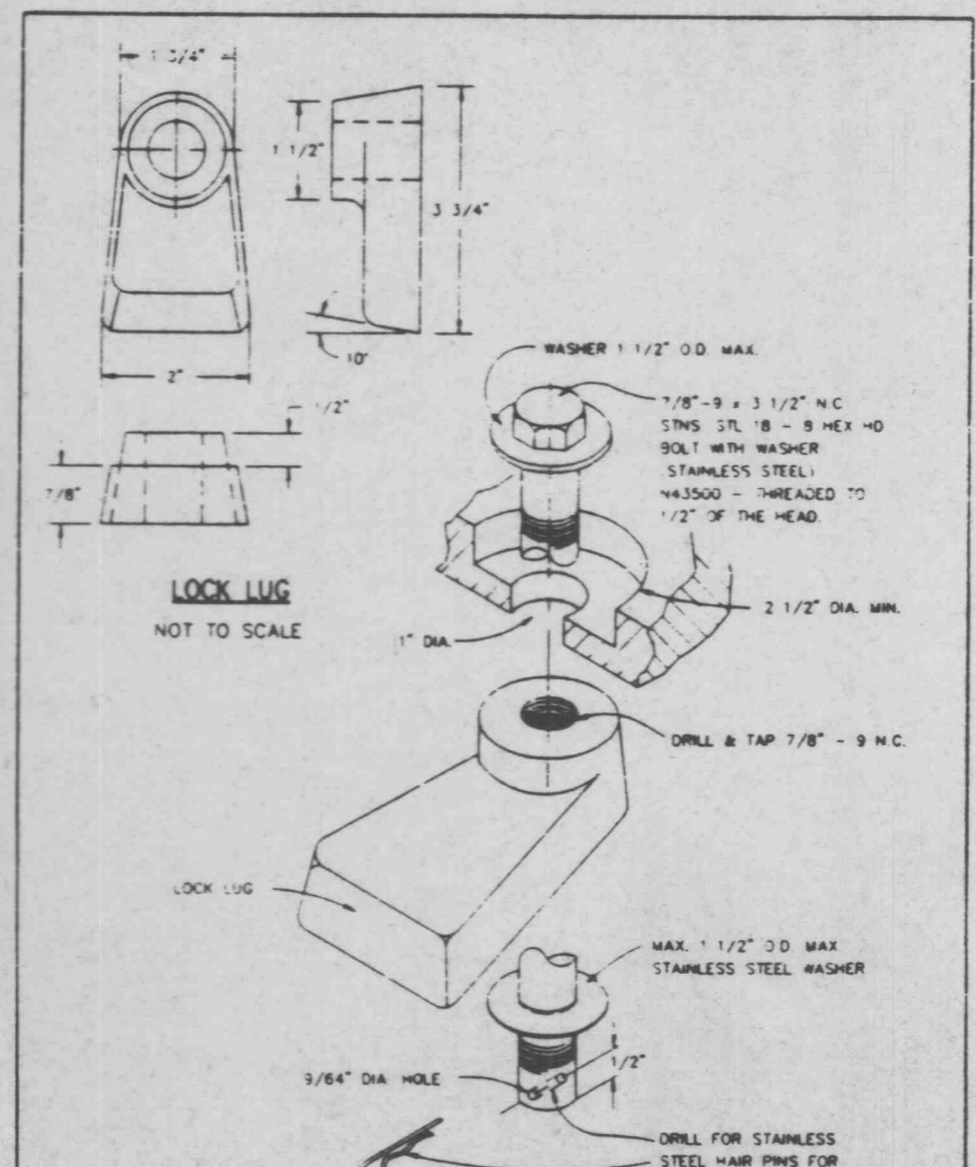
LOCKING DEVICE FOR TYPE 'N' LOCK TYPE MANHOLE COVER METROPOLITAN ST. LOUIS SEWER DISTRICT Standard Details of Sewer Construction Dr. W.S.H. Ch. J.C.K. 1992 SHEET 52
