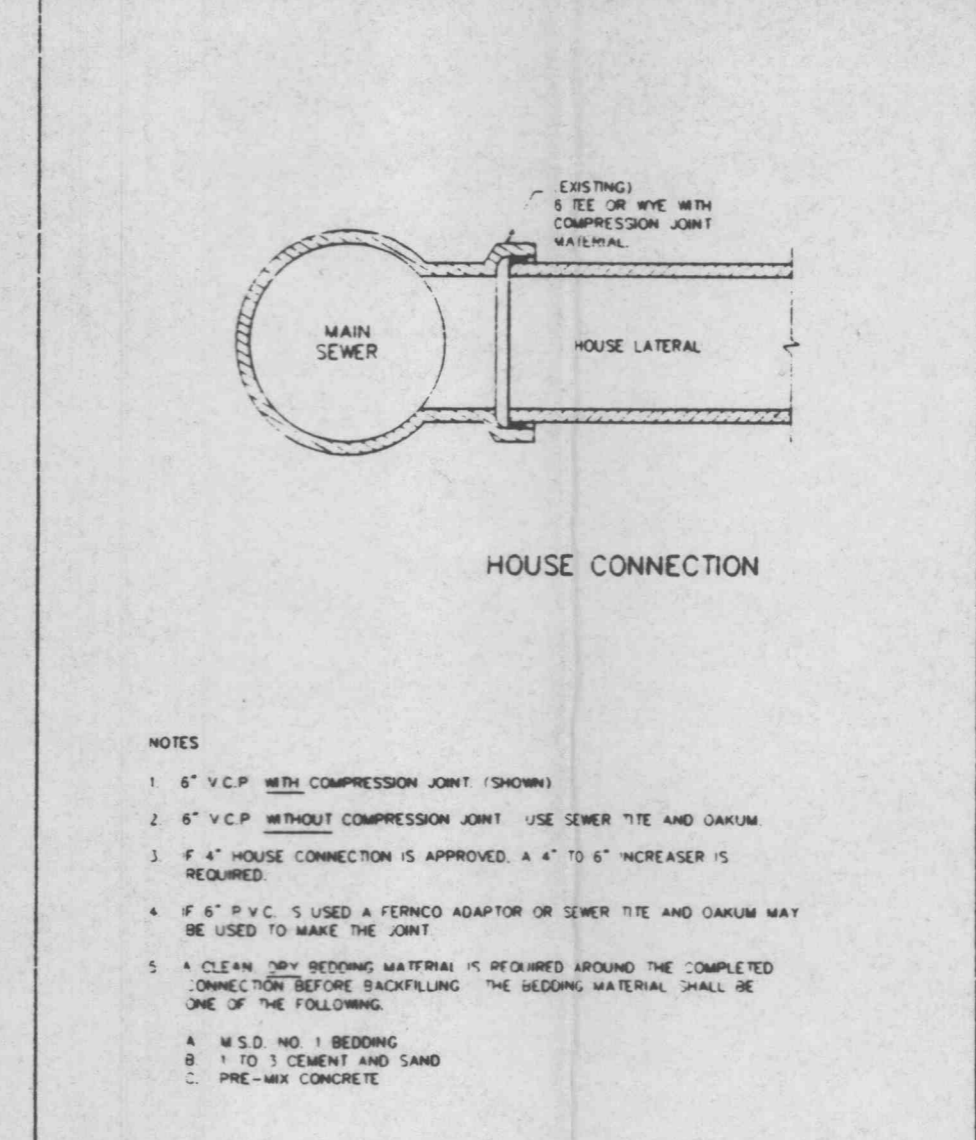
HOUSE CONNECTION TO EXISTING TEE OR WYE METROPOLITAN ST. LOUIS SEWER DISTRICT Standard Details of Sewer Construction Dr. D.A.B. Ch. J.C.K. 1992 SHEET 59
