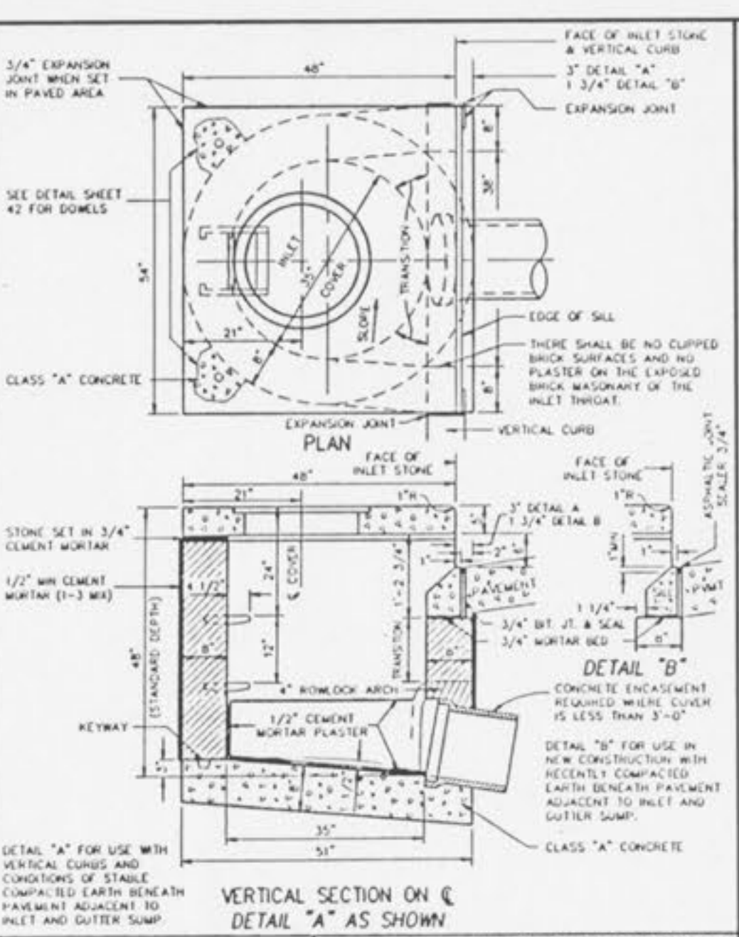
UNTRAPPED STREET INLET BRICK CONSTRUCTION METROPOLITAN ST. LOUIS SEWER DISTRICT Standard Details of Sewer Construction Dr. W.S.H. Ch. J.C.K. 1992 SHEET 20
