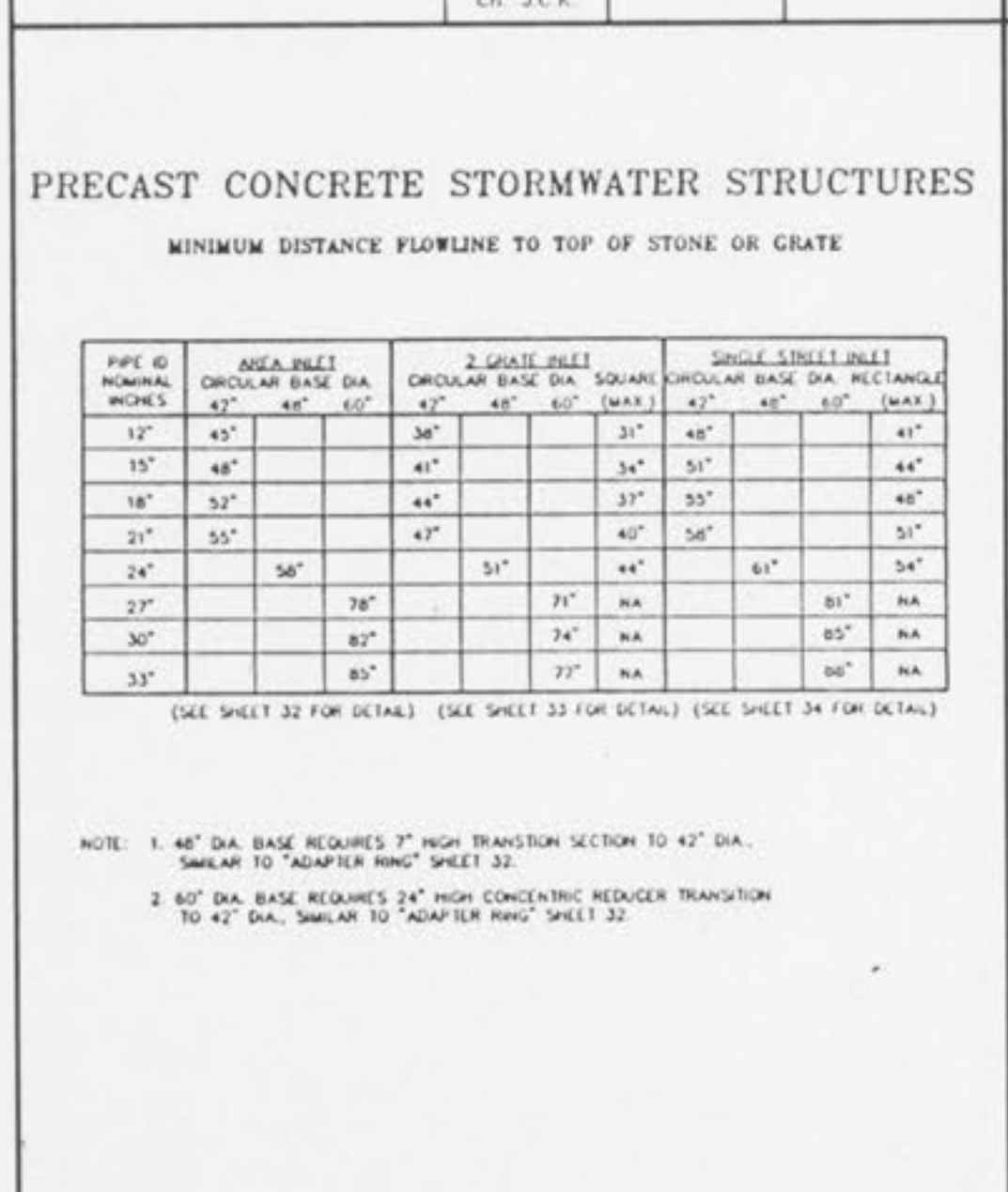
PRECAST CONCRETE STORMWATER STRUCTURES METROPOLITAN ST. LOUIS SEWER DISTRICT Standard Details of Sewer Construction Dr. J.L.G. Ch. J.C.K. SEPT. 1990 SHEET 31
