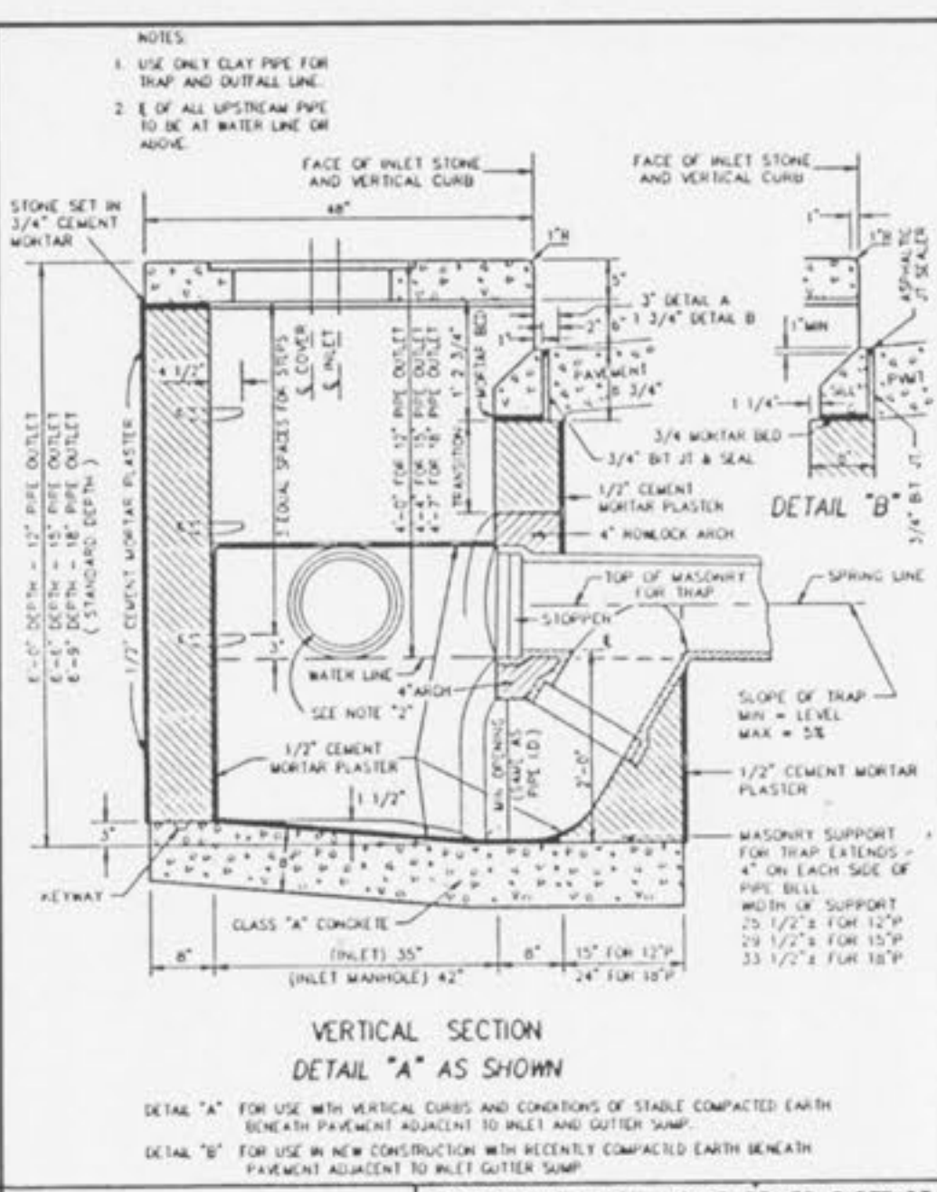
TRAPPED STREET INLET BRICK CONSTRUCTION METROPOLITAN ST. LOUIS SEWER DISTRICT Standard Details of Sewer Construction Dr. W.S.H. Ch. J.C.K. 1992 SHEET 21
