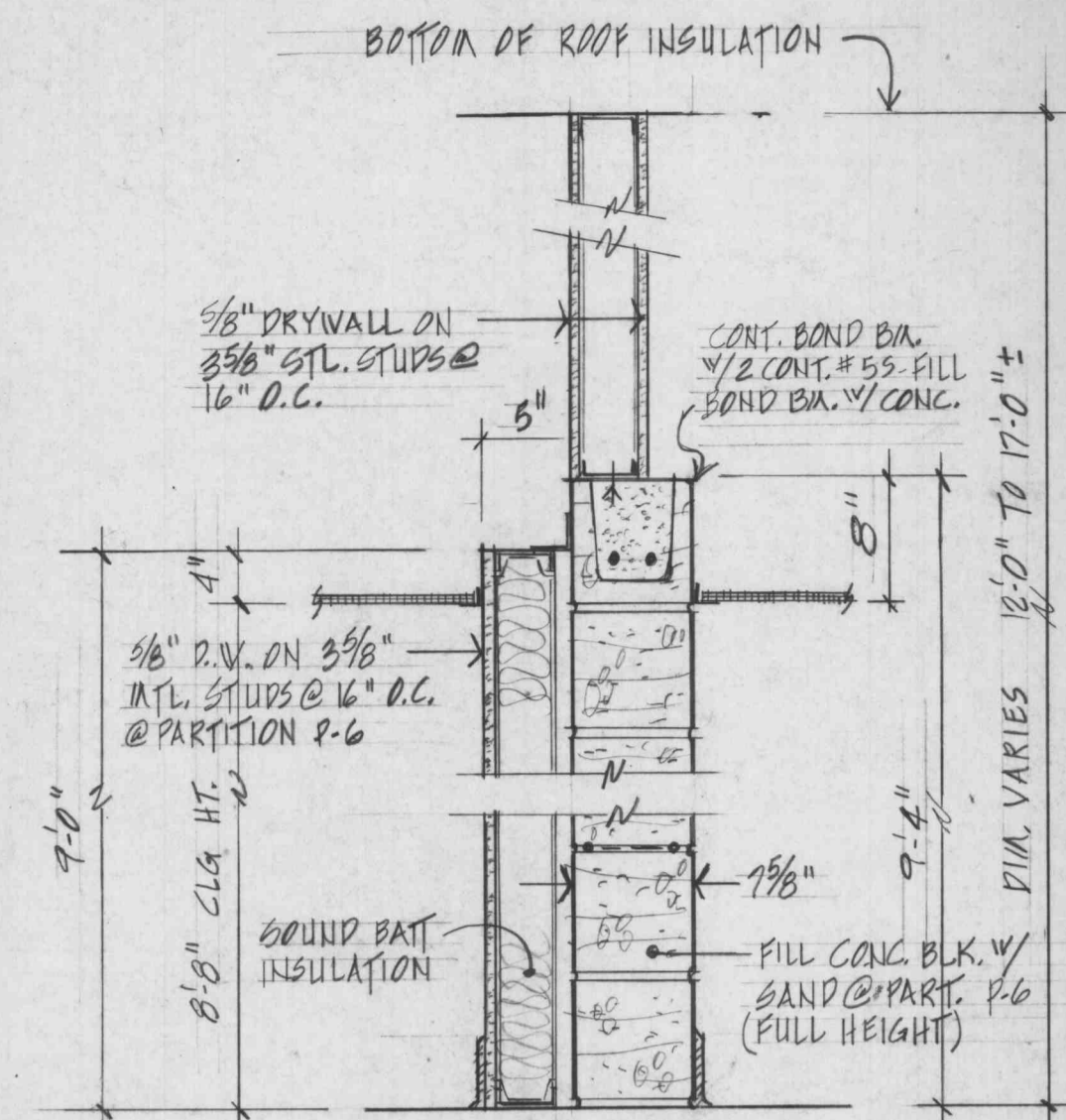
PARTITIONS P6 P7 SCALE 1" = 1'-0"
