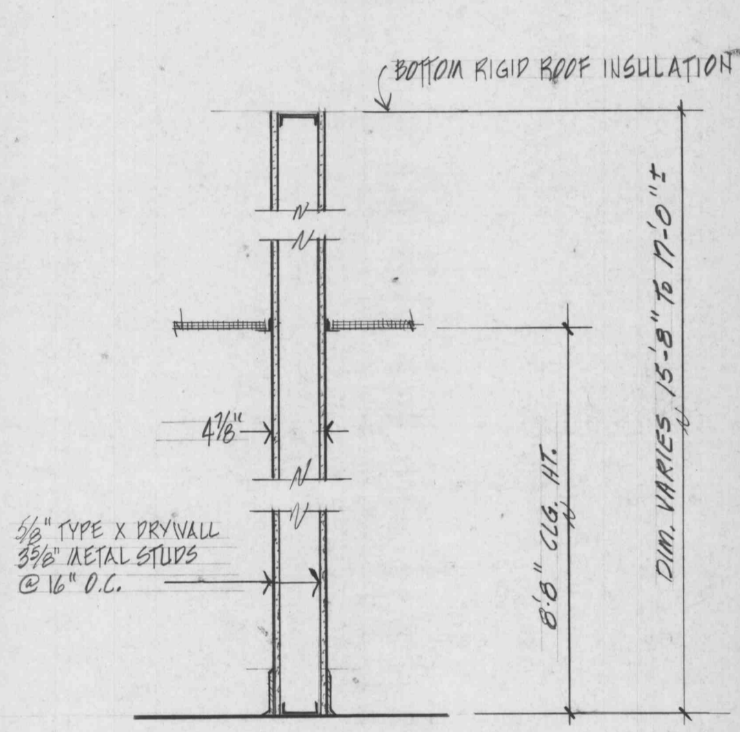
PARTITIONS P6 P7 SCALE 1" = 1'-0"
