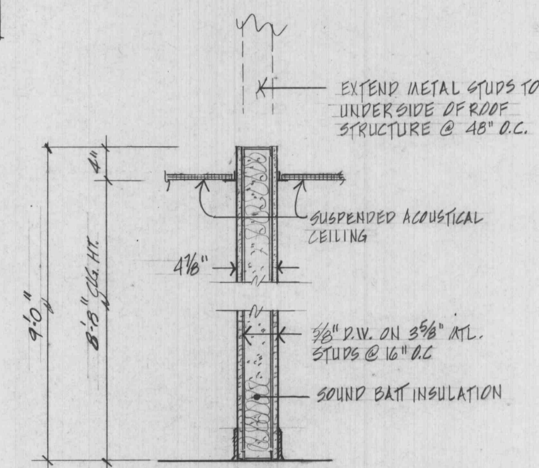
PARTITION P8 SCALE 1" = 1'-0"
