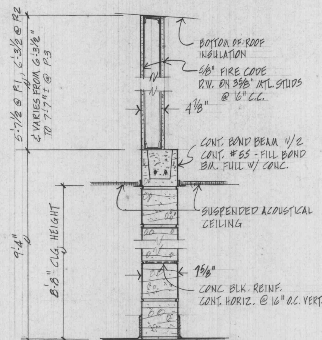
PARTITIONS P1 P2 P3 SCALE 1" = 1'-0"
