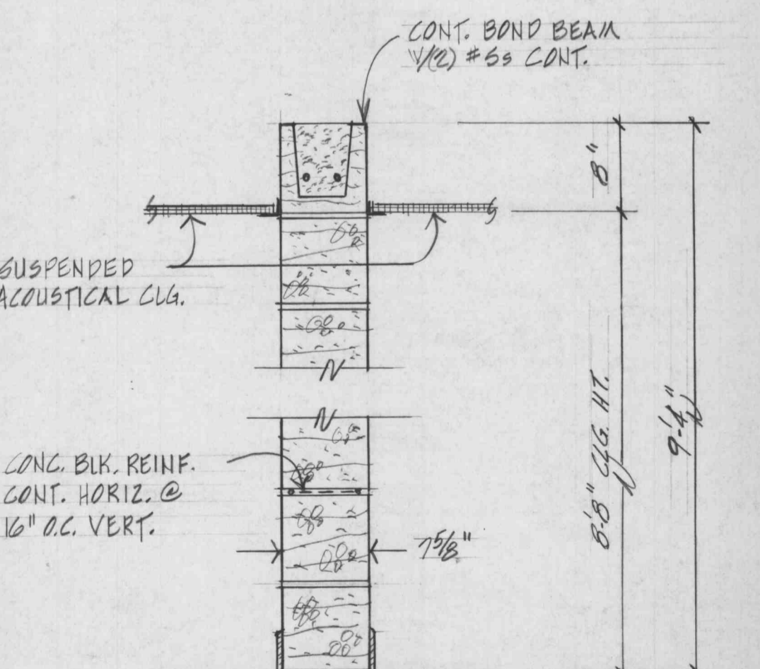
PARTITION P10 SCALE 1" = 1'-0"
