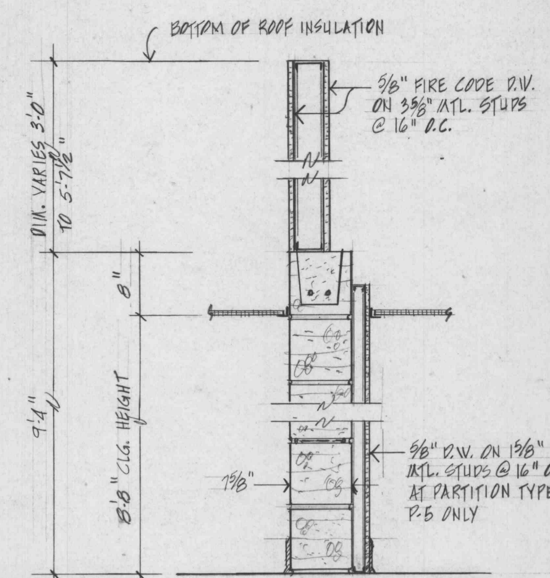
PARTITIONS P4 P5 SCALE 1" = 1'-0"
