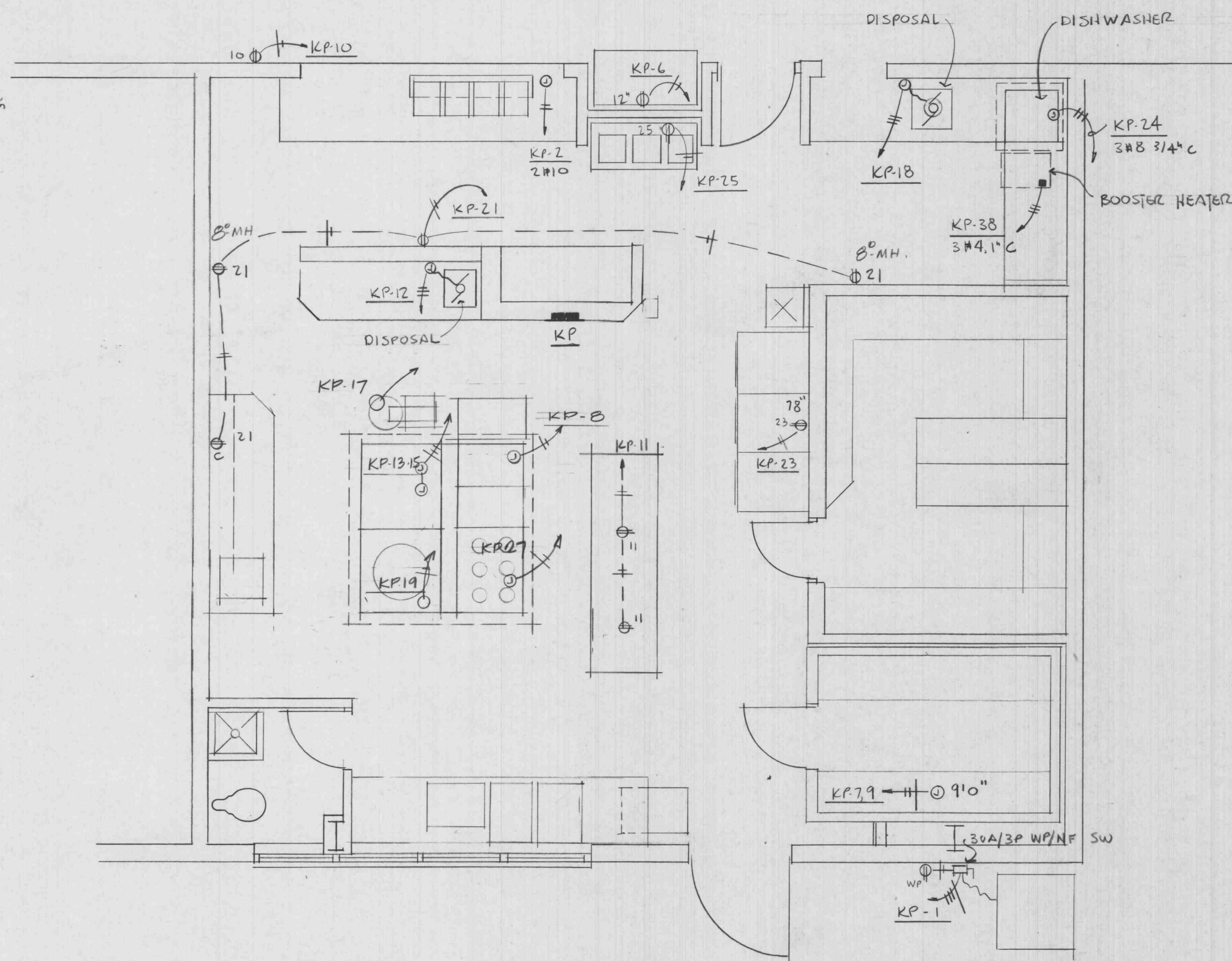
KITCHEN PLAN SCALE: 1/4" = 1'-0"
