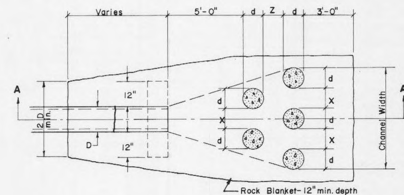
PLAN VIEW
