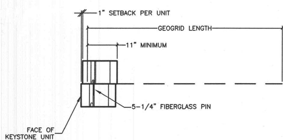
CONNECTION DETAIL NOT TO SCALE
