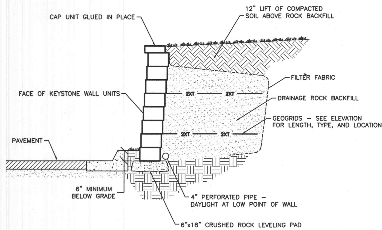
TYPICAL SECTION WALL A NOT TO SCALE
