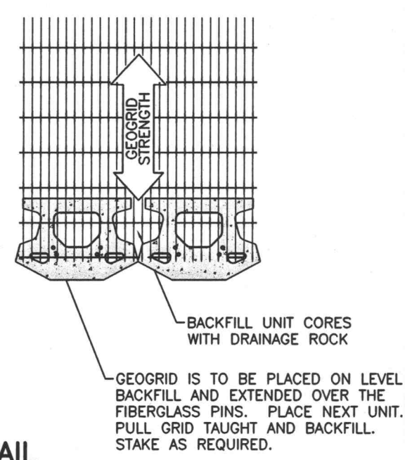
COMPAC II UNIT NOT TO SCALE
