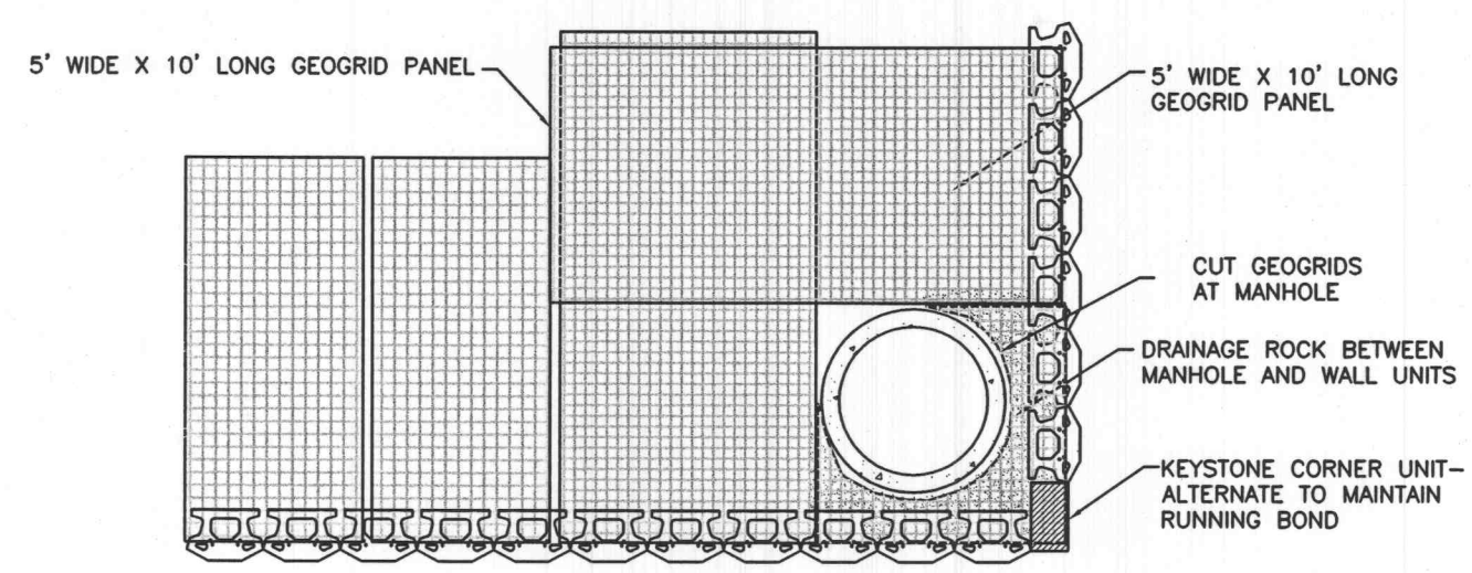
MANHOLE DETAIL NOT TO SCALE
