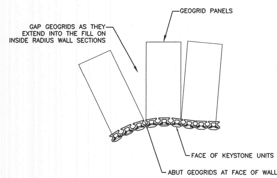
INSIDE RADIUS DETAIL NOT TO SCALE
