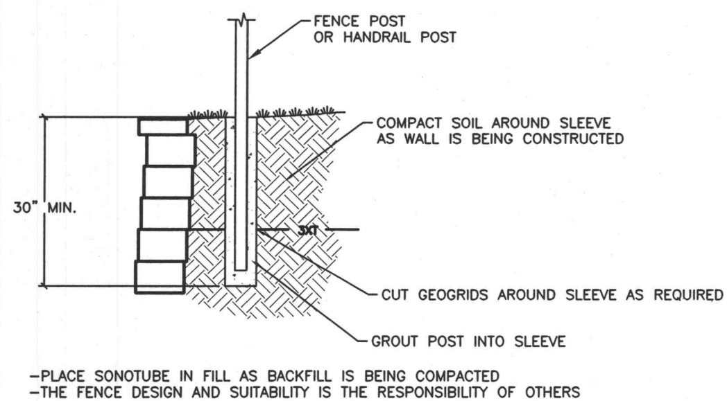
FENCE DETAIL NOT TO SCALE
