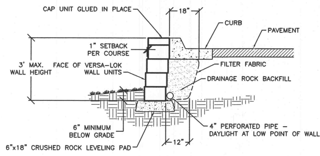
UNREINFORCED SECTION NOT TO SCALE
