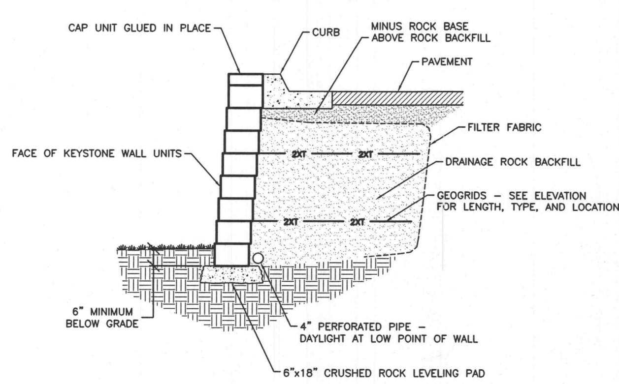
TYPICAL SECTION WALL B & C NOT TO SCALE
