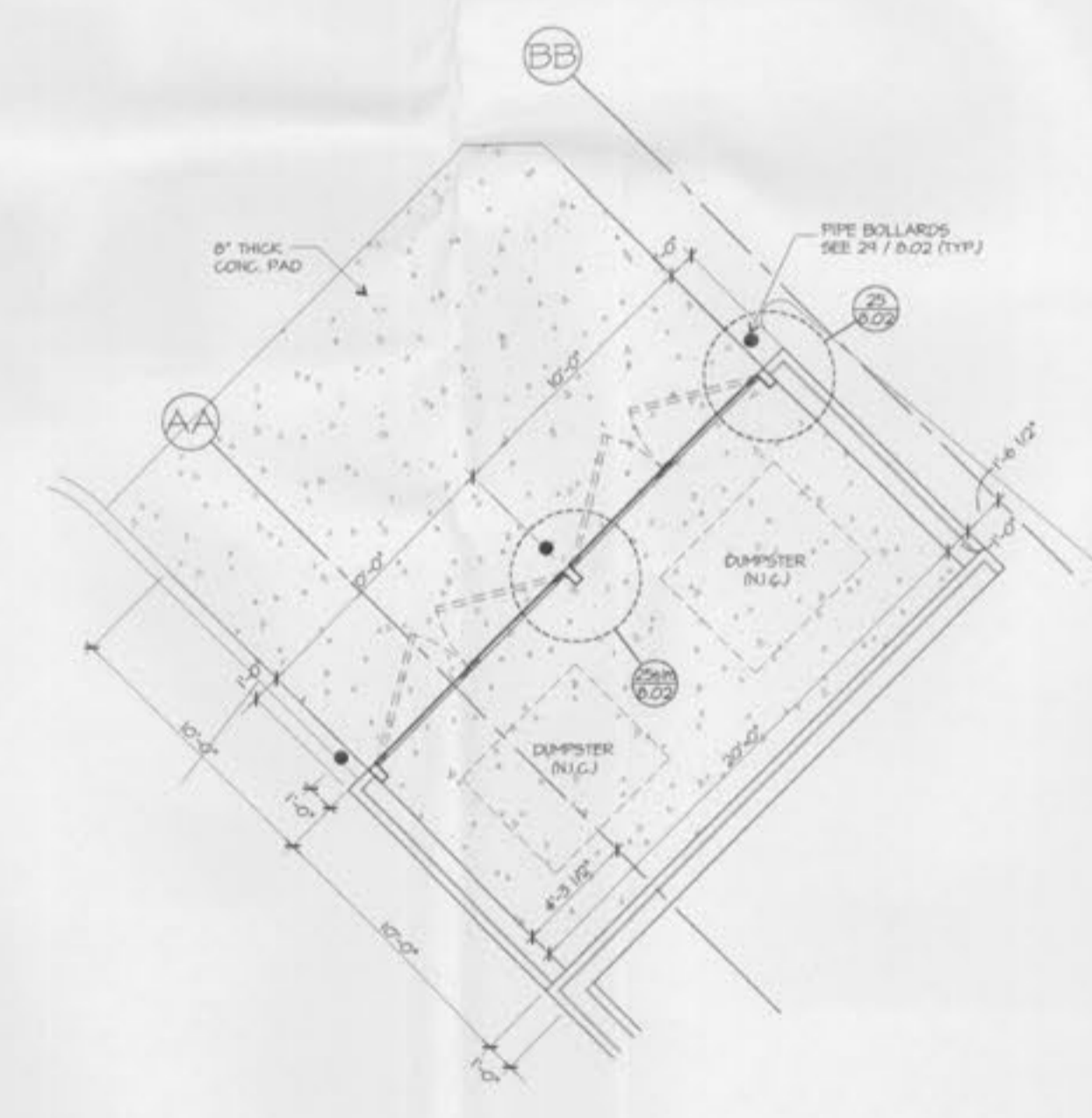
25 DUMPSTER ENCLOSURE SCALE: 1/4" = 1'-0"
