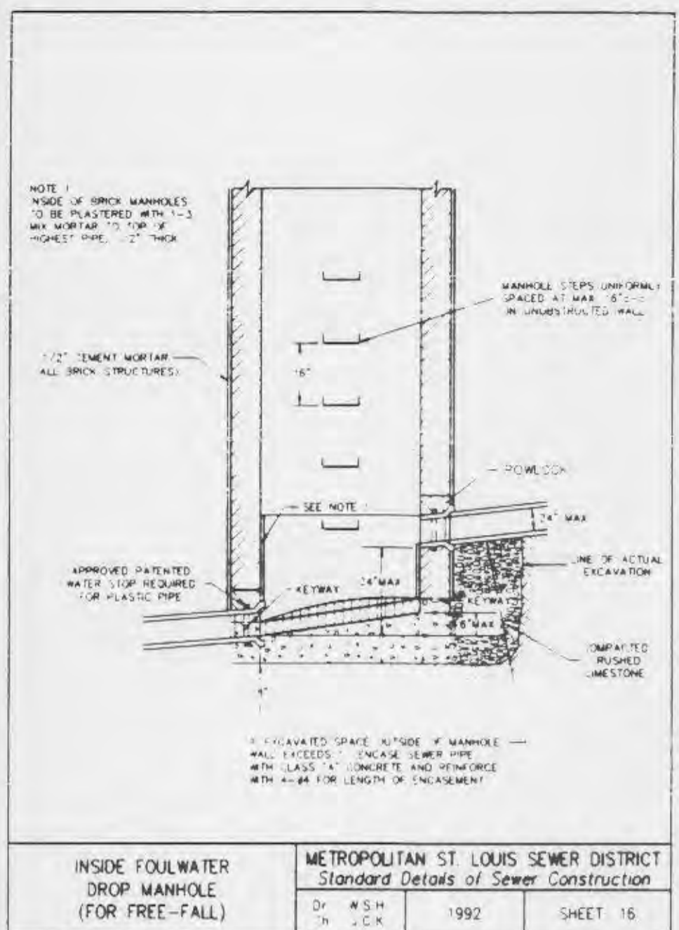
INSIDE FOULWATER DROP MANHOLE METROPOLITAN ST. LOUIS SEWER DISTRICT Standard Details of Sewer Construction 1992 SHEET 15
