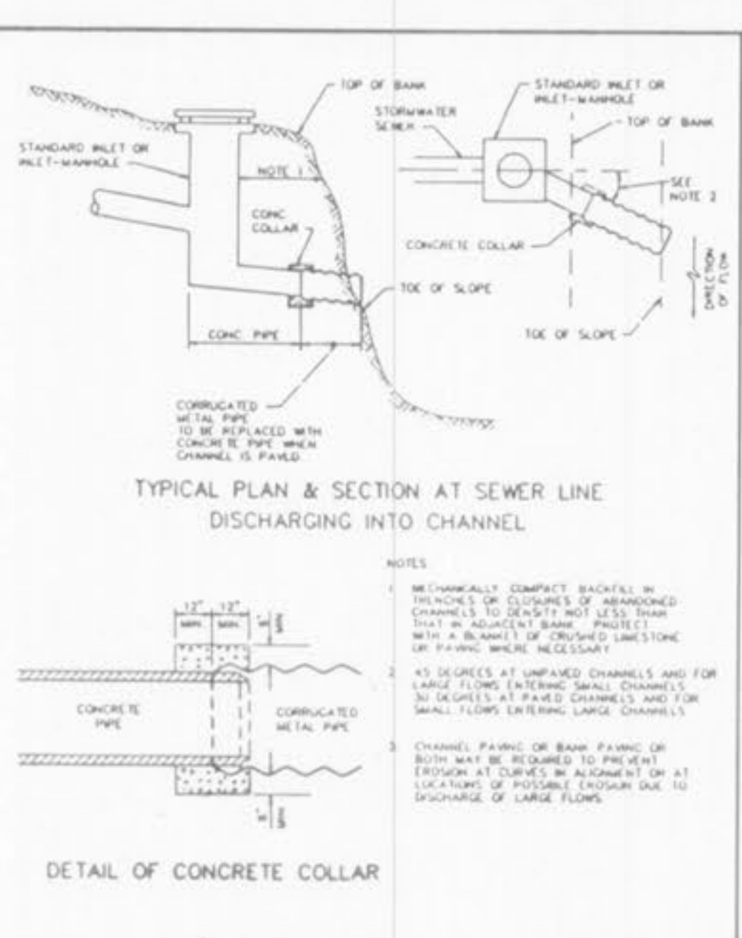
STORMWATER CHANNELS METROPOLITAN ST. LOUIS SEWER DISTRICT Standard Details of Sewer Construction Dr. R.C.W. Ch. J.C.K. 1992 SHEET 58
