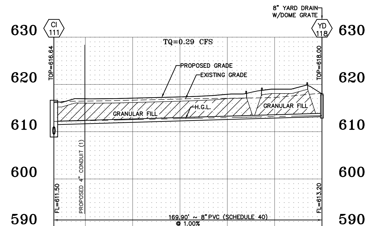
(PRIVATE) Storm Sewer Profile HORIZONTAL SCALE: 1" = 30' VERTICAL SCALE: 1" = 10' * STORM SEWERS MAY ALSO BE ADS N-12 OR EQUAL
