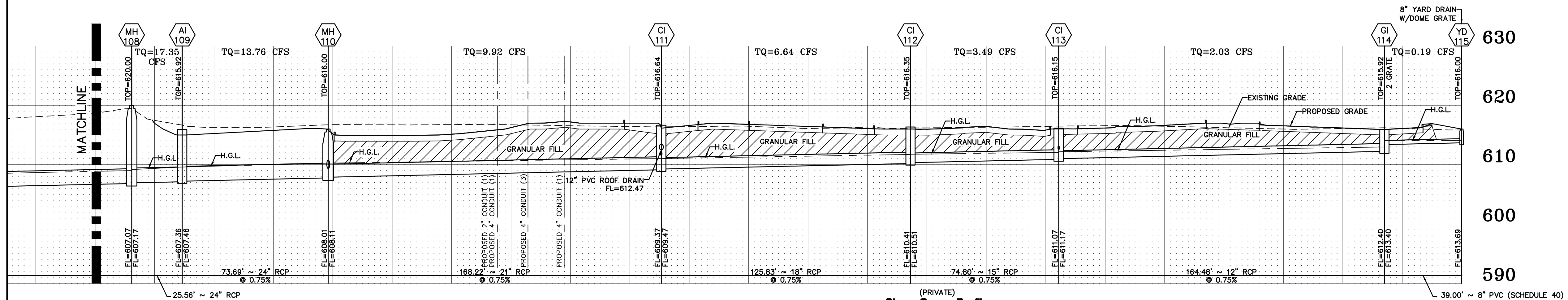
(PRIVATE) Storm Sewer Profile HORIZONTAL SCALE: 1" = 30' VERTICAL SCALE: 1" = 10' * STORM SEWERS MAY ALSO BE ADS N-12 OR EQUAL
