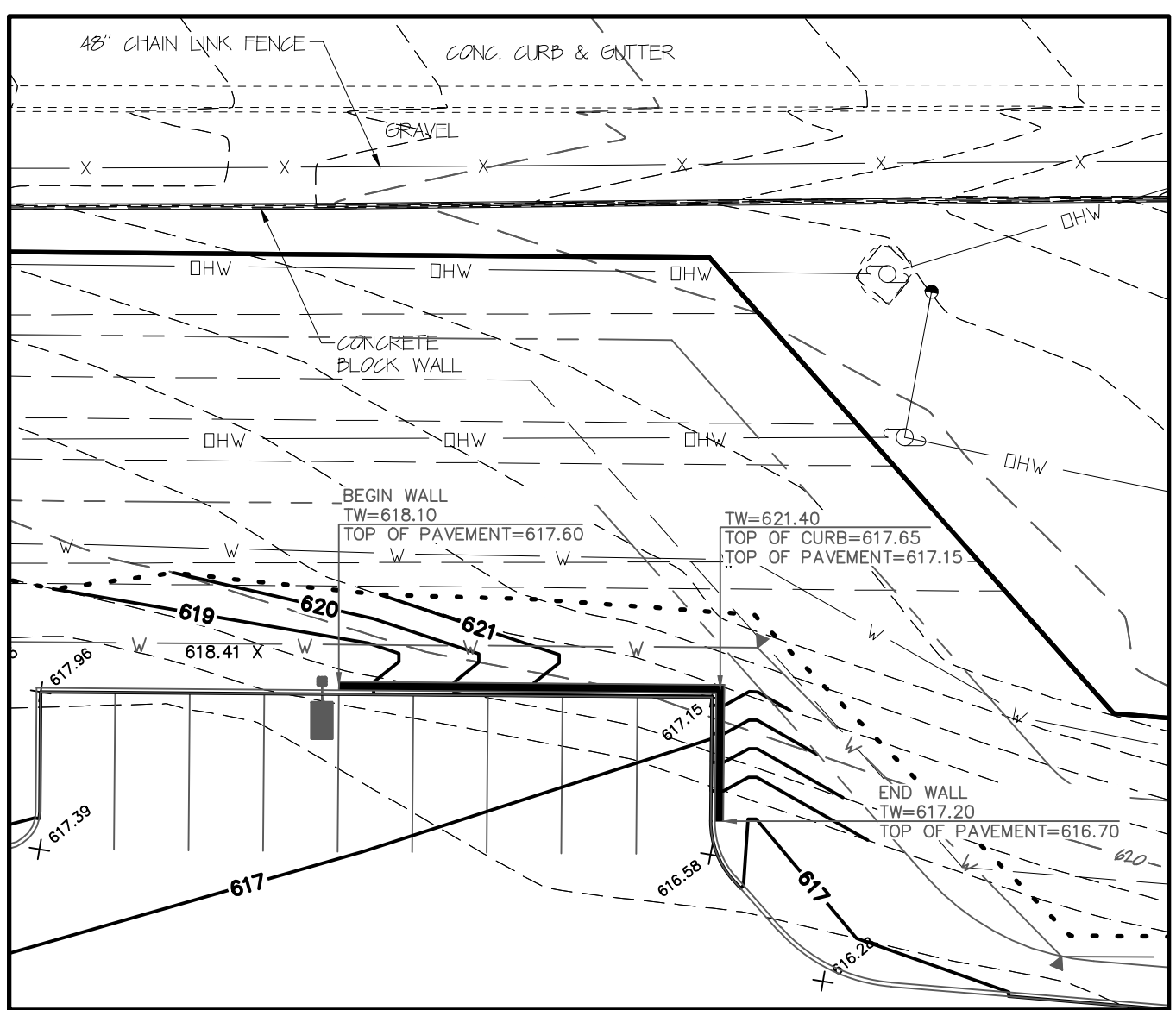
Modular Block Wall Detail SCALE: 1"=20'
