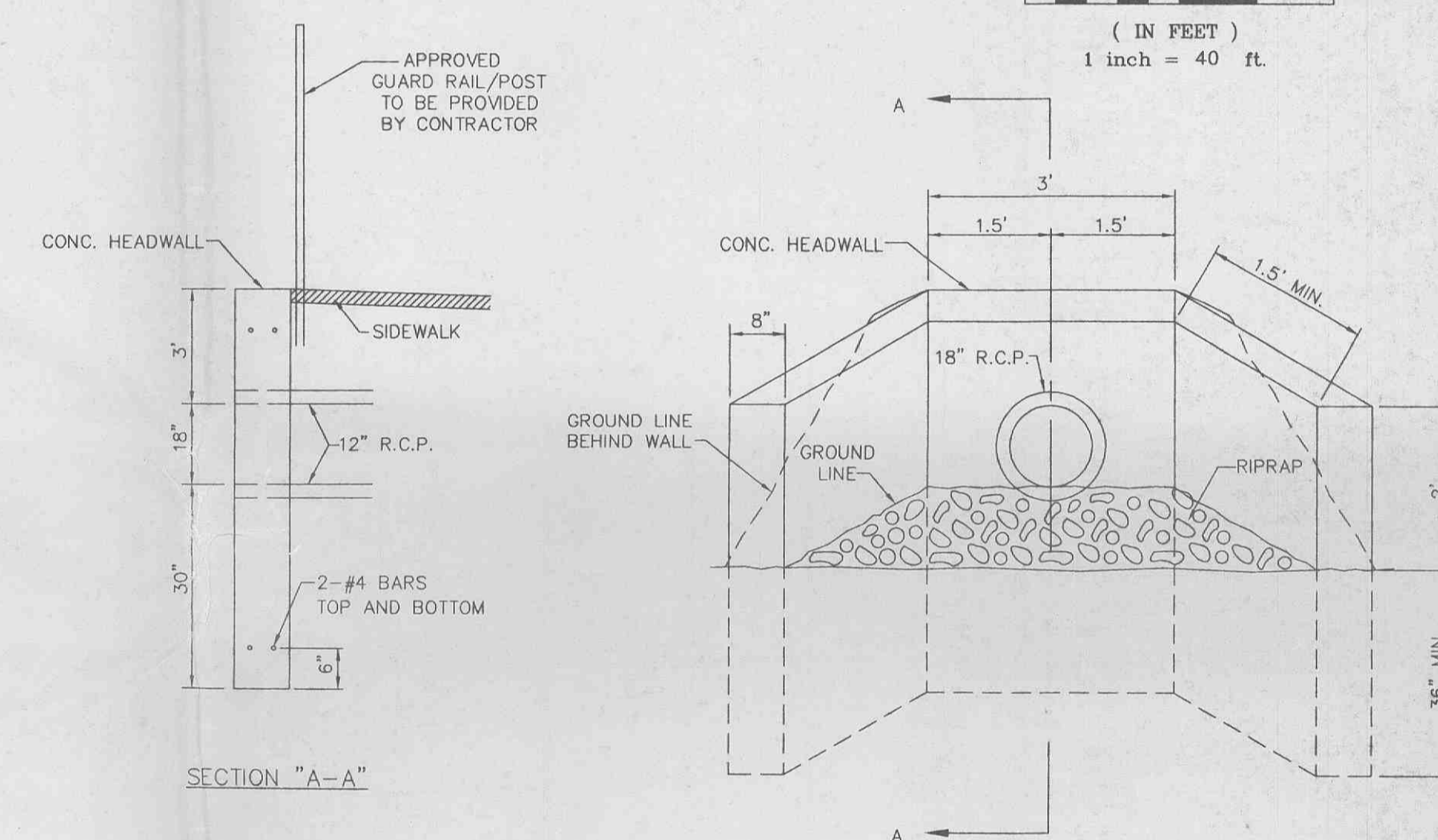
CONCRETE HEADWALL DETAIL NOT TO SCALE
