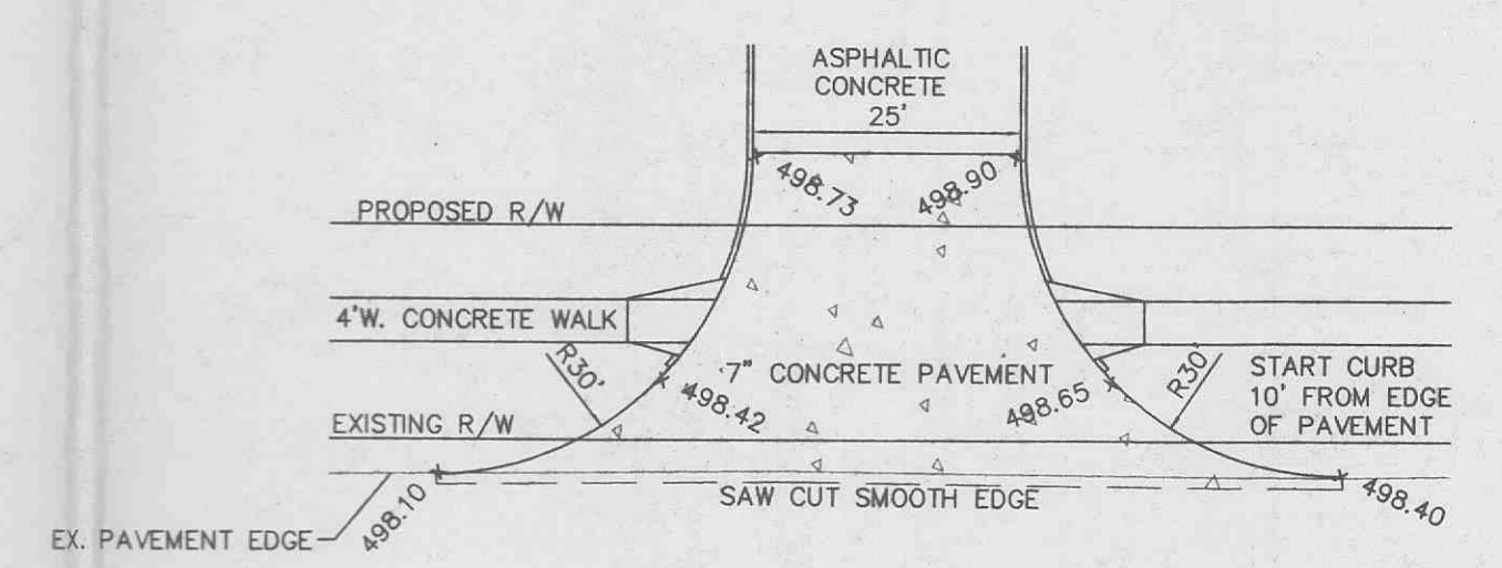
ENTRANCE DETAIL SCALE: 1" = 20'
