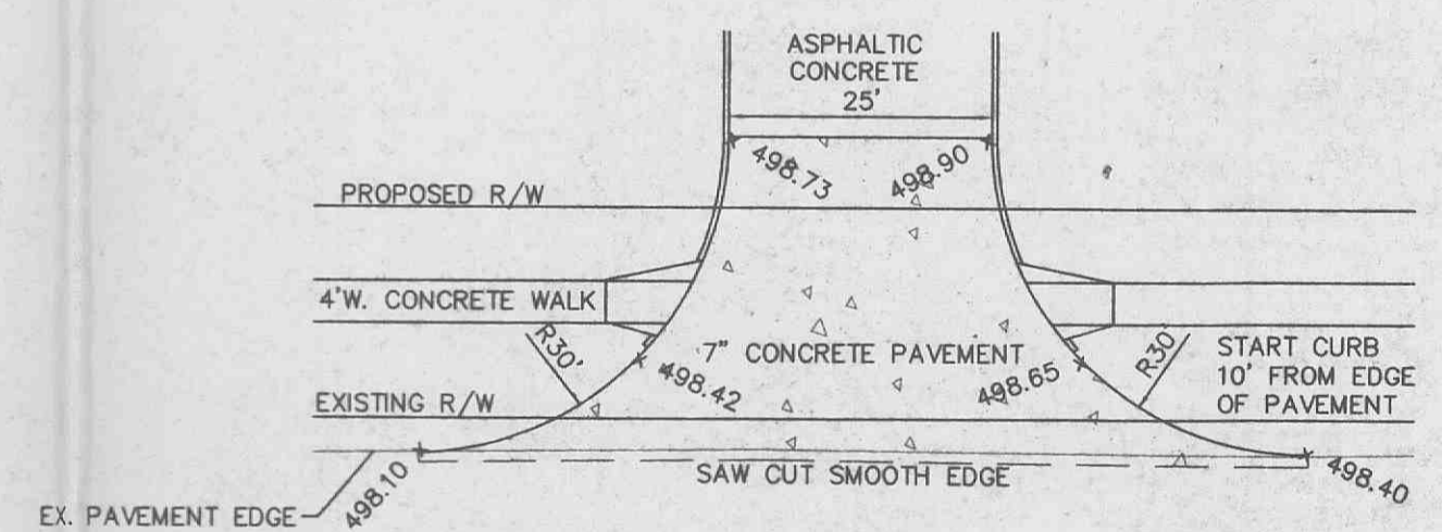
ENTRANCE DETAIL SCALE: 1" = 20'
