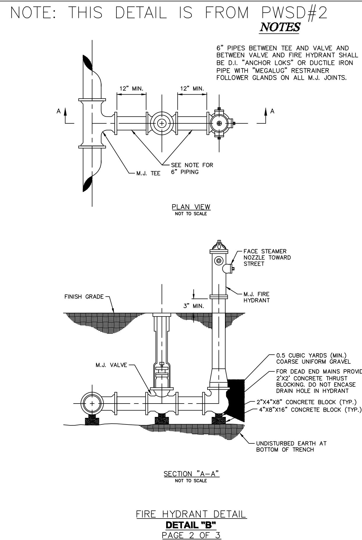
FIRE HYDRANT DETAIL DETAIL "B" PAGE 1 OF 3
