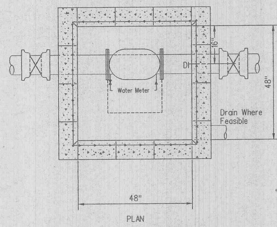
WATER METER BOX FOR 8" METER
