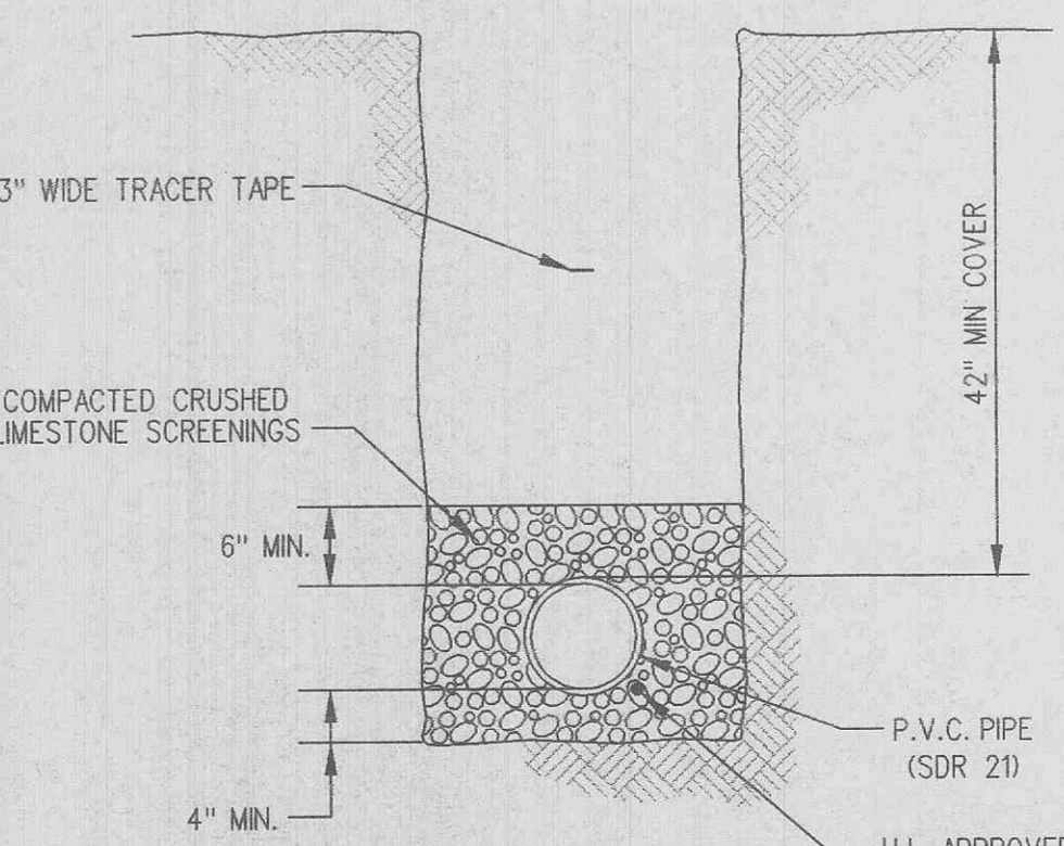
TRENCH DETAIL
