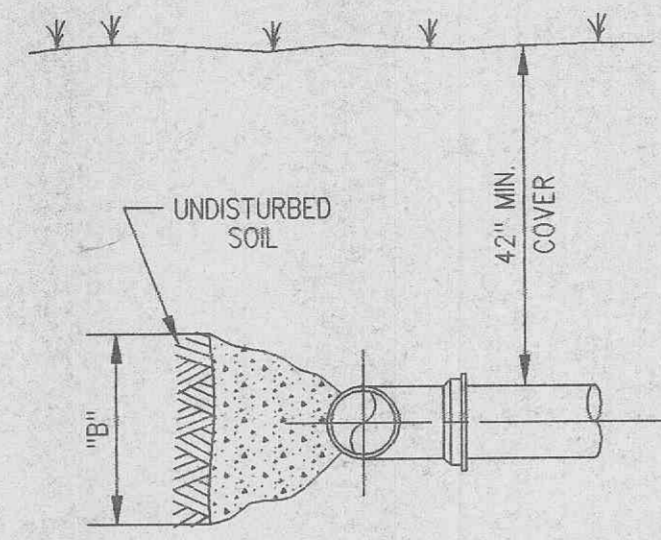
SECTION A-A (TYPICAL FOR ALL THRUST BLOCKS)
