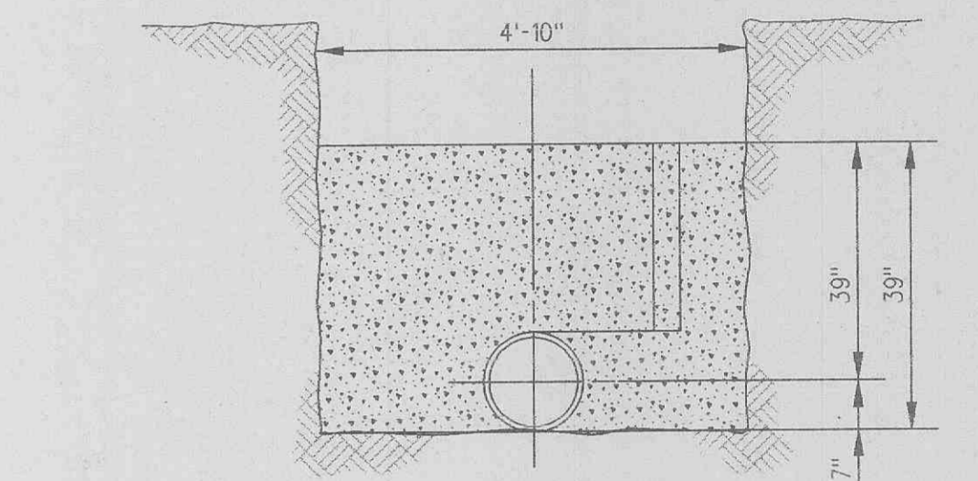
HORIZONTAL THRUST BLOCK DETAILS
