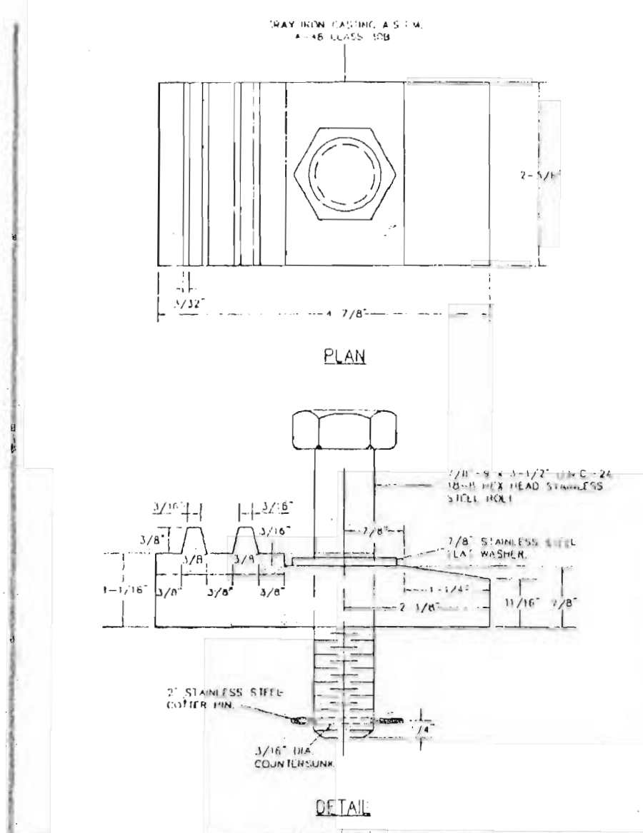
LOCKING DEVICE FOR TYPE "T" LOCK TYPE MANHOLE COVER METROPOLITAN ST. LOUIS SEWER DISTRICT Standard Details of Sewer Construction D. RW/SAM Ch. J.C.K. 2000 SHEET 55
