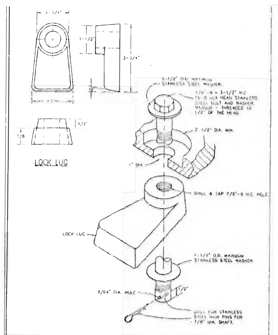
LOCKING DEVICE FOR TYPE "N" LOCK TYPE MANHOLE COVER METROPOLITAN ST. LOUIS SEWER DISTRICT Standard Details of Sewer Construction D. RW/SAM Ch. J.C.K. 2000 SHEET 56
