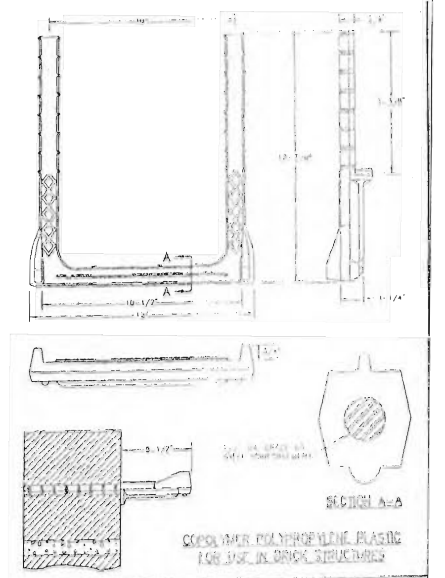
PSI-B MANHOLE STEP INTO JOINT METROPOLITAN ST. LOUIS SEWER DISTRICT Standard Details of Sewer Construction D. RW/SAM Ch. J.C.K. 2000 SHEET 57
