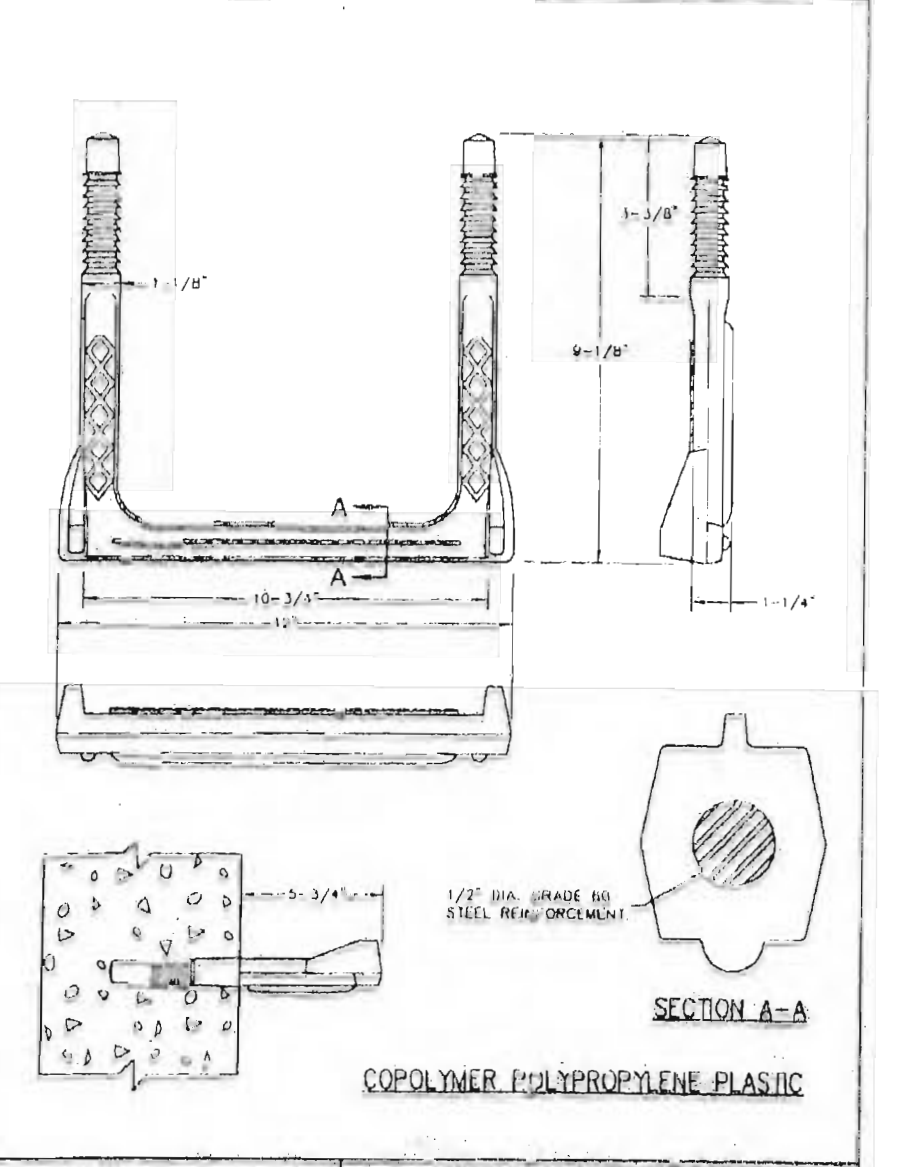
MANHOLE STEP FOR PRECAST & CAST-IN-PLACE MANHOLE METROPOLITAN ST. LOUIS SEWER DISTRICT Standard Details of Sewer Construction D. RW/SAM Ch. J.C.K. 2000 SHEET 58
