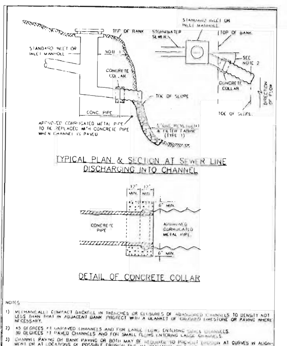
TYPICAL PLAN & SECTION AT SEWER LINE DISCHARGING INTO CHANNEL METROPOLITAN ST. LOUIS SEWER DISTRICT Standard Details of Sewer Construction D. RW/SAM Ch. J.C.K. 2000 SHEET 62
