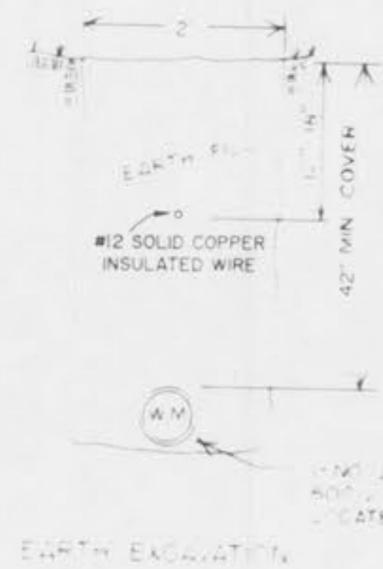
EARTH EXCAVATION
