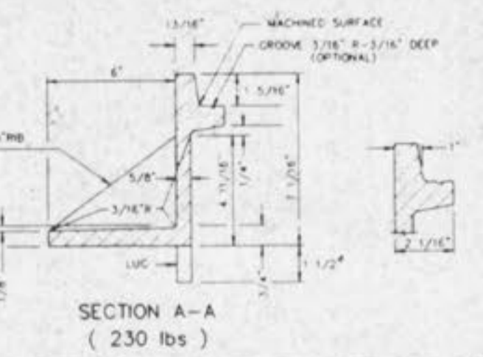
CAST IRON MANHOLE FRAME METROPOLITAN ST. LOUIS SEWER DISTRICT Standard Details of Sewer Construction Dr. D.A.B. Ch. J.C.K. 1992 SHEET 48
