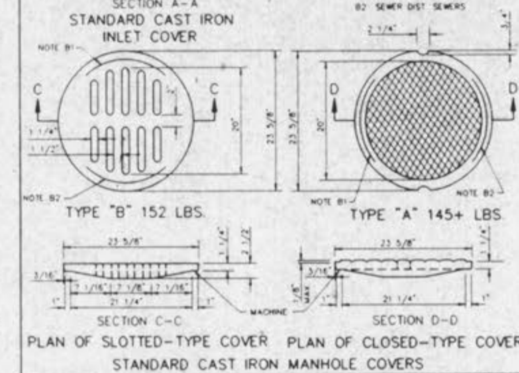
CAST IRON COVERS MANHOLES AND INLETS METROPOLITAN ST. LOUIS SEWER DISTRICT Standard Details of Sewer Construction Dr. R.G.W. Ch. J.C.K. 1992 SHEET 49
