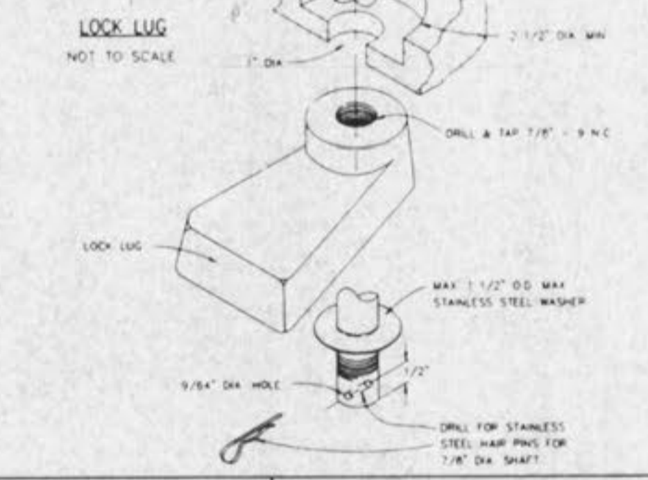
LOCKING DEVICE FOR TYPE "N" LOCK TYPE MANHOLE COVER METROPOLITAN ST. LOUIS SEWER DISTRICT Standard Details of Sewer Construction Dr. J.L.G. Ch. J.C.K. 1992 SHEET 52
