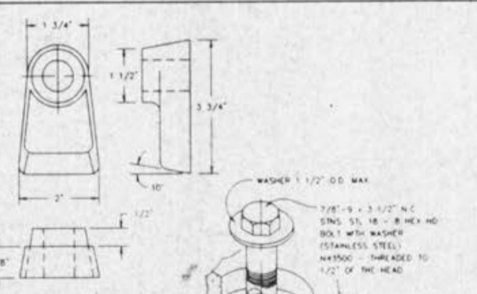
CAST IRON SIDE INTAKE UNIT FOR GRATED INLETS 249 LBS. METROPOLITAN ST. LOUIS SEWER DISTRICT Standard Details of Sewer Construction Dr. R.G.W. Ch. J.C.K. 1992 SHEET 47
