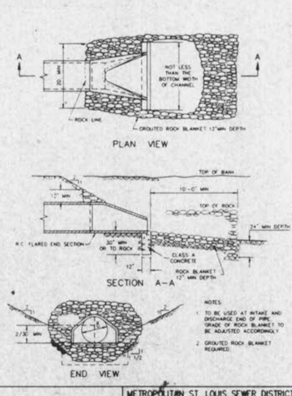
FLARED END SECTION METROPOLITAN ST. LOUIS SEWER DISTRICT Standard Details of Sewer Construction Dr. W.S.H. Ch. J.C.K. 1992 SHEET 57
