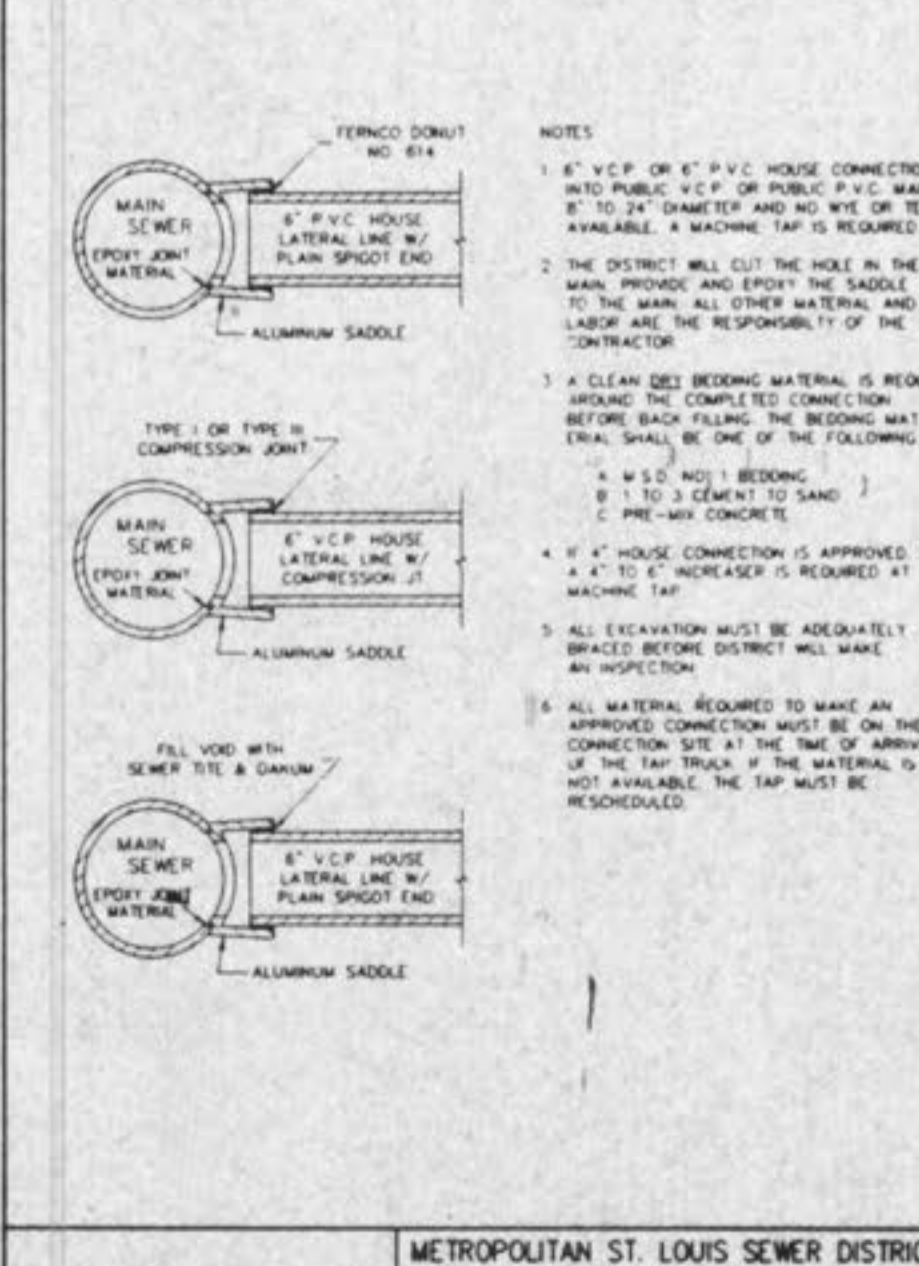
MACHINE TAP METROPOLITAN ST. LOUIS SEWER DISTRICT Standard Details of Sewer Construction Dr. W.S.H. Ch. J.C.K. 1992 SHEET 60
