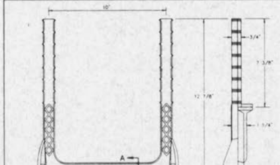
CAST IRON MANHOLE FRAME METROPOLITAN ST. LOUIS SEWER DISTRICT Standard Details of Sewer Construction Dr. D.A.B. Ch. J.C.K. 1992 SHEET 48
