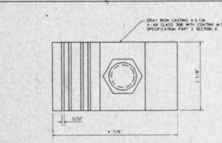
STEEL REQUIREMENTS FOR GRATE INLET SEAT METROPOLITAN ST. LOUIS SEWER DISTRICT Standard Details of Sewer Construction Dr. W.S.H. Ch. J.C.K. 1992 SHEET 46
