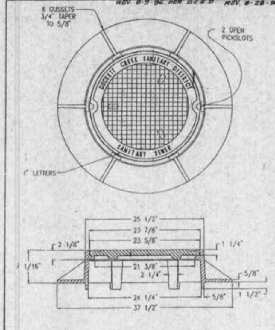
MANHOLE RING & COVER DUCKETT CREEK SANITARY DISTRICT STANDARD CONSTRUCTION DETAIL DETAIL NO. MAY 1996
