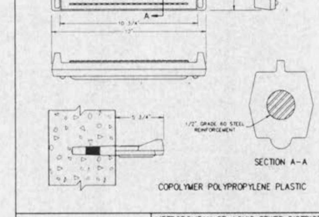
MANHOLE STEP FOR PRECAST MANHOLE METROPOLITAN ST. LOUIS SEWER DISTRICT Standard Details of Sewer Construction Dr. D.A.B. Ch. J.C.K. 1992 SHEET 54
