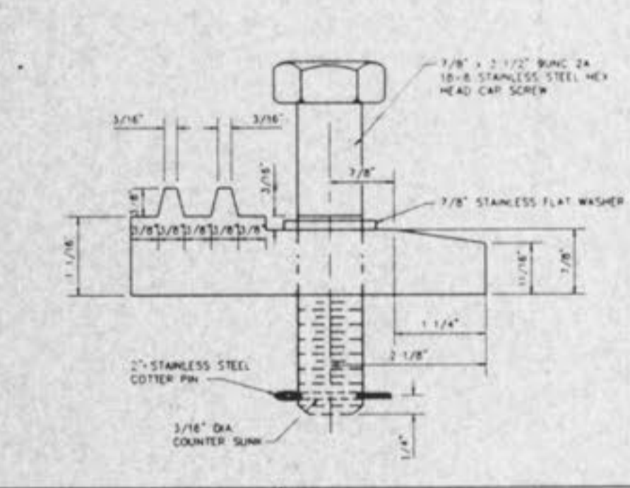
LOCKING DEVICE FOR TYPE "I" LOCK TYPE MANHOLE COVER METROPOLITAN ST. LOUIS SEWER DISTRICT Standard Details of Sewer Construction Dr. R.G.W. Ch. J.C.K. 1992 SHEET 51
