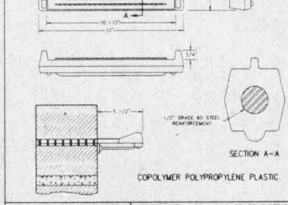
PSI-B MANHOLE STEP INTO JOINT METROPOLITAN ST. LOUIS SEWER DISTRICT Standard Details of Sewer Construction Dr. W.S.H. Ch. J.C.K. 1992 SHEET 53
