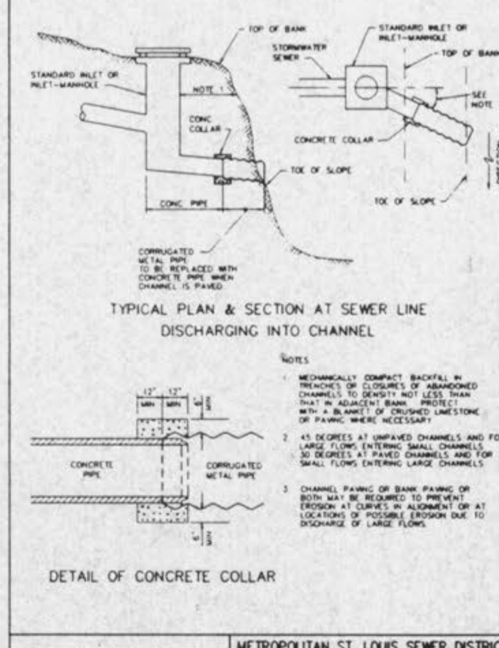
DETAIL OF CONCRETE COLLAR METROPOLITAN ST. LOUIS SEWER DISTRICT Standard Details of Sewer Construction Dr. R.G.W. Ch. J.C.K. 1992 SHEET 58
