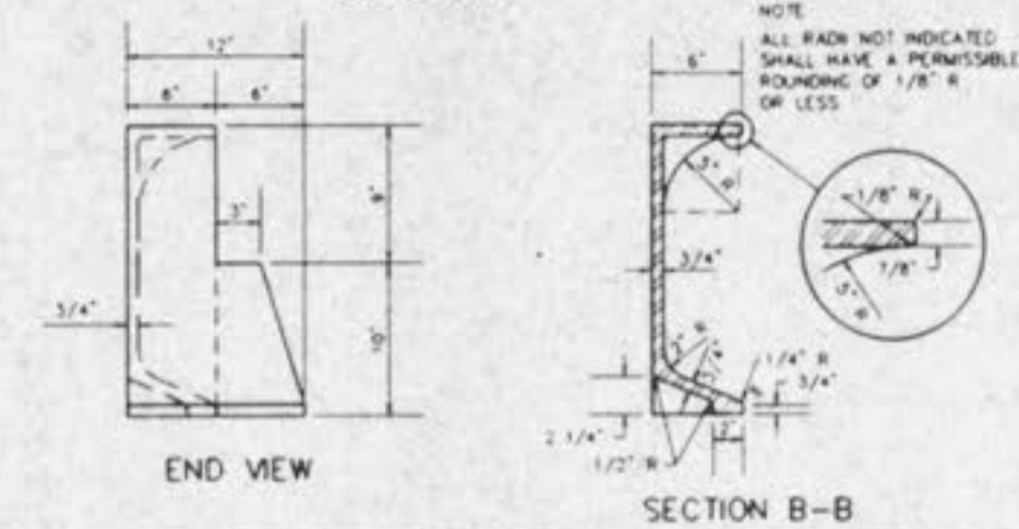
CAST IRON SIDE INTAKE UNIT FOR GRATED INLETS 249 LBS. METROPOLITAN ST. LOUIS SEWER DISTRICT Standard Details of Sewer Construction Dr. R.G.W. Ch. J.C.K. 1992 SHEET 47
