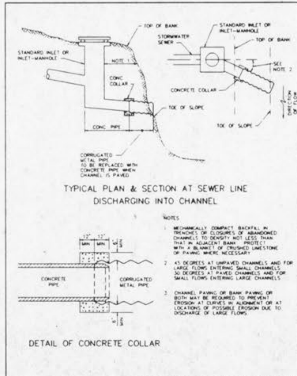
TYPICAL PLAN & SECTION AT SEWER LINE DISCHARGING INTO CHANNEL METROPOLITAN ST. LOUIS SEWER DISTRICT Standard Details of Sewer Construction Dr. R.G.W. 1992 SHEET 58
