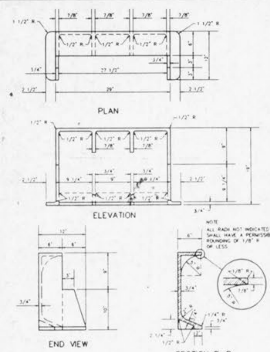
CAST IRON SIDE INTAKE UNIT FOR GRATED INLETS 249 LBS. METROPOLITAN ST. LOUIS SEWER DISTRICT Standard Details of Sewer Construction Dr. R.G.W. 1992 SHEET 47
