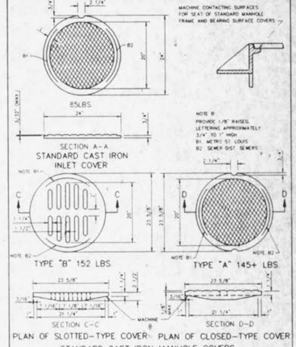
CAST IRON COVERS MANHOLES AND INLETS METROPOLITAN ST. LOUIS SEWER DISTRICT Standard Details of Sewer Construction Dr. R.G.W. 1992 SHEET 49
