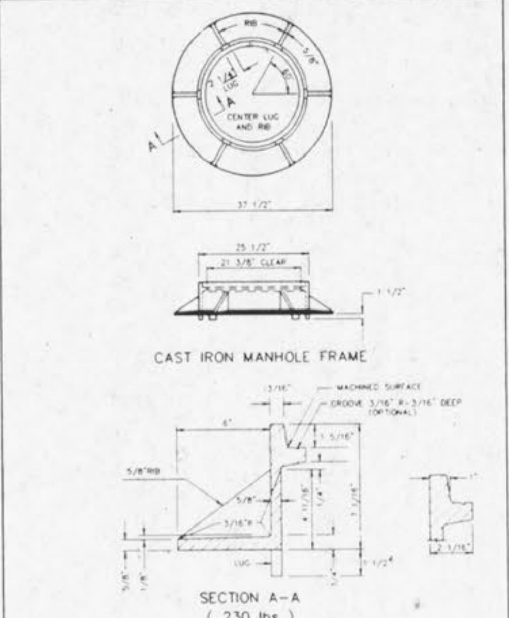
CAST IRON MANHOLE FRAME METROPOLITAN ST. LOUIS SEWER DISTRICT Standard Details of Sewer Construction Dr. D.A.B. 1992 SHEET 48
