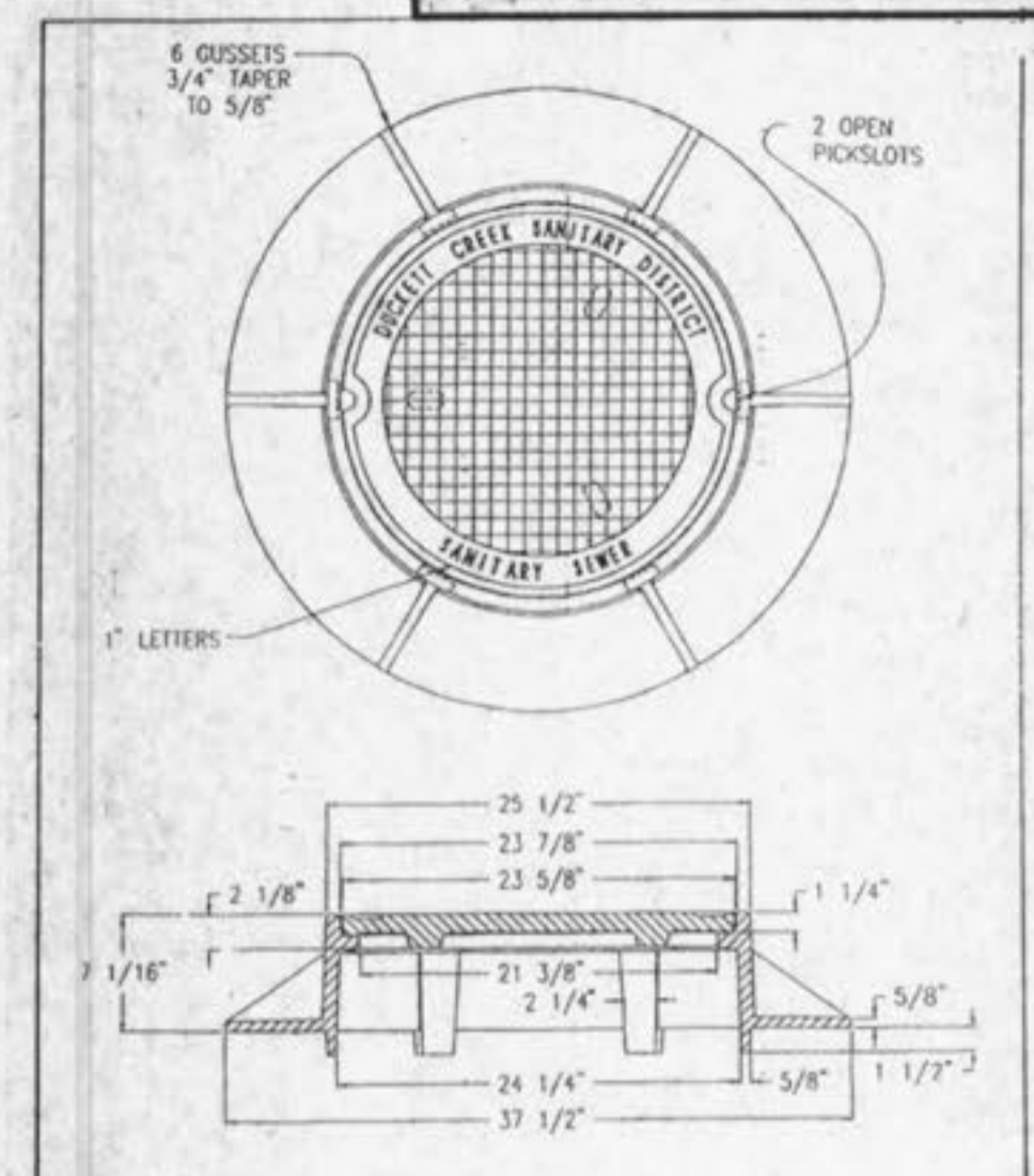
MANHOLE RING & COVER DUCKETT CREEK SANITARY DISTRICT STANDARD CONSTRUCTION DETAIL DETAIL NO. MAY 1996
