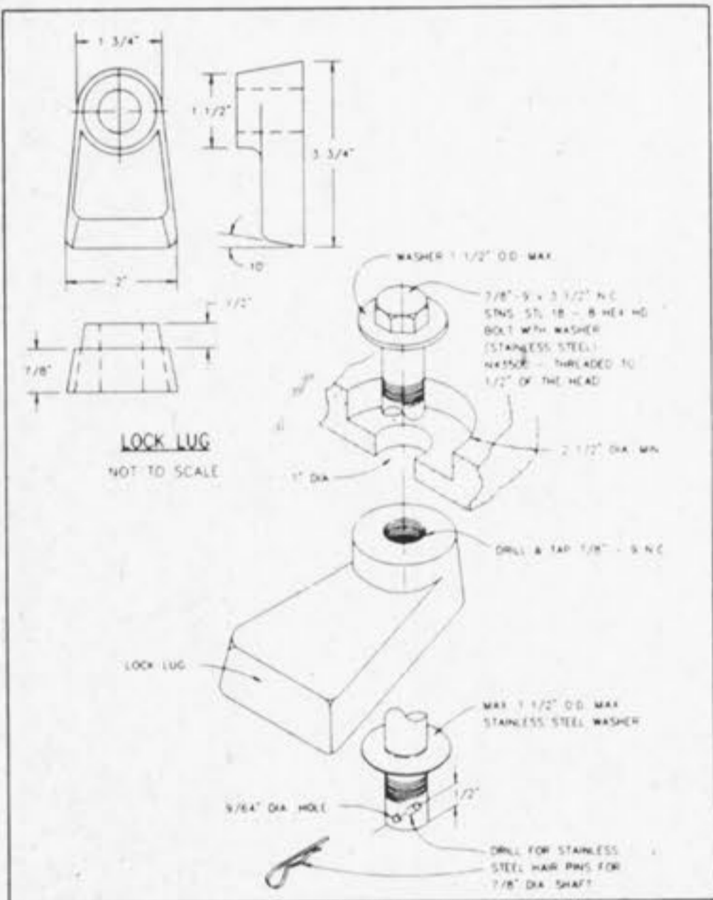
LOCK LUG FOR TYPE 'T' LOCK TYPE MANHOLE COVER METROPOLITAN ST. LOUIS SEWER DISTRICT Standard Details of Sewer Construction Dr. J.L.G. 1992 SHEET 52
