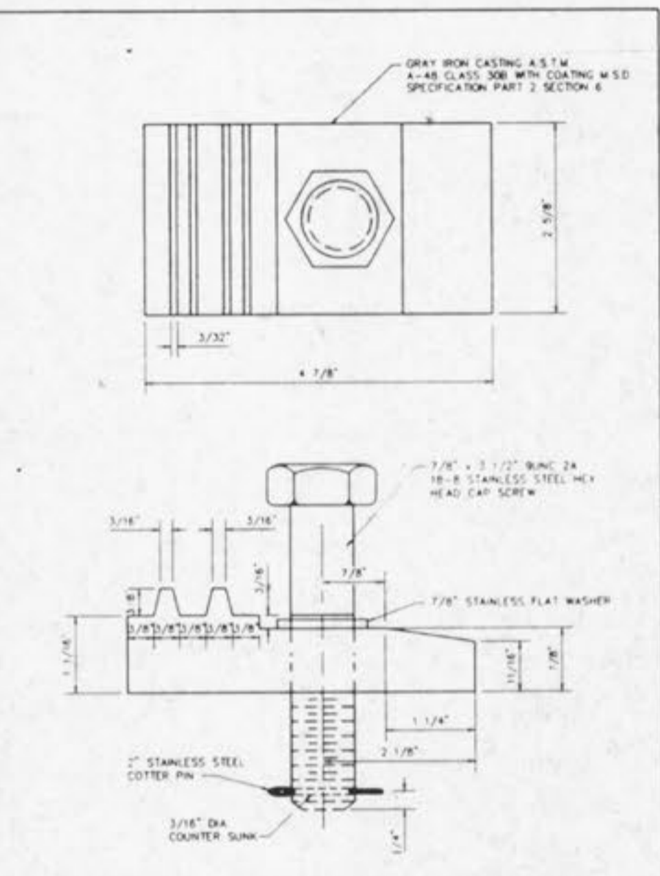
LOCKING DEVICE FOR TYPE 'T' LOCK TYPE MANHOLE COVER METROPOLITAN ST. LOUIS SEWER DISTRICT Standard Details of Sewer Construction Dr. R.G.W. 1992 SHEET 51
