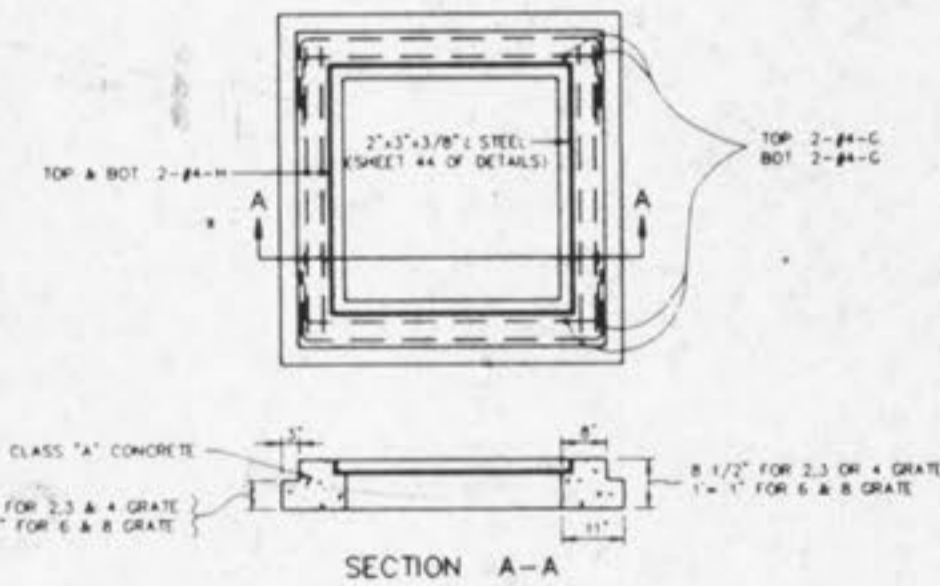
STEEL REQUIREMENTS FOR GRATE INLET SEAT METROPOLITAN ST. LOUIS SEWER DISTRICT Standard Details of Sewer Construction Dr. W.S.H. 1992 SHEET 46
