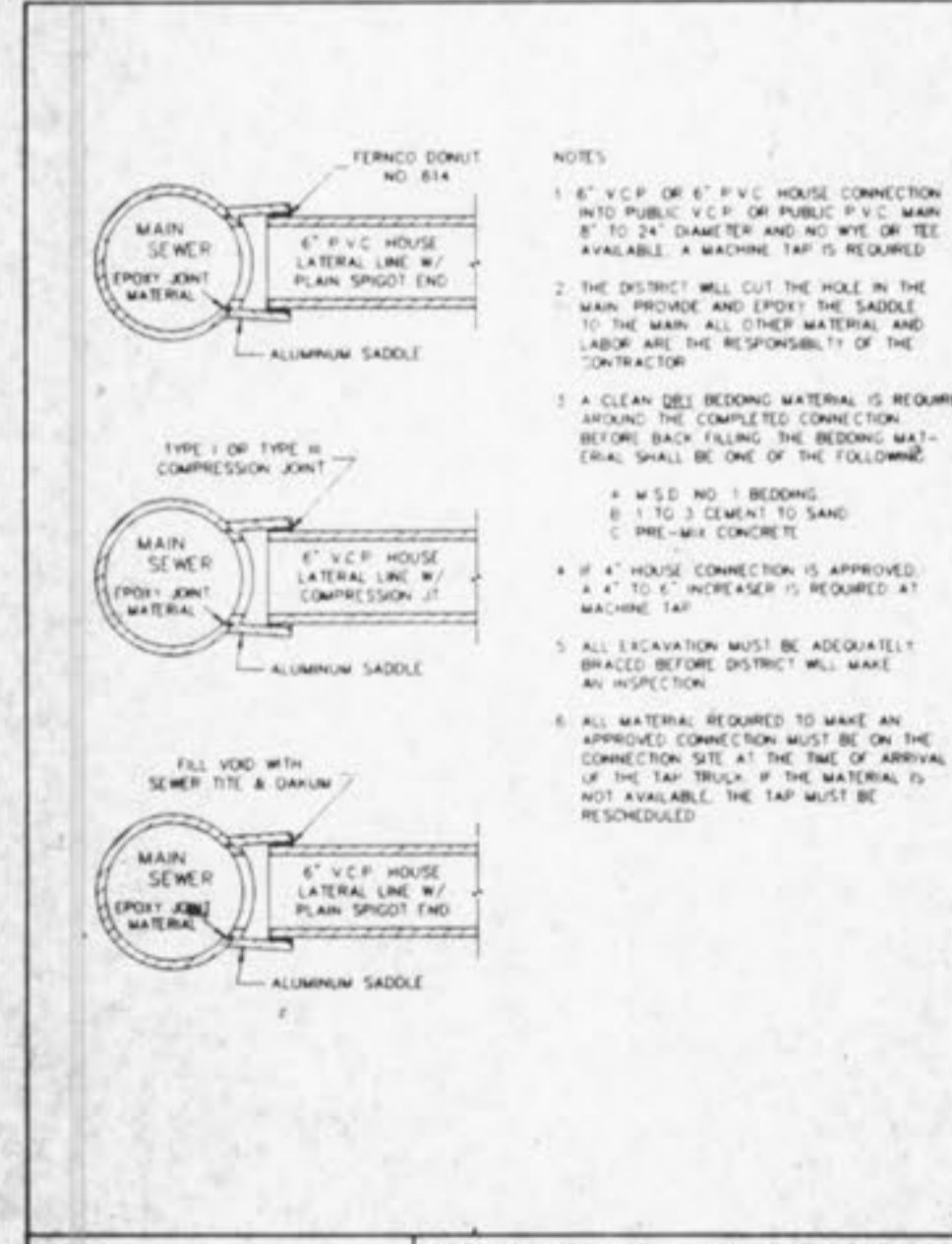
MACHINE TAP METROPOLITAN ST. LOUIS SEWER DISTRICT Standard Details of Sewer Construction Dr. W.S.H. 1992 SHEET 60
