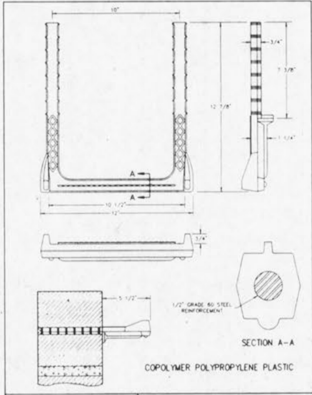
PSI-B MANHOLE STEP INTO JOINT METROPOLITAN ST. LOUIS SEWER DISTRICT Standard Details of Sewer Construction Dr. W.S.H. 1992 SHEET 53
