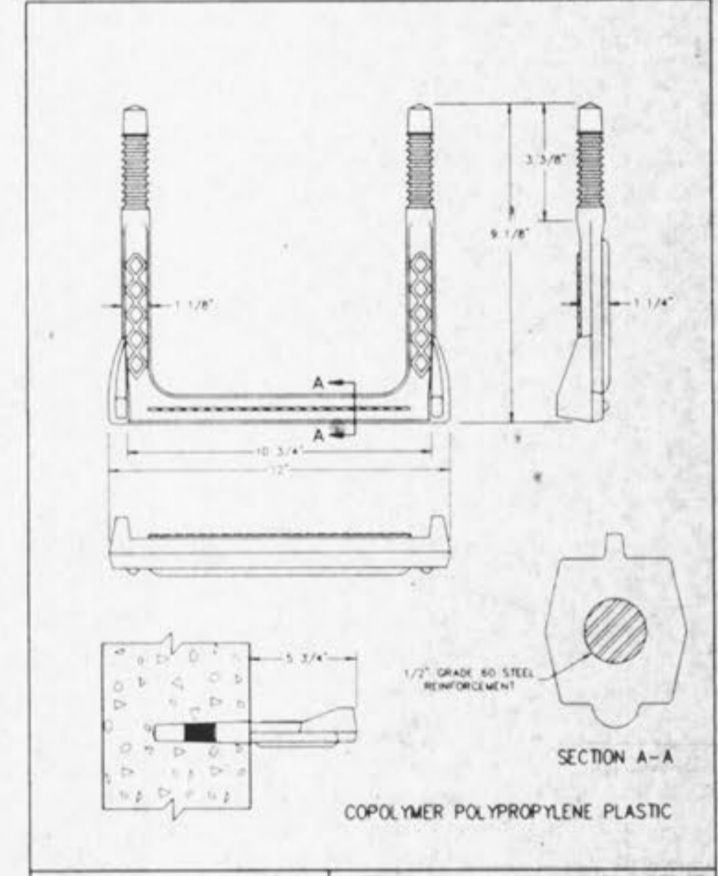
MANHOLE STEP FOR PRECAST MANHOLE METROPOLITAN ST. LOUIS SEWER DISTRICT Standard Details of Sewer Construction Dr. D.A.B. 1992 SHEET 54
