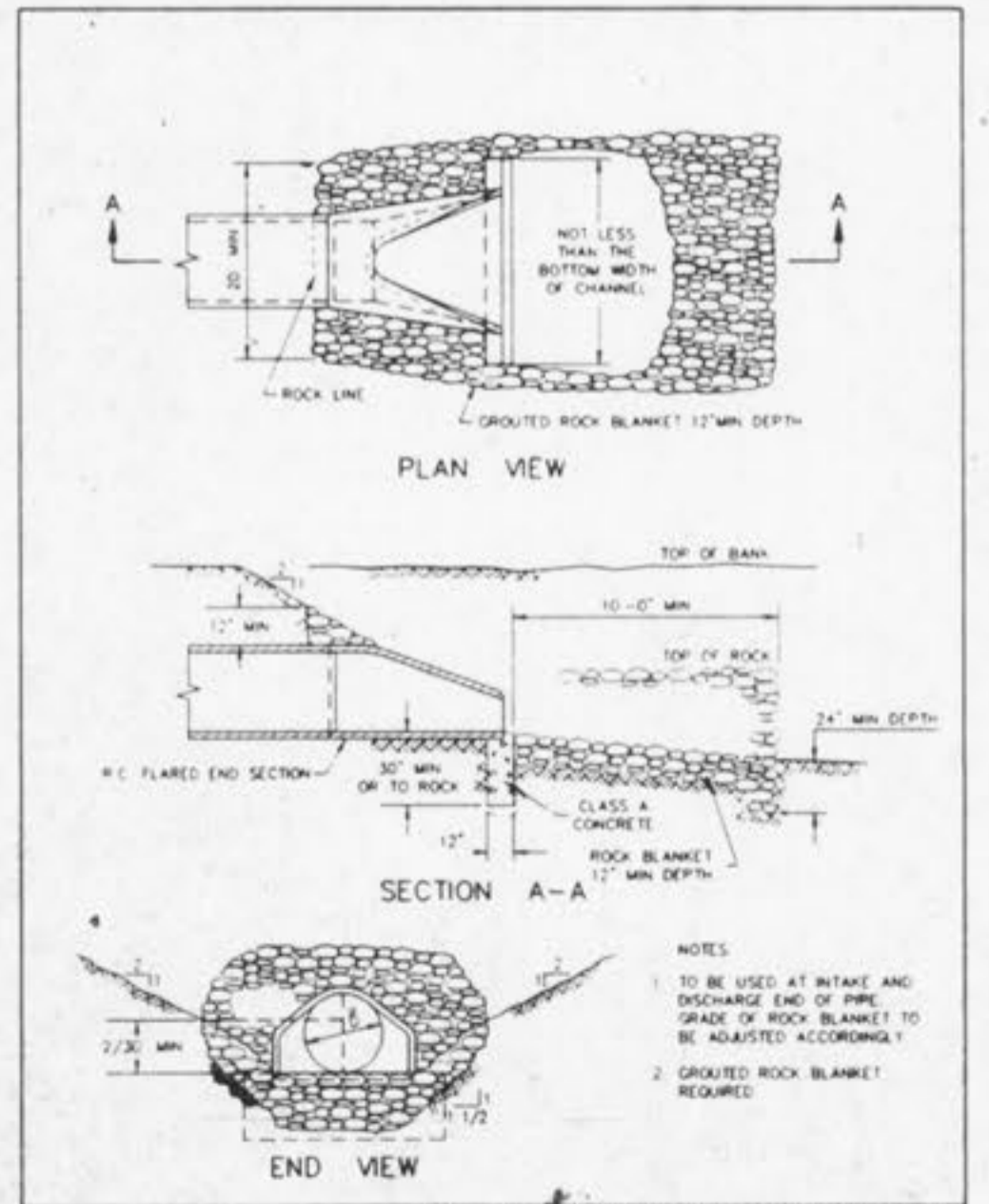
FLARED END SECTION METROPOLITAN ST. LOUIS SEWER DISTRICT Standard Details of Sewer Construction Dr. W.S.H. 1992 SHEET 57
