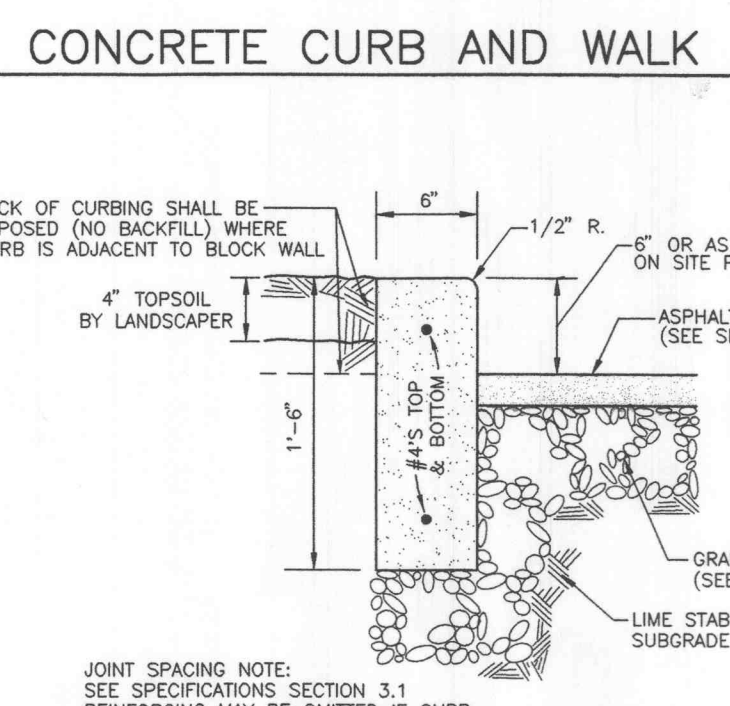
CONCRETE CURB AND GUTTER WITH WALK (OPTIONAL CONSTRUCTION)
