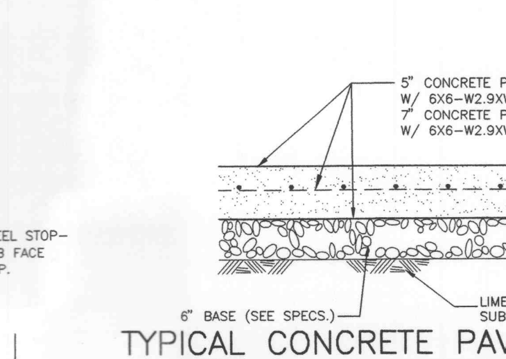
TYPICAL CONCRETE PAVING SECTION
