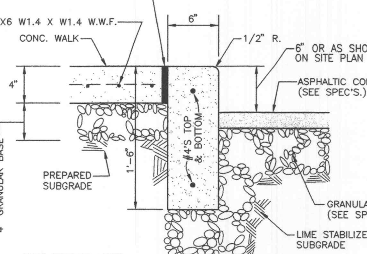
CONCRETE CURB AND WALK
