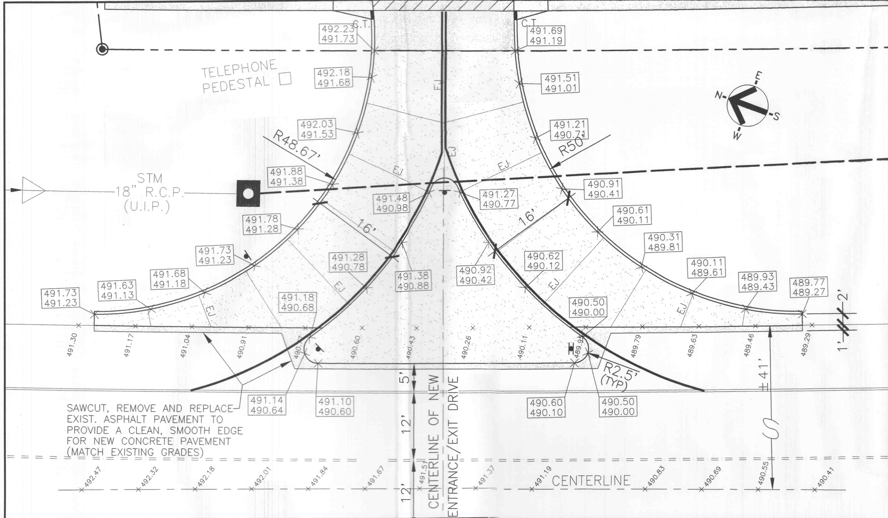
NEW CONCRETE DRIVE APRON GRADES AND JOINT LOCATIONS (MISSOURI STATE HIGHWAY 'K')
