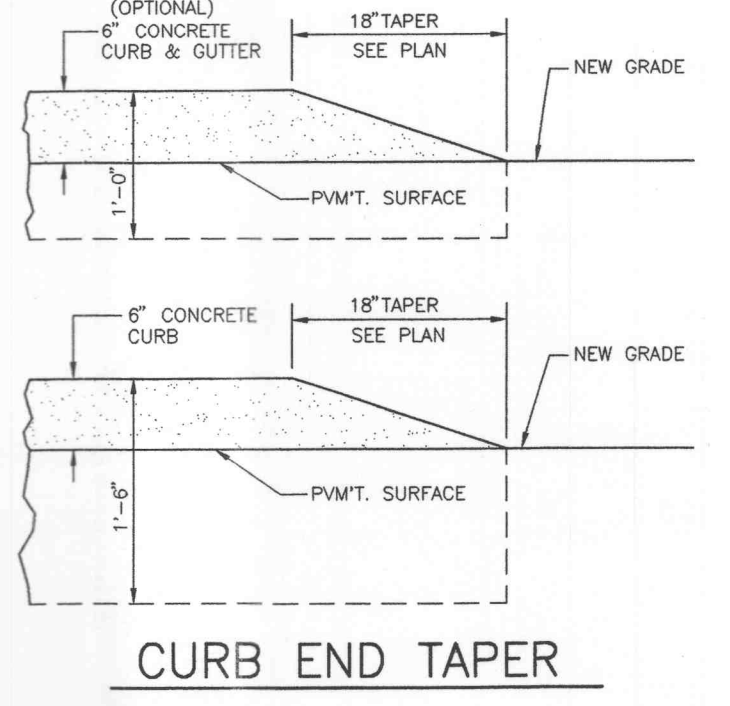
CURB END TAPER
