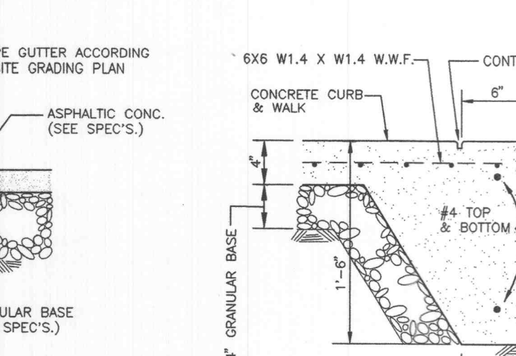
CONCRETE CURB AND GUTTER WITH WALK (OPTIONAL CONSTRUCTION)
