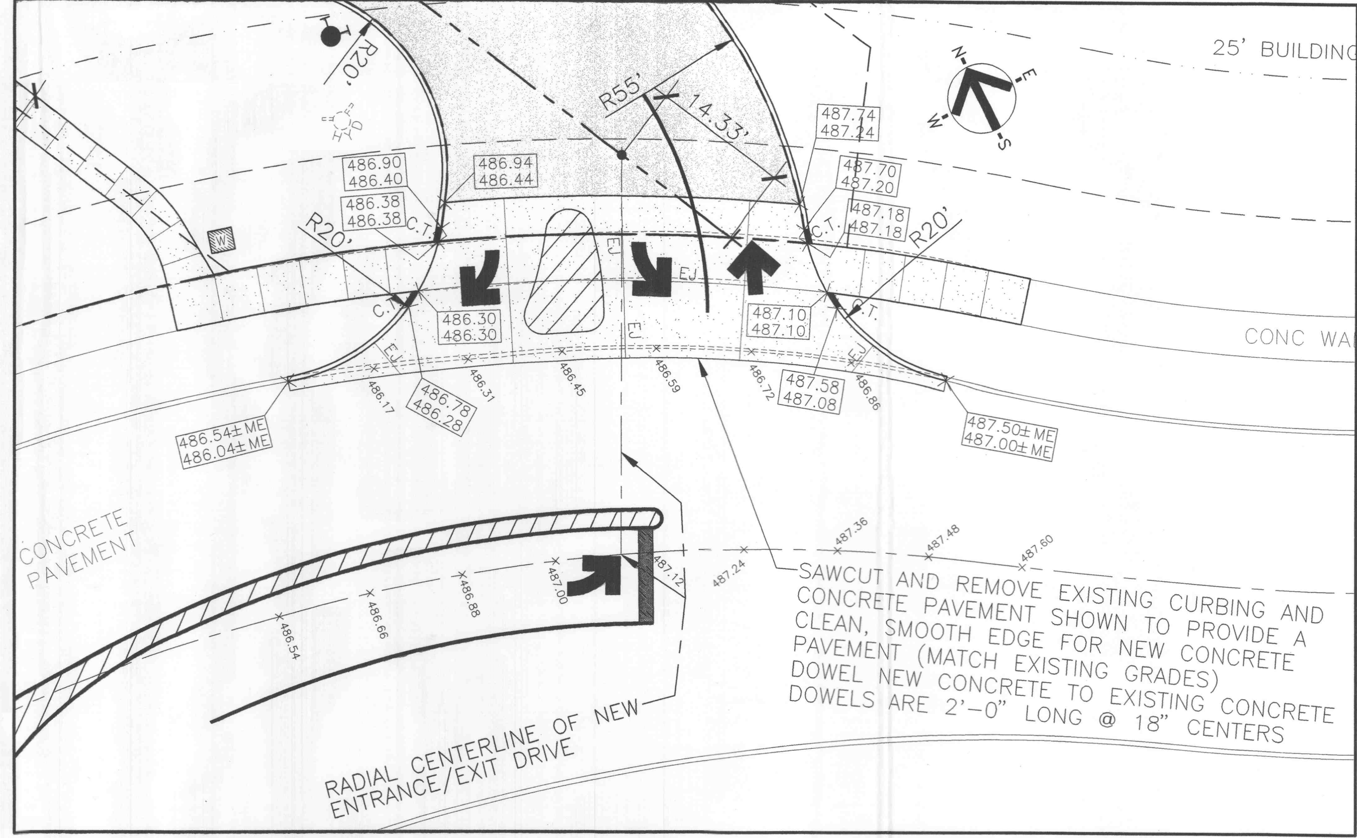
NEW CONCRETE DRIVE APRON GRADES AND JOINT LOCATIONS (PHEASANT MEADOW DRIVE)
