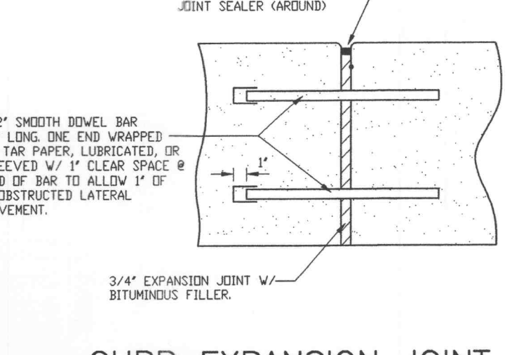
CURB EXPANSION JOINT
