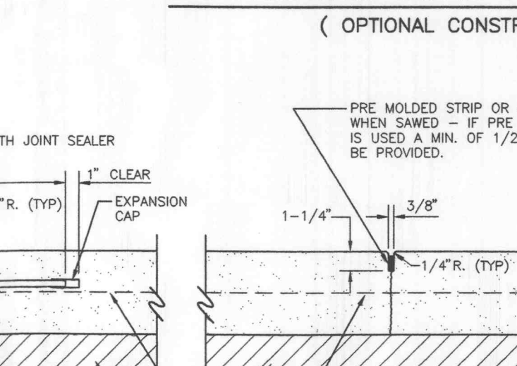
TYPICAL PAVEMENT AND JOINT DETAIL
