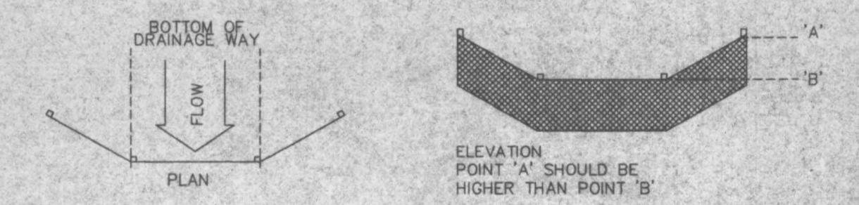
SILTATION FENCE DETAIL NOT TO SCALE
