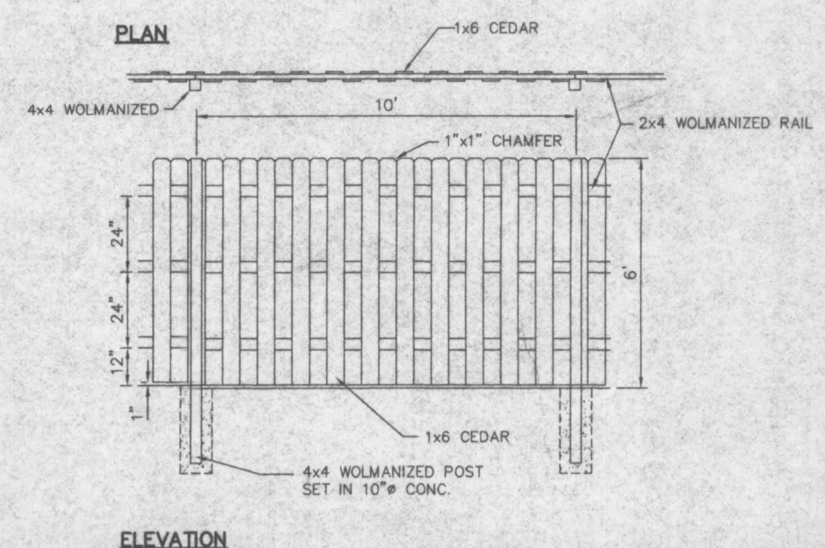
SCREEN FENCE DETAIL NOT TO SCALE
