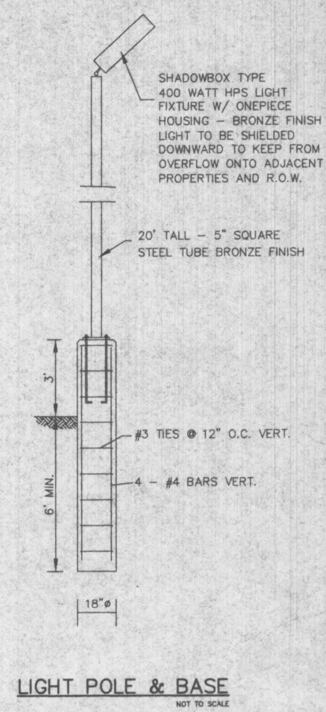
LIGHT POLE & BASE NOT TO SCALE
