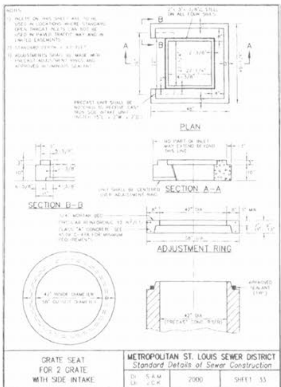
GRATE SEAT FOR 2 GRATES WITH SIDE INTAKE METROPOLITAN ST. LOUIS SEWER DISTRICT Standard Details of Sewer Construction SHEET 33
