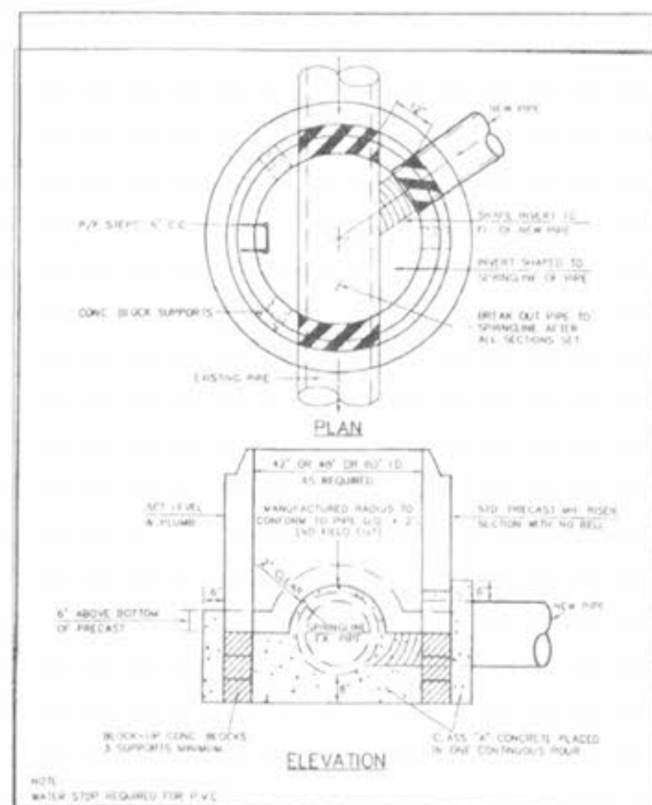
PRECAST MANHOLE ON EXIST. PIPE W/CONTINUOUS FLOW ONLY METROPOLITAN ST. LOUIS SEWER DISTRICT Standard Details of Sewer Construction SHEET 22
