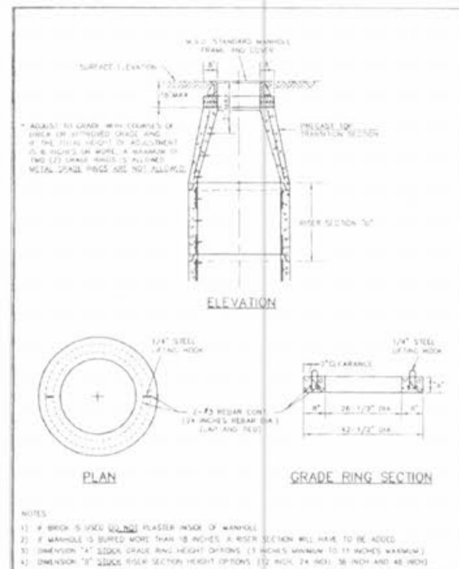
ADJUST TO GRADE METROPOLITAN ST. LOUIS SEWER DISTRICT Standard Details of Sewer Construction SHEET 23
