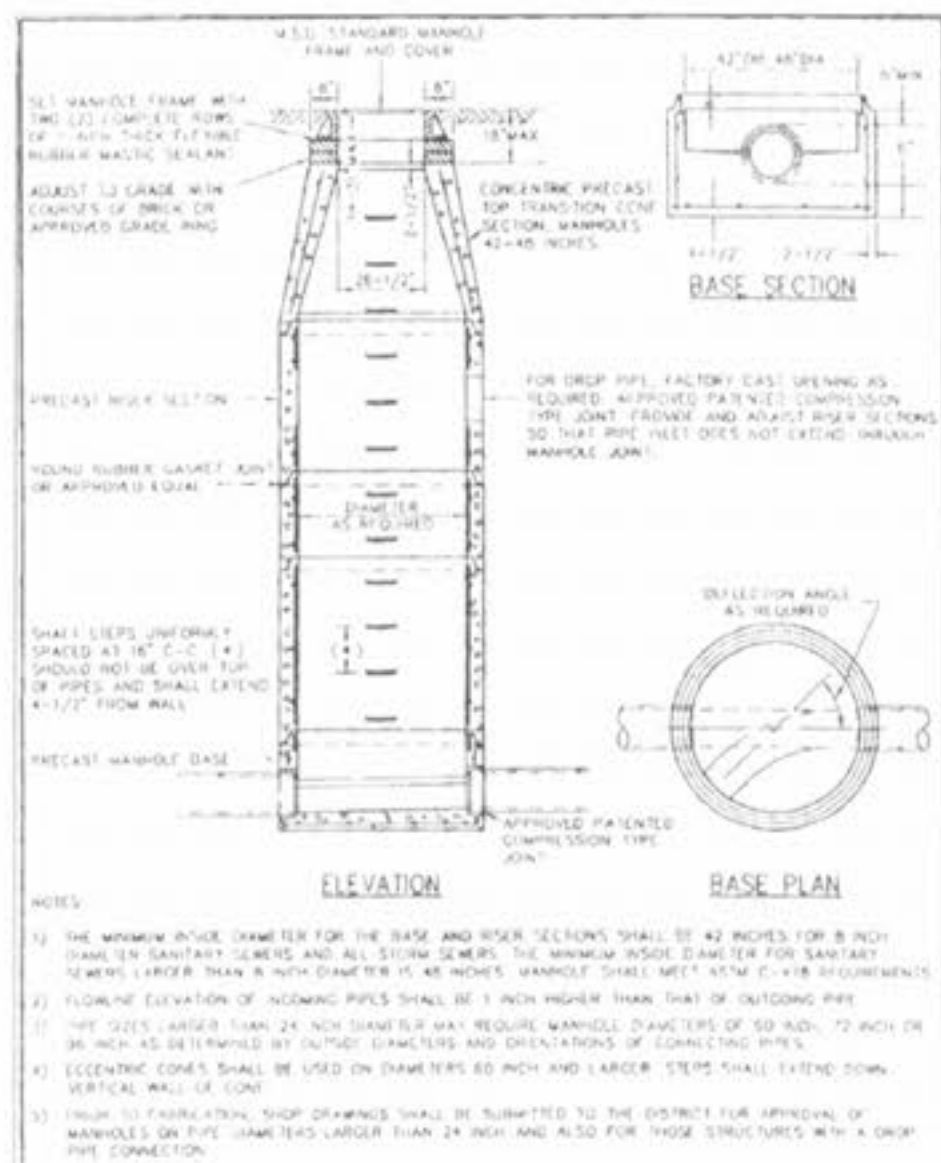
PRECAST CONCRETE MANHOLE METROPOLITAN ST. LOUIS SEWER DISTRICT Standard Details of Sewer Construction SHEET 21
