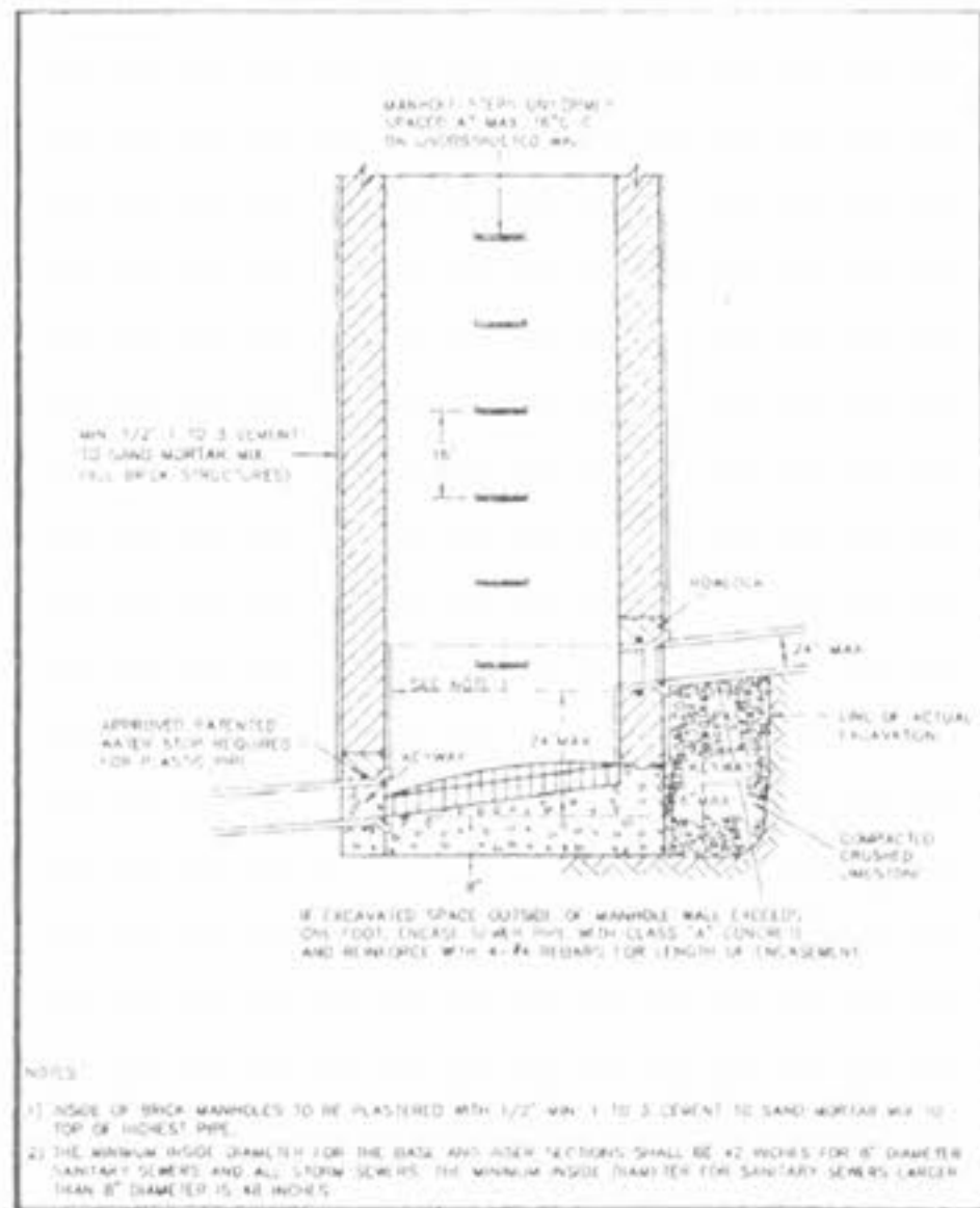
INSIDE FOULWATER DROP MANHOLE (FOR FREE-FALL) METROPOLITAN ST. LOUIS SEWER DISTRICT Standard Details of Sewer Construction SHEET 19
