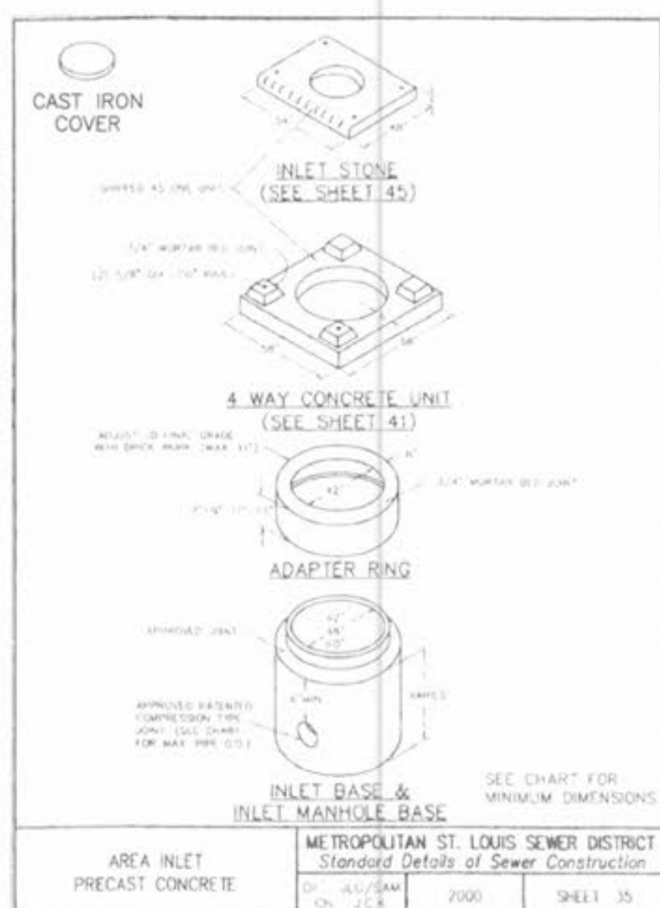
AREA INLET PRECAST CONCRETE METROPOLITAN ST. LOUIS SEWER DISTRICT Standard Details of Sewer Construction SHEET 35
