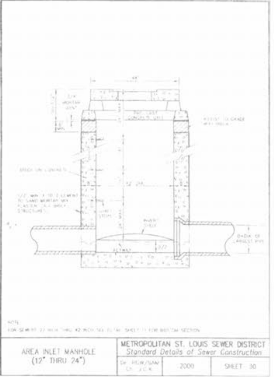
AREA INLET MANHOLE (12\"/>
