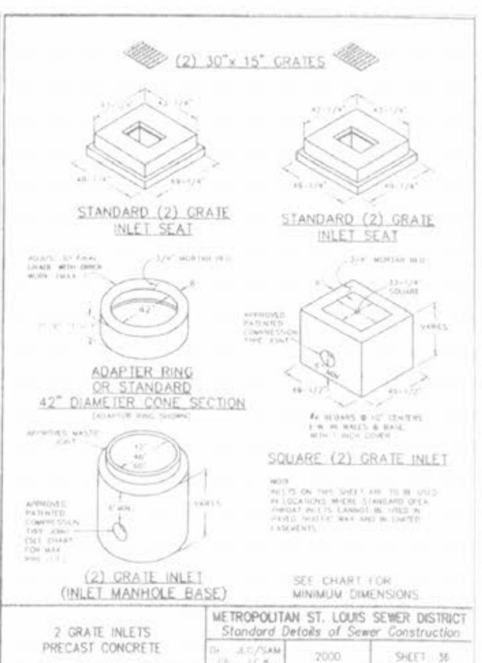
2 GRATE INLETS PRECAST CONCRETE METROPOLITAN ST. LOUIS SEWER DISTRICT Standard Details of Sewer Construction SHEET 36
