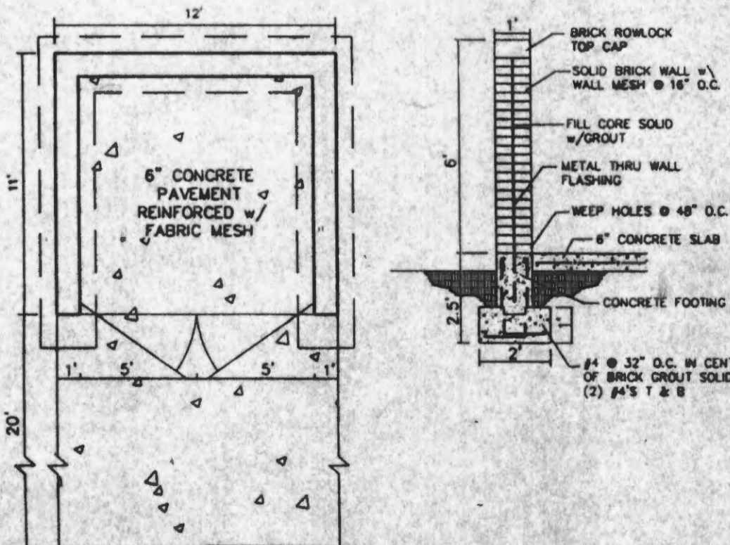
CONCRETE TRASH ENCLOSURE DETAIL
