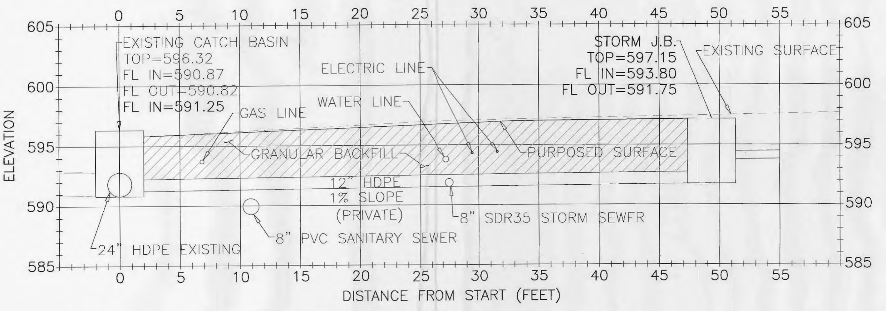
STORM SEWER PROFILE SCALE 1"=5' (PRIVATE)
